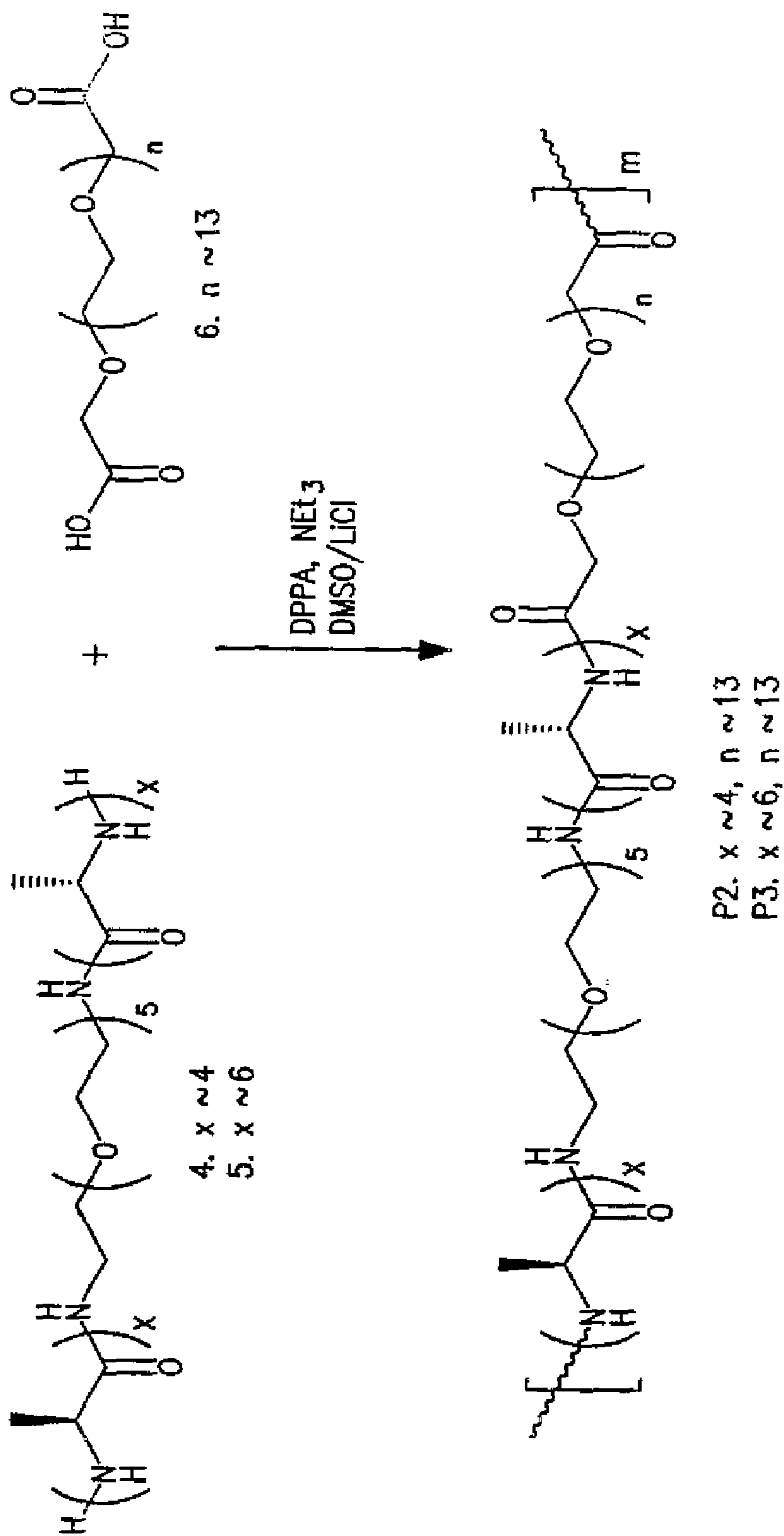
Scheme 2
