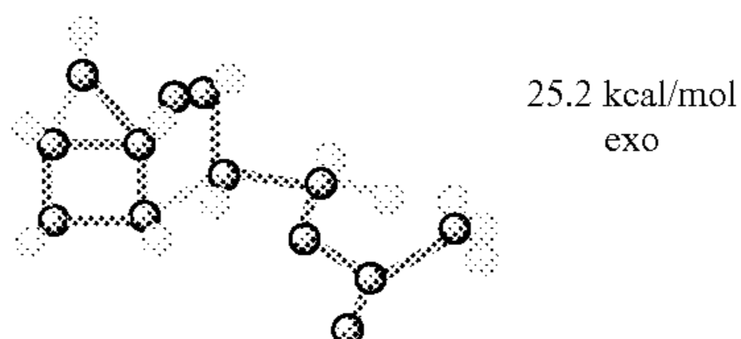
[Reaction scheme 1]
