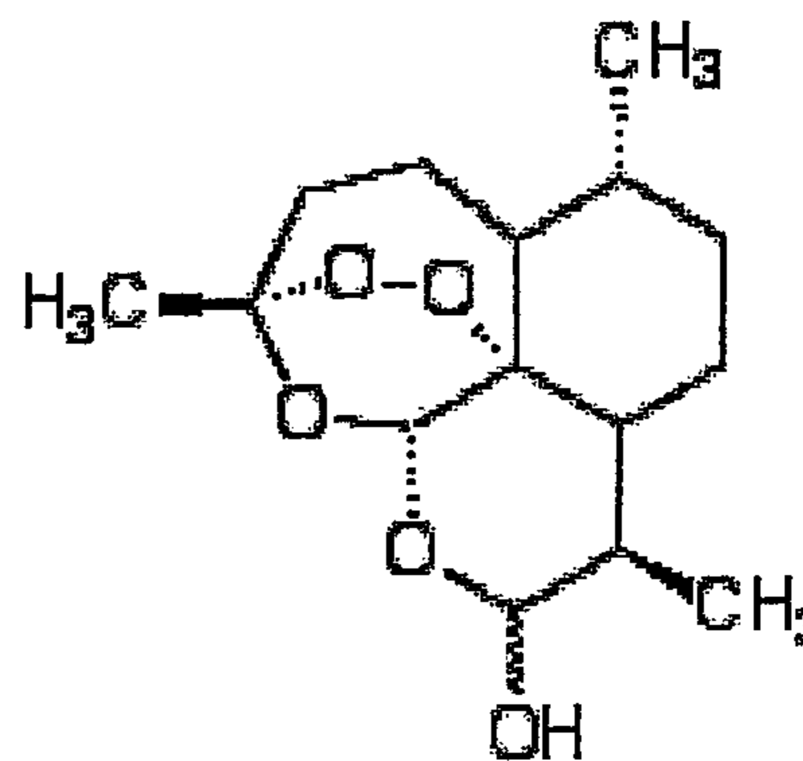
Dihydroartemisinin
