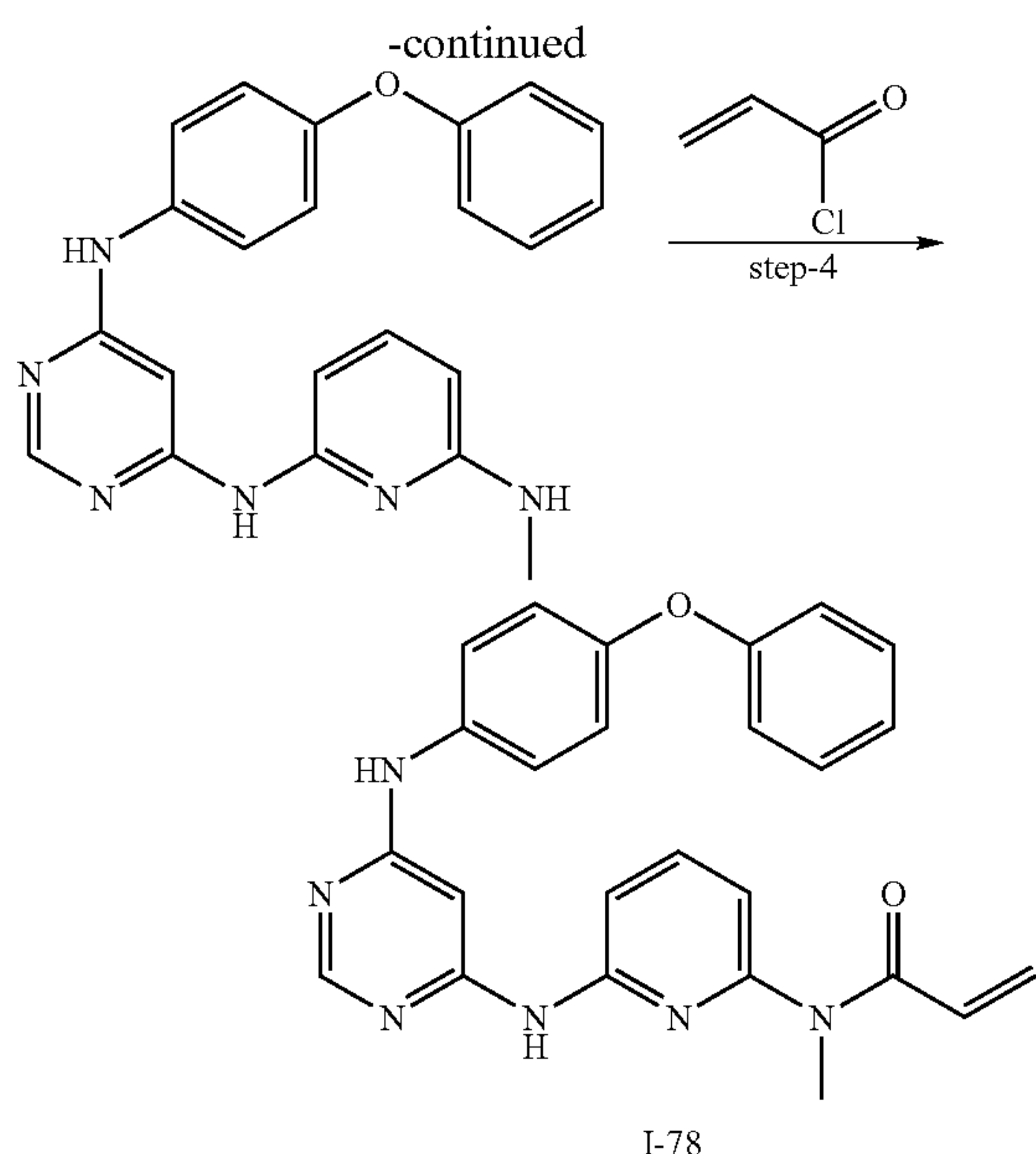
Synthesis of N-methyl-N-(6-(6-(4-phenoxyphenylamino)pyrimidin-4-ylamino)pyridine-2-yl)acrylamide (I-78)
