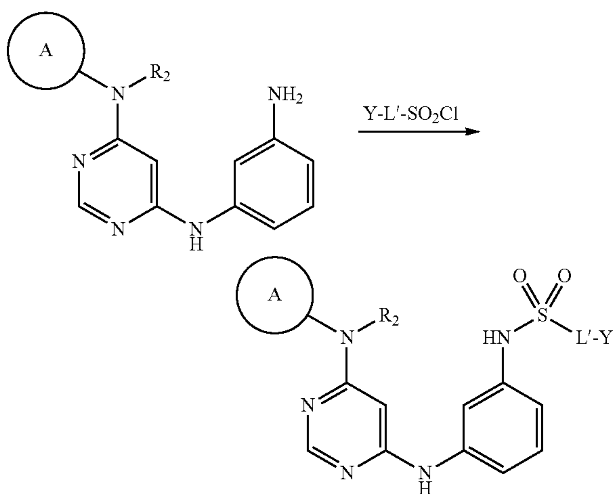
SCHEME 5a Synthesis of N-{3-[6-(arylamino)-pyrimidin-4-ylamino]-phenyl}-ethanesulfonamides
