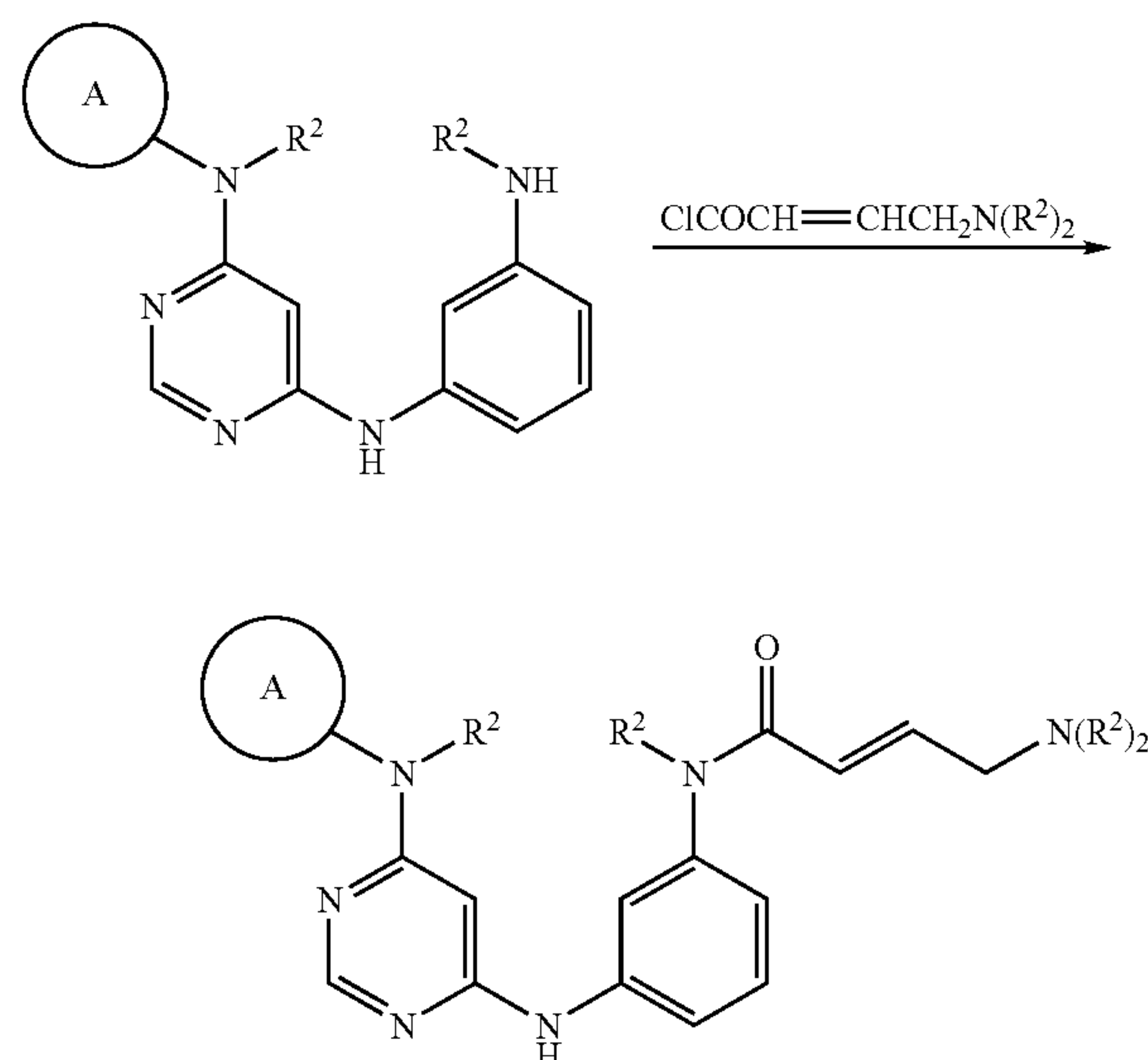
SCHEME 4a Sequence A for Synthesis of N-3-(6-mono or disubstituted-aminopyrimidin-4-yl)amino-N-mono- or unsubstituted-phenyl-4-amino-substituted-2-butenamides
