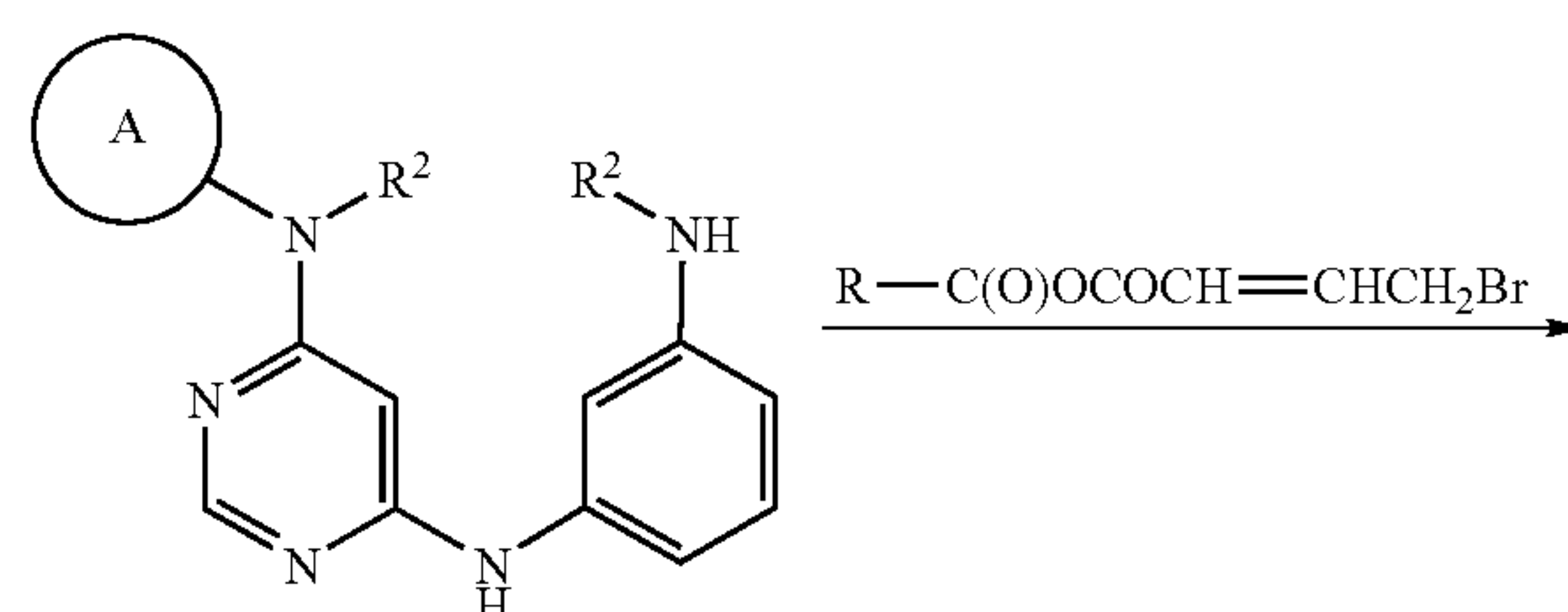
SCHEME 4b Sequence B for Synthesis of N-3-(6-mono or disubstituted-aminopyrimidin-4-yl)amino-N-mono- or unsubstituted-phenyl-4-amino-substituted-2-butenamides
