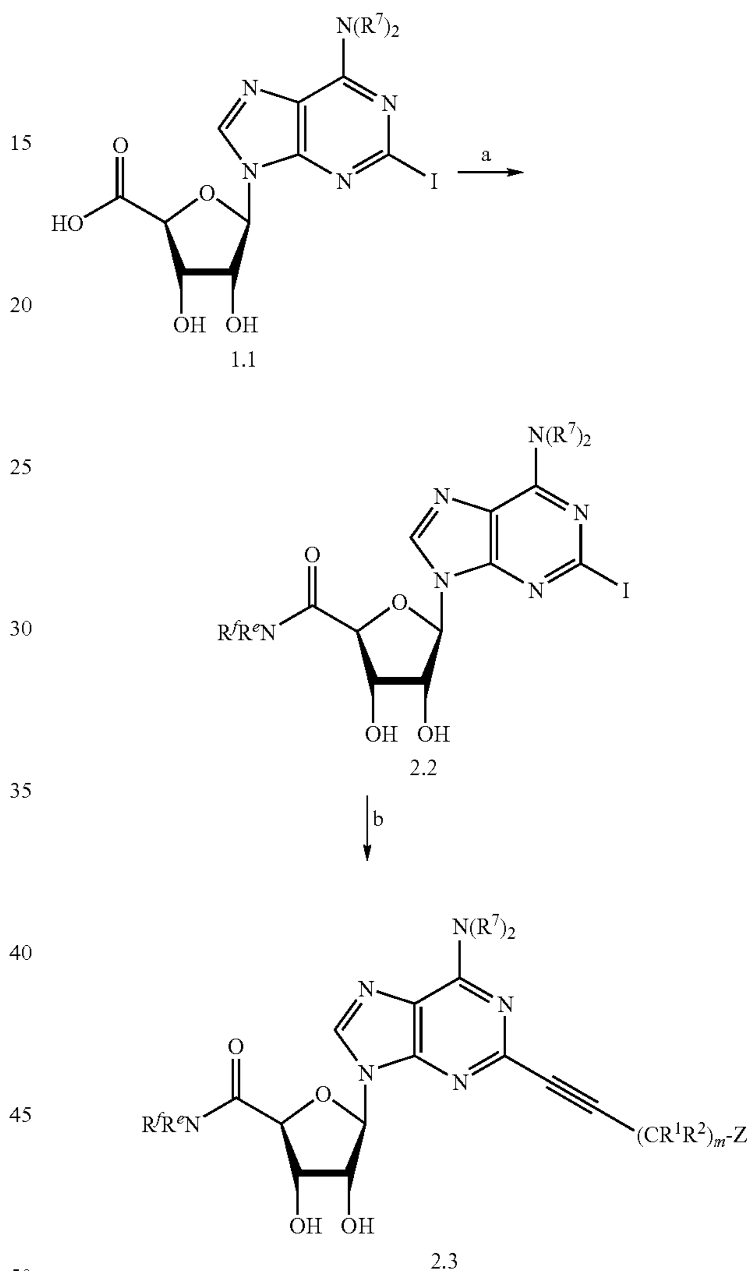
Scheme 2: Preparation of 5' amide analogs:
