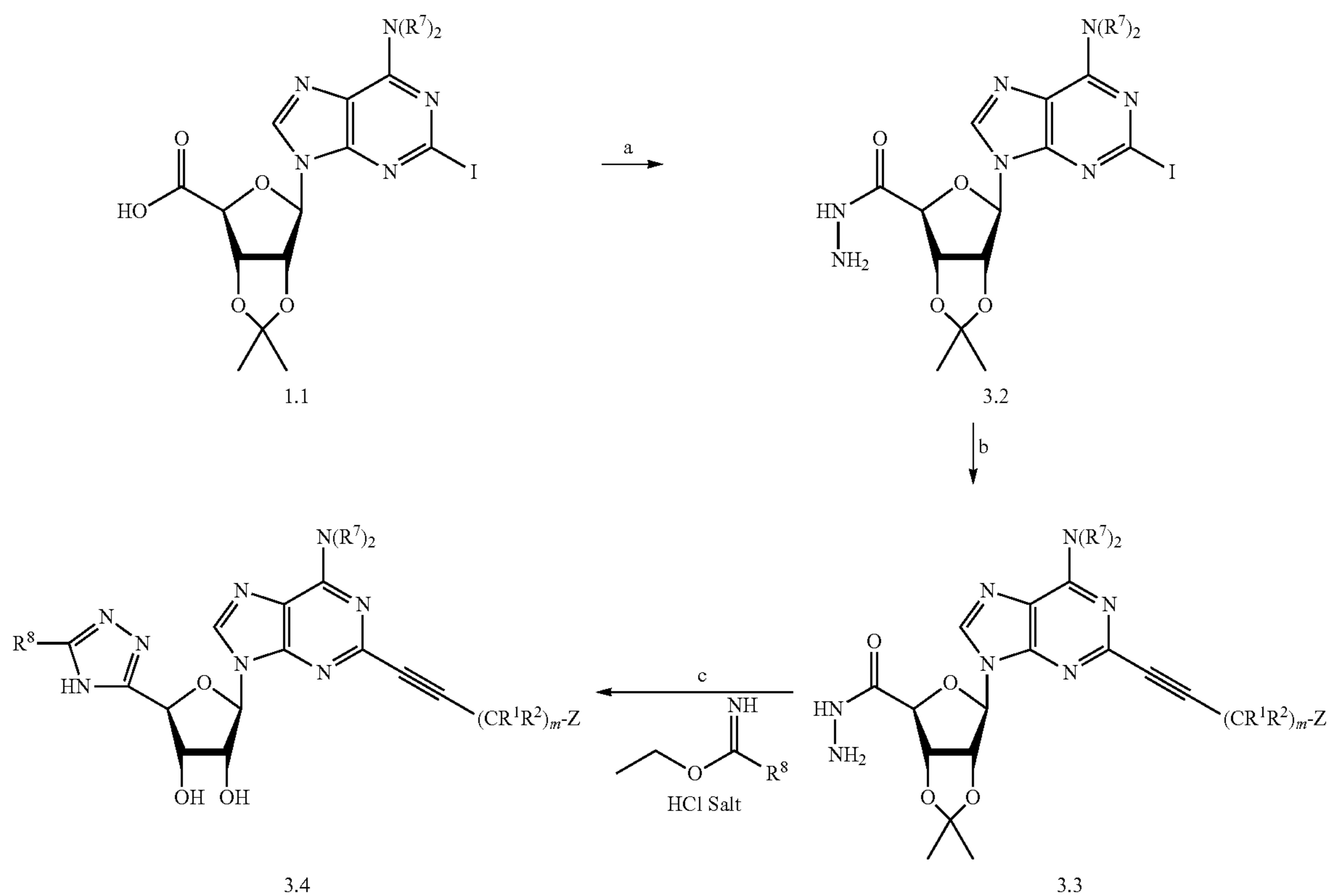
Scheme 3: Preparation of 4' triazoles:
