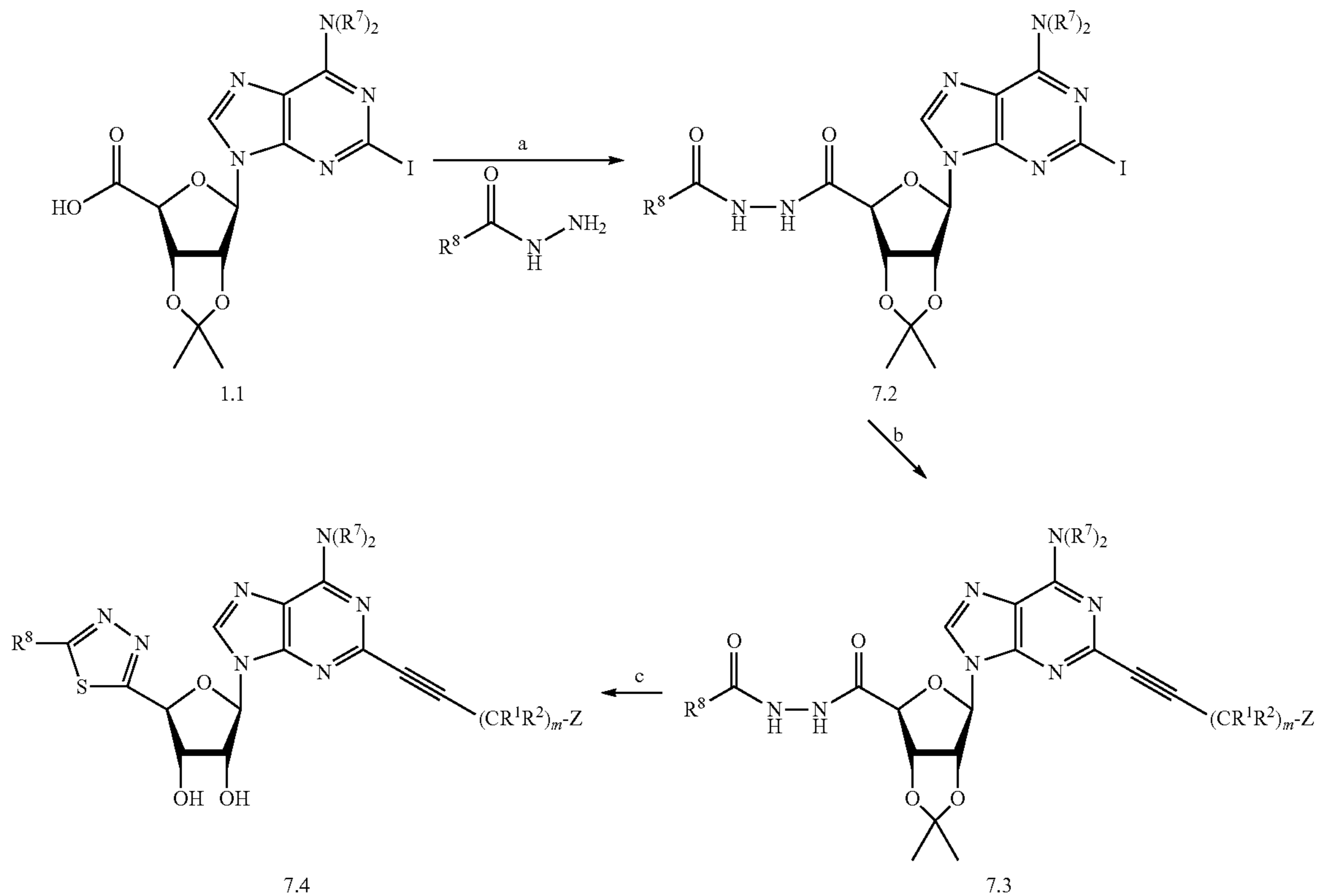
Scheme 7: Preparation of 4'-1,3,4 thiadiazole
