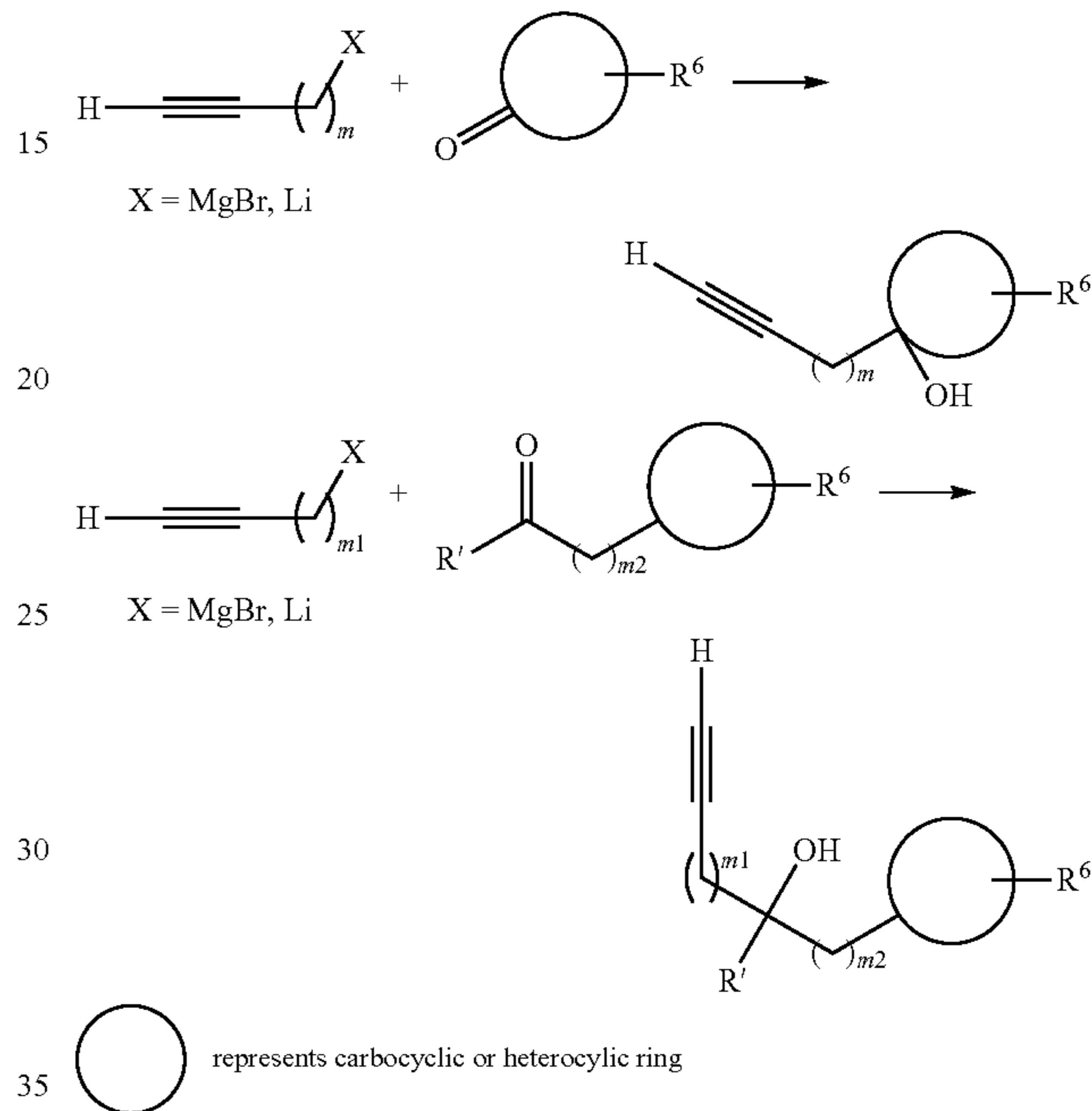
Scheme 1A General Route to Synthesis of Alkyne Precursors
