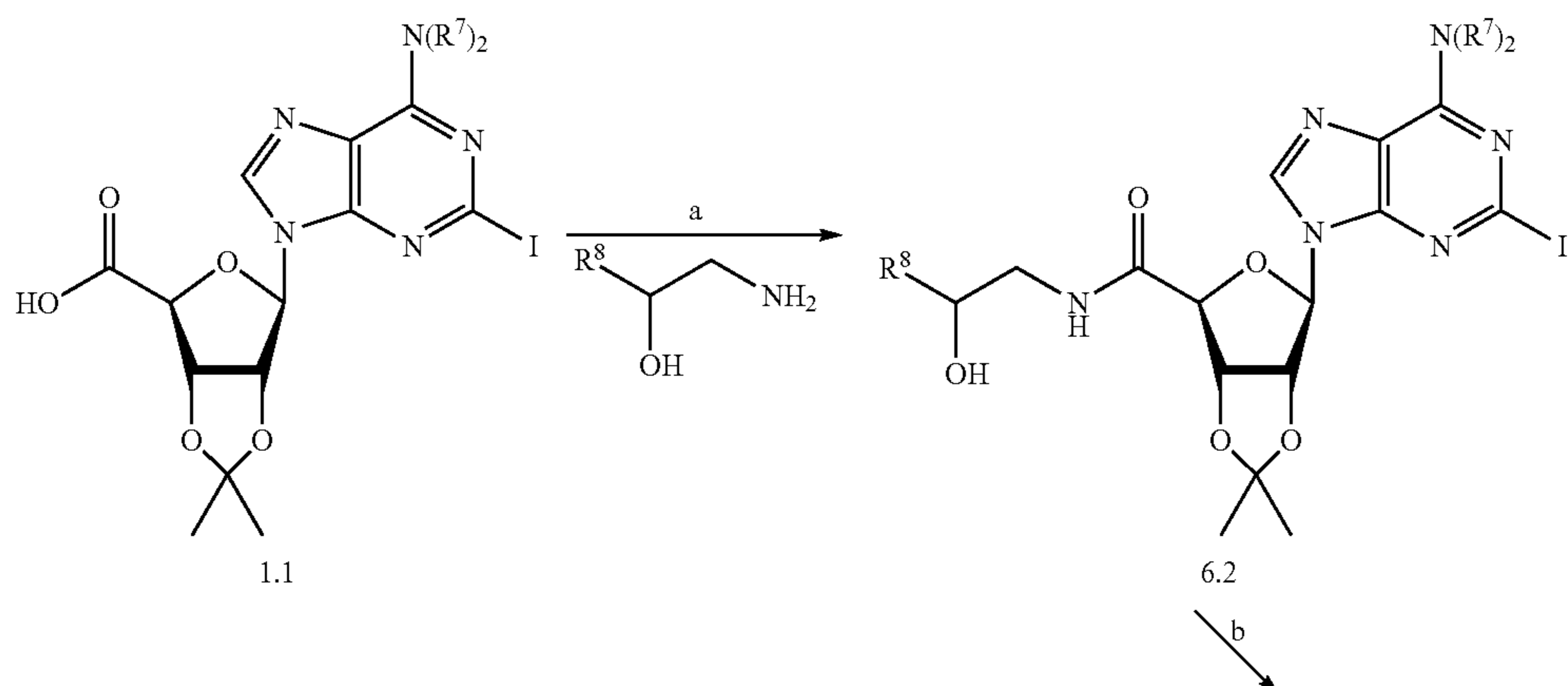
Scheme 6: Preparation of 4'-1,3 oxazole
