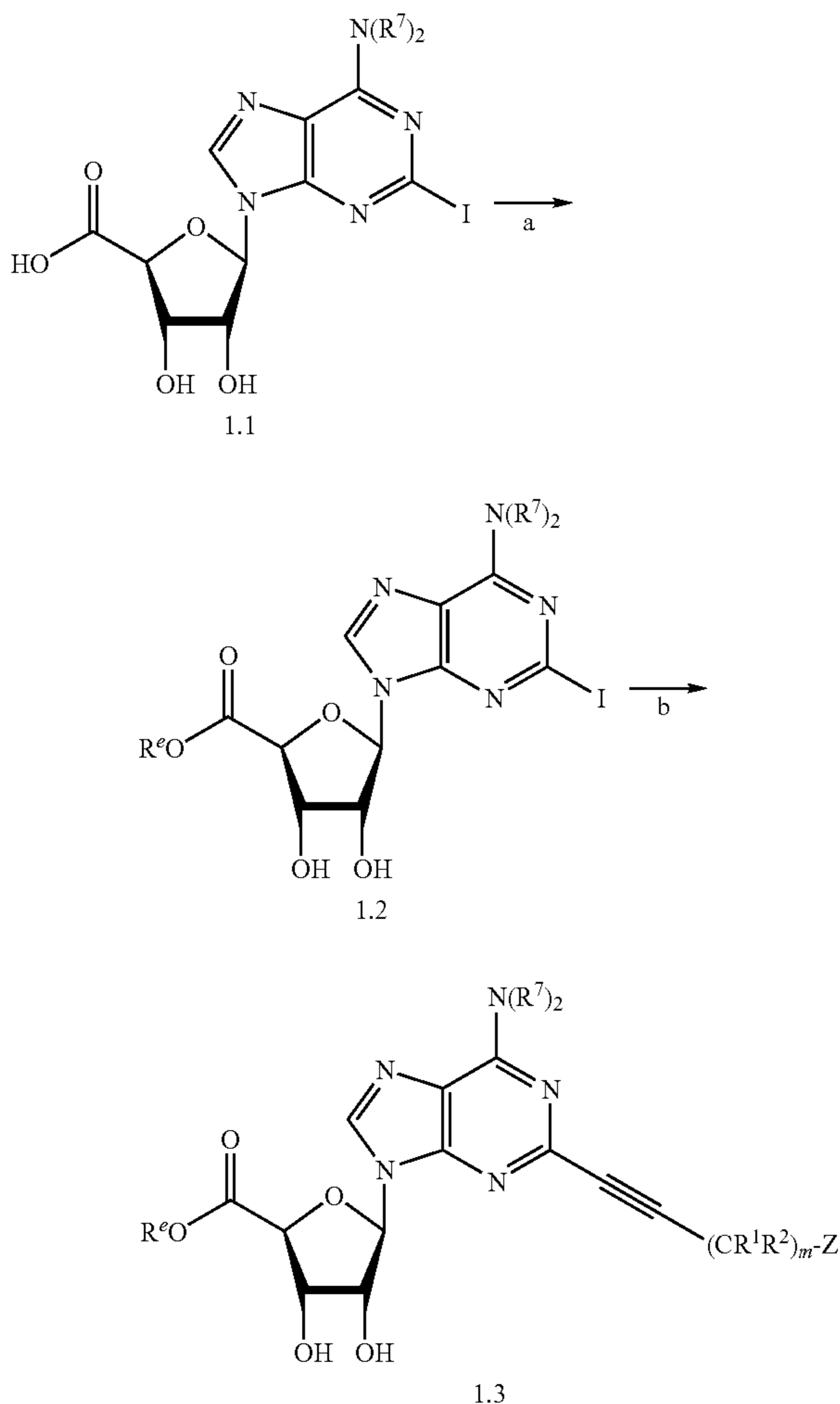
Scheme 1: Preparation of 5' ester analogs:
