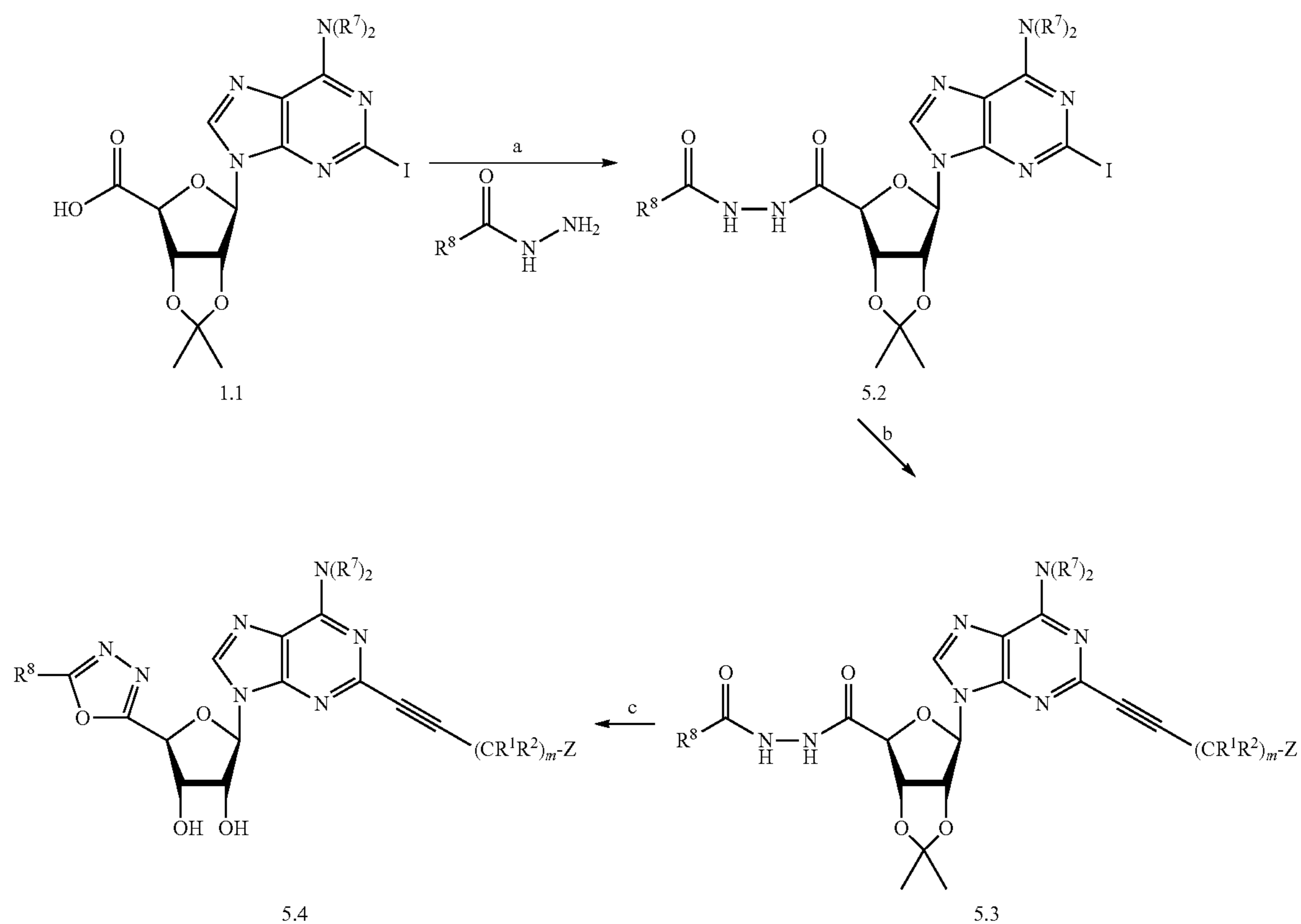
Scheme 5: Preparation of 4'-1,3,4 oxadiazoles
