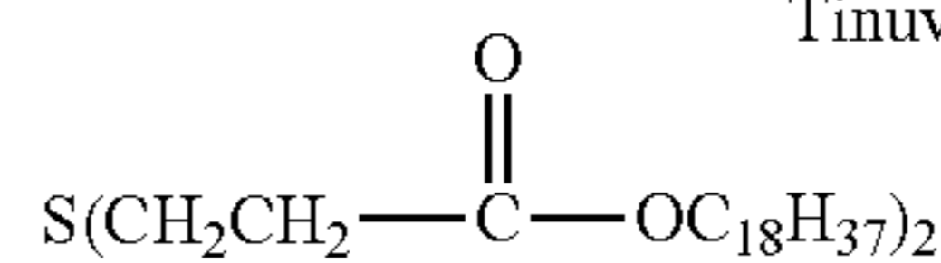
CYANOX STDP
