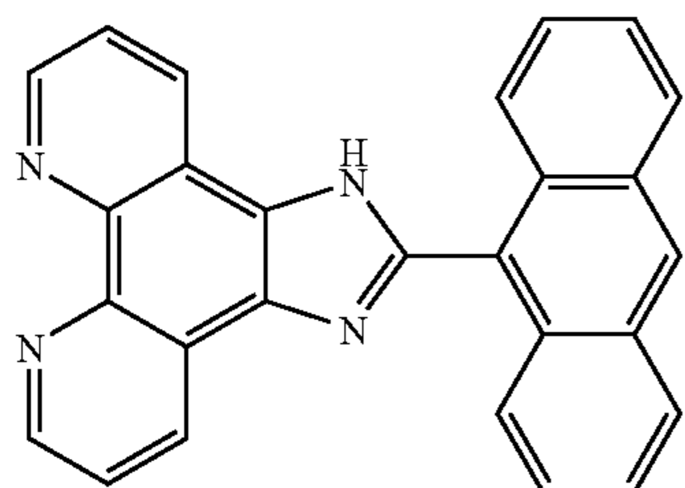
PhenImAn: 2-(9-anthryl)imidazo[4,5-f]-[1,10]phenanthroline (2)
