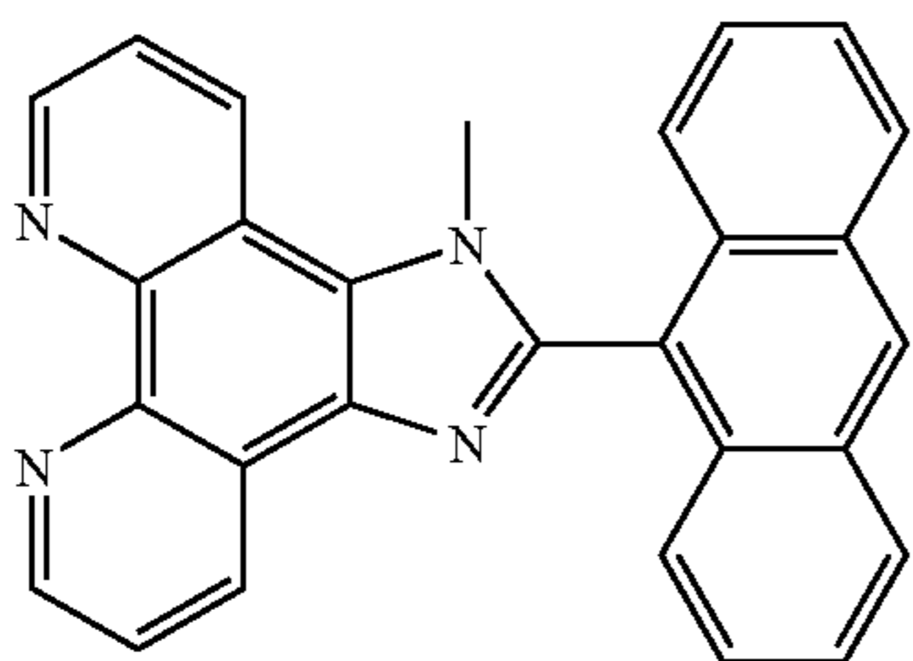
MePhenImAn: 1-methyl-2-(9-anthryl)imidazo[4,5-f]-[1,10]phenanthroline (3)
