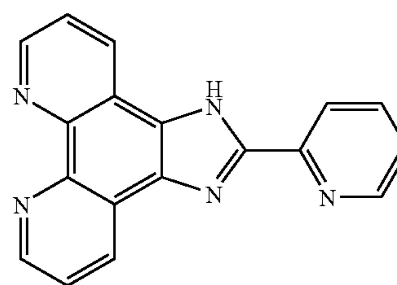
MePhenImPy: 1-methyl-2-(2-pyridyl)imidazo[4,5-f]-[1,10]phenanthroline (5)
