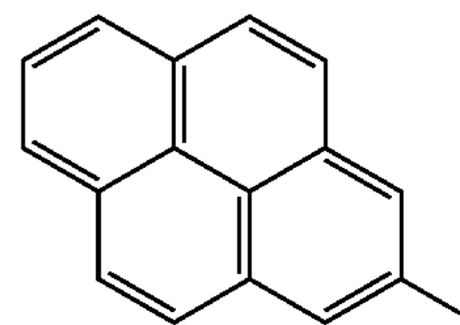
2-pyrenyl
