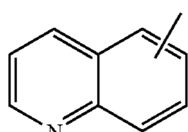
quinolinyl
