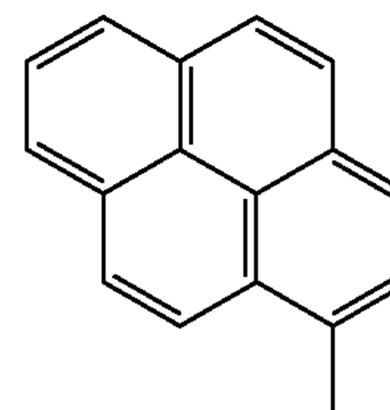
1-pyrenyl
