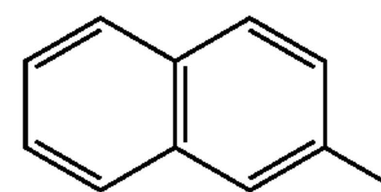
2-naphthyl
