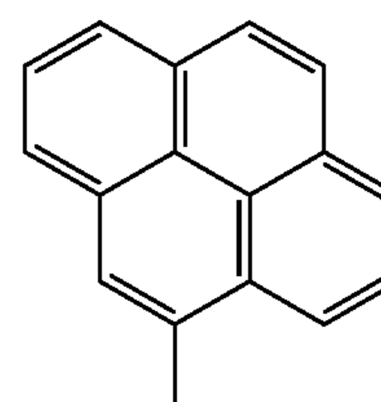
4-pyrenyl
