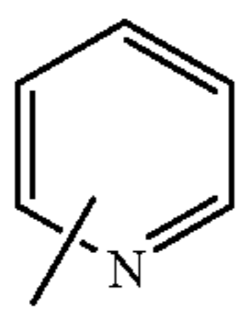
pyridyl
