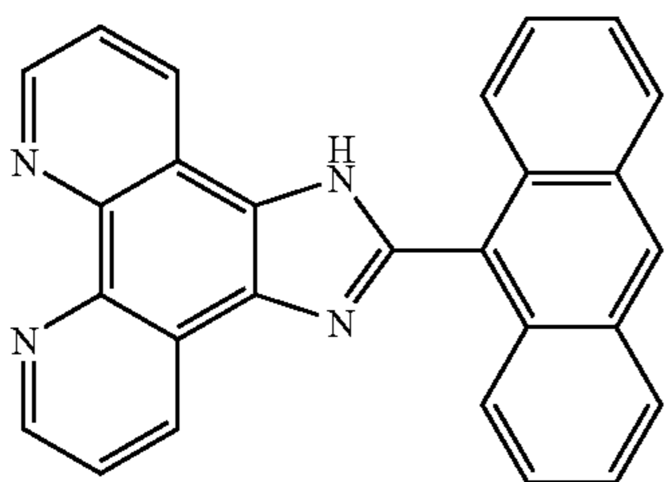
PhenImAn: 2-(9-anthryl)imidazo[4,5-f]-[1,10]phenanthroline (2)
