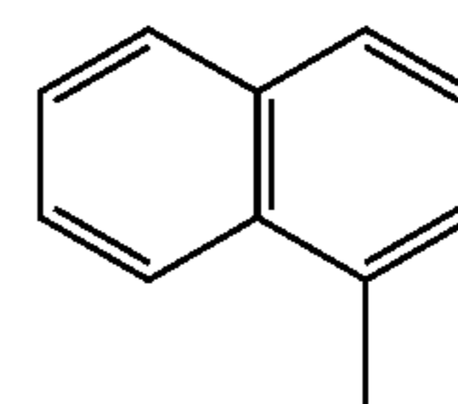
1-naphthyl
