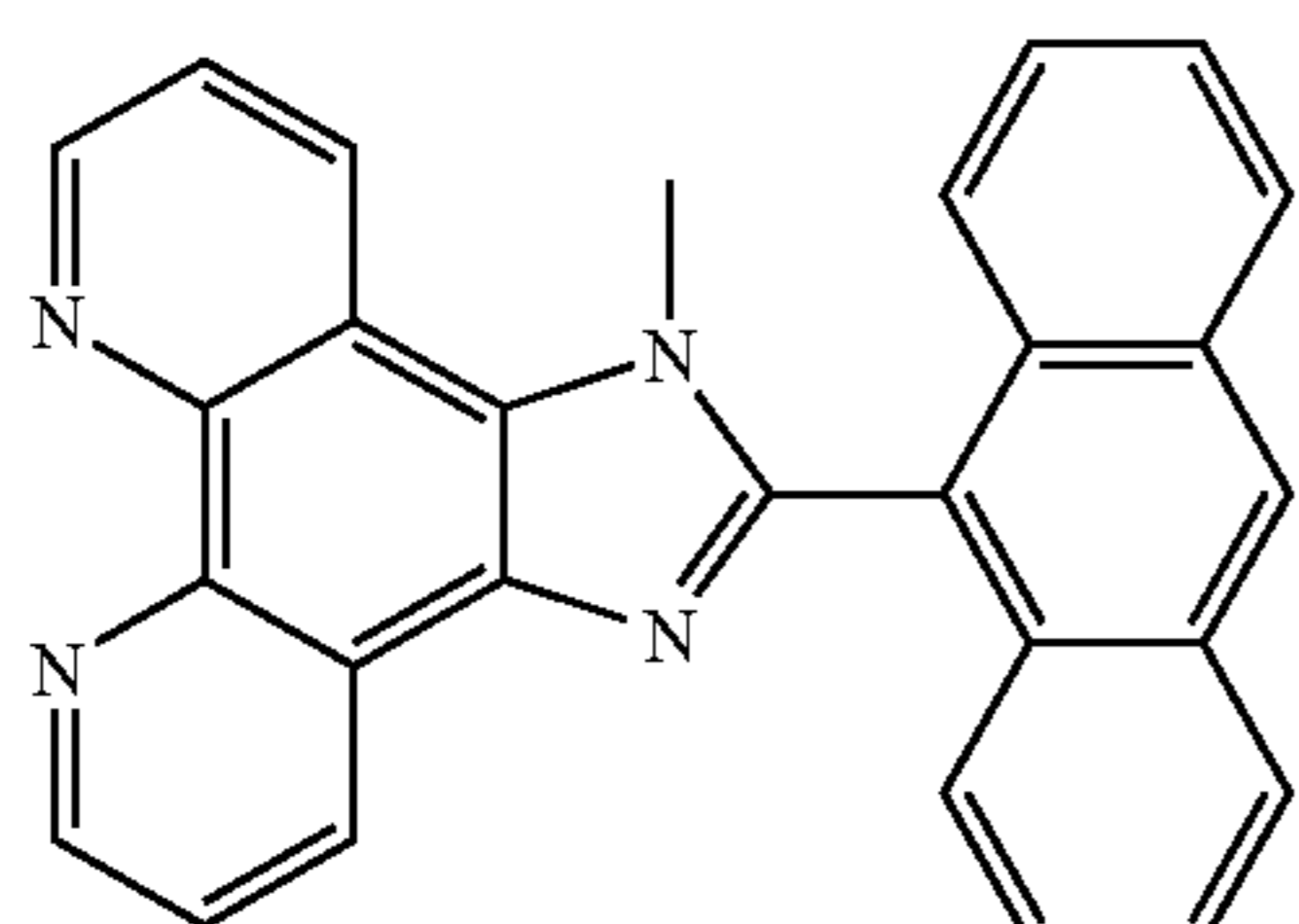
MePhenImAn: 1-methyl-2-(9-anthryl)imidazo[4,5-f]-[1,10]phenanthroline (3)
