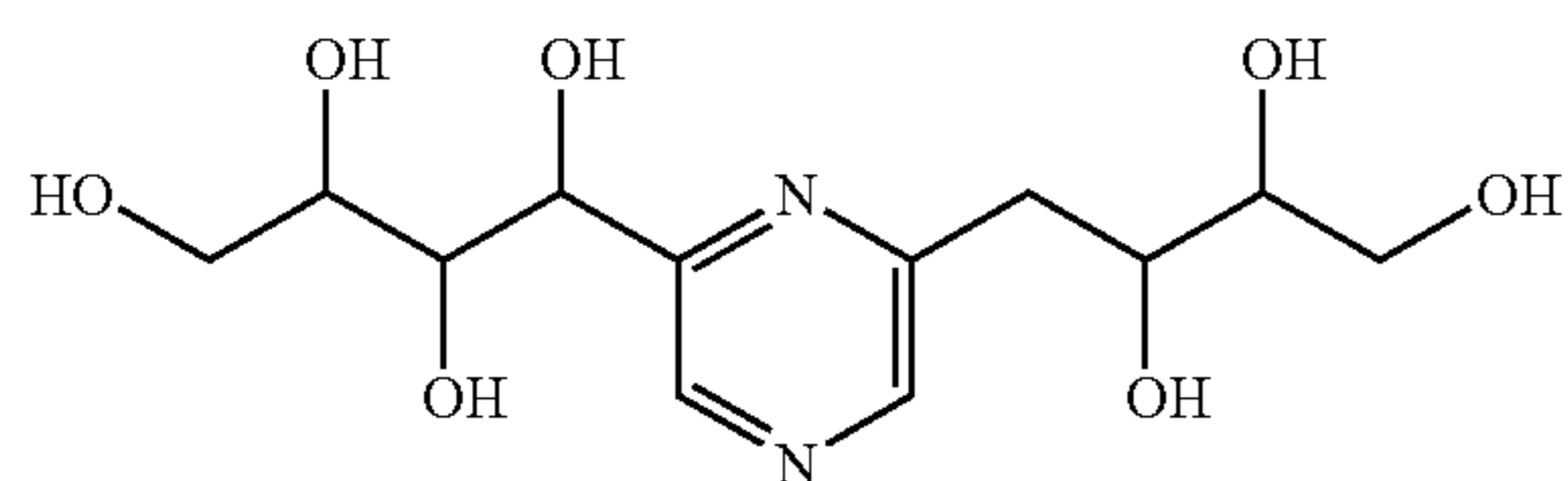
1-[6-(2,3,4-trihydroxybutyl)-pyrazin-2-yl]-butane-1,2,3,4-tetraol (2,6-deoxyfructosazine)
