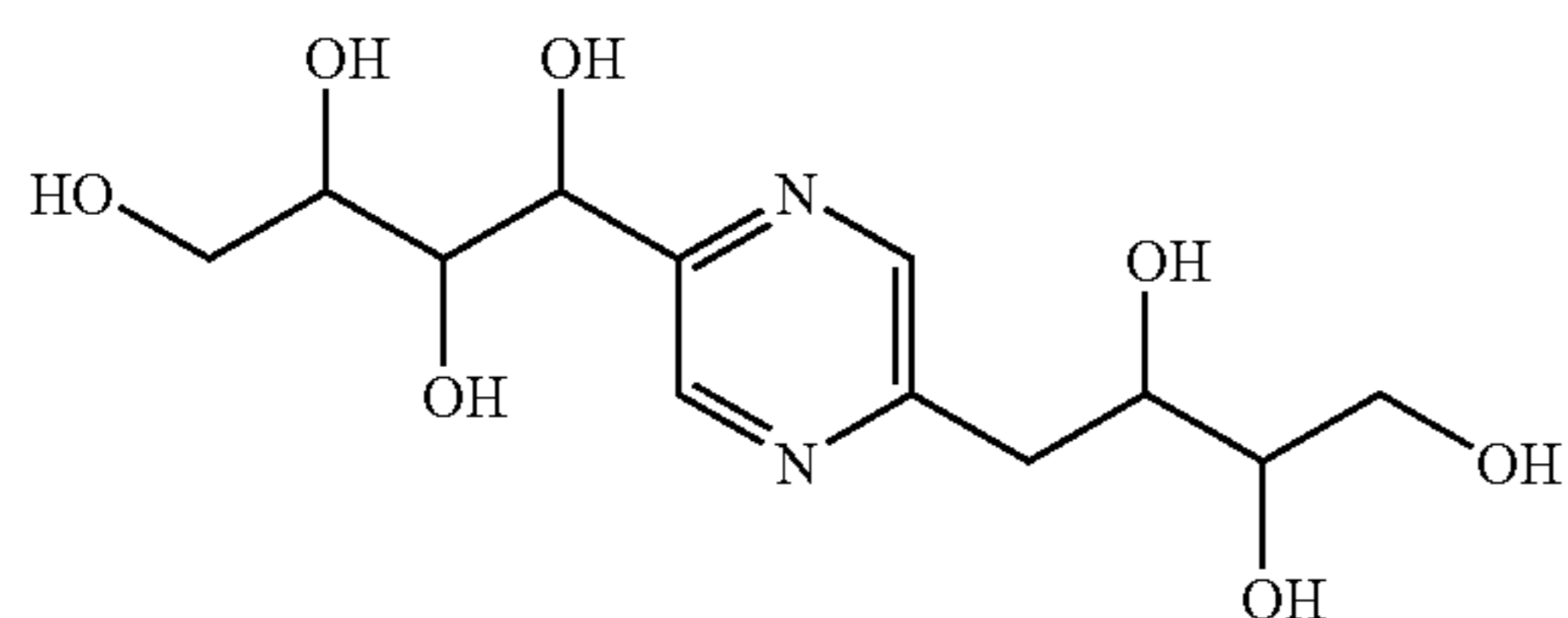
1-[5-(2,3,4-trihydroxybutyl)-pyrazin-2-yl]-butane-1,2,3,4-tetraol (2,5-deoxyfructosazine)
