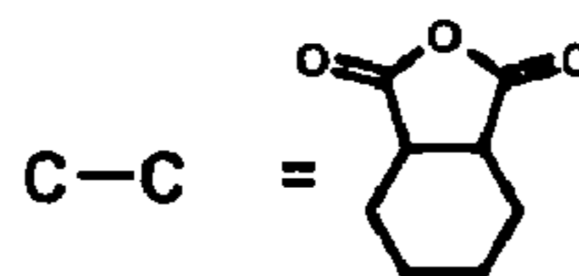
monomer C 2
