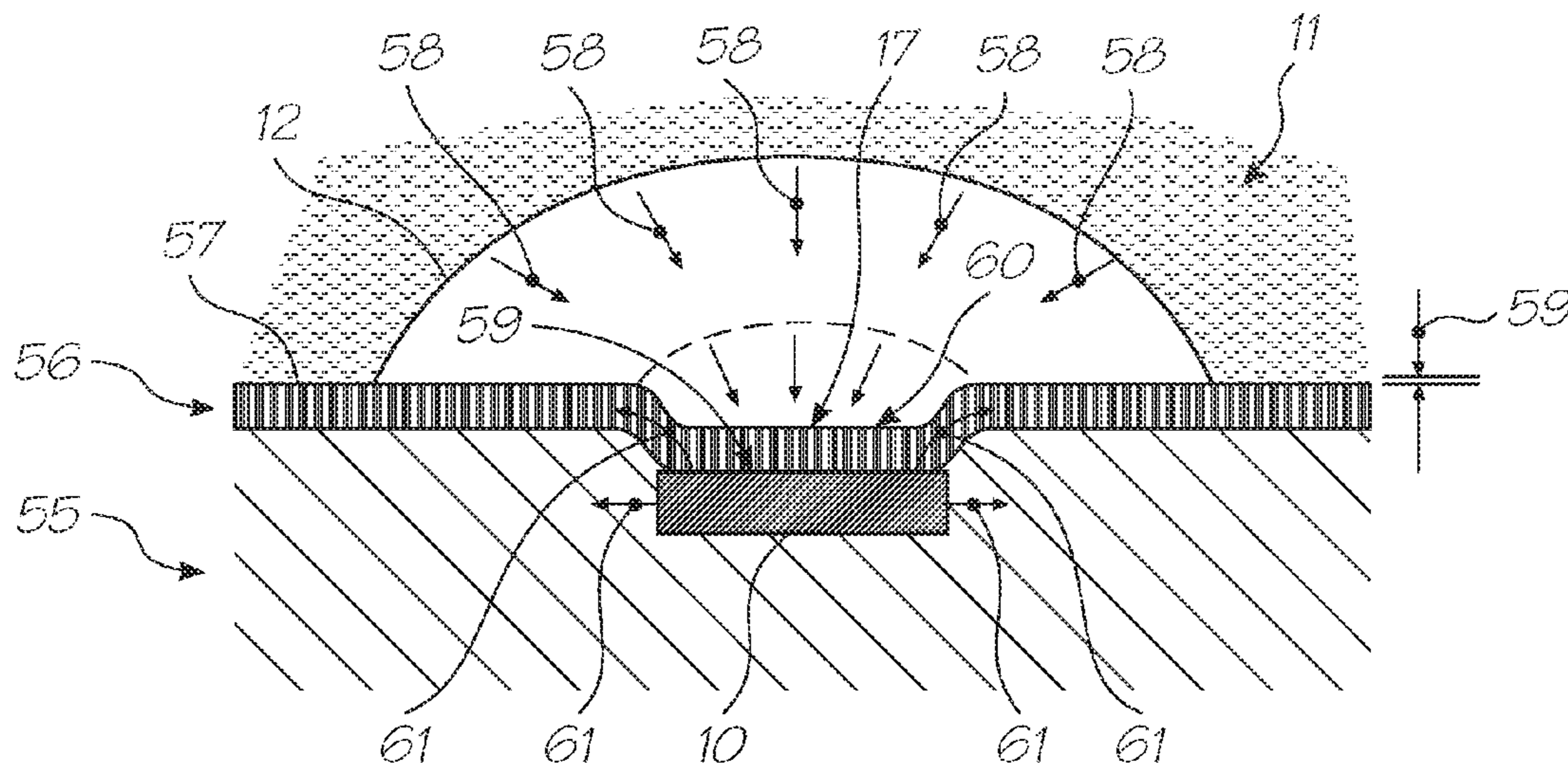
FIG. 47 (PRIOR ART)
