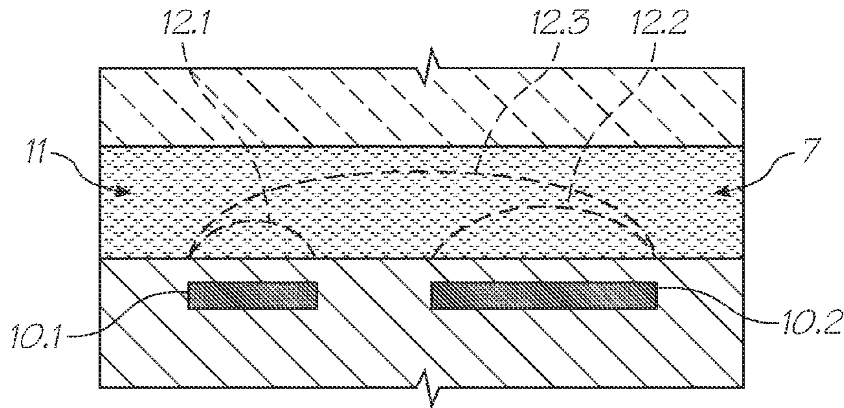
FIG. 52 (PRIOR ART)
