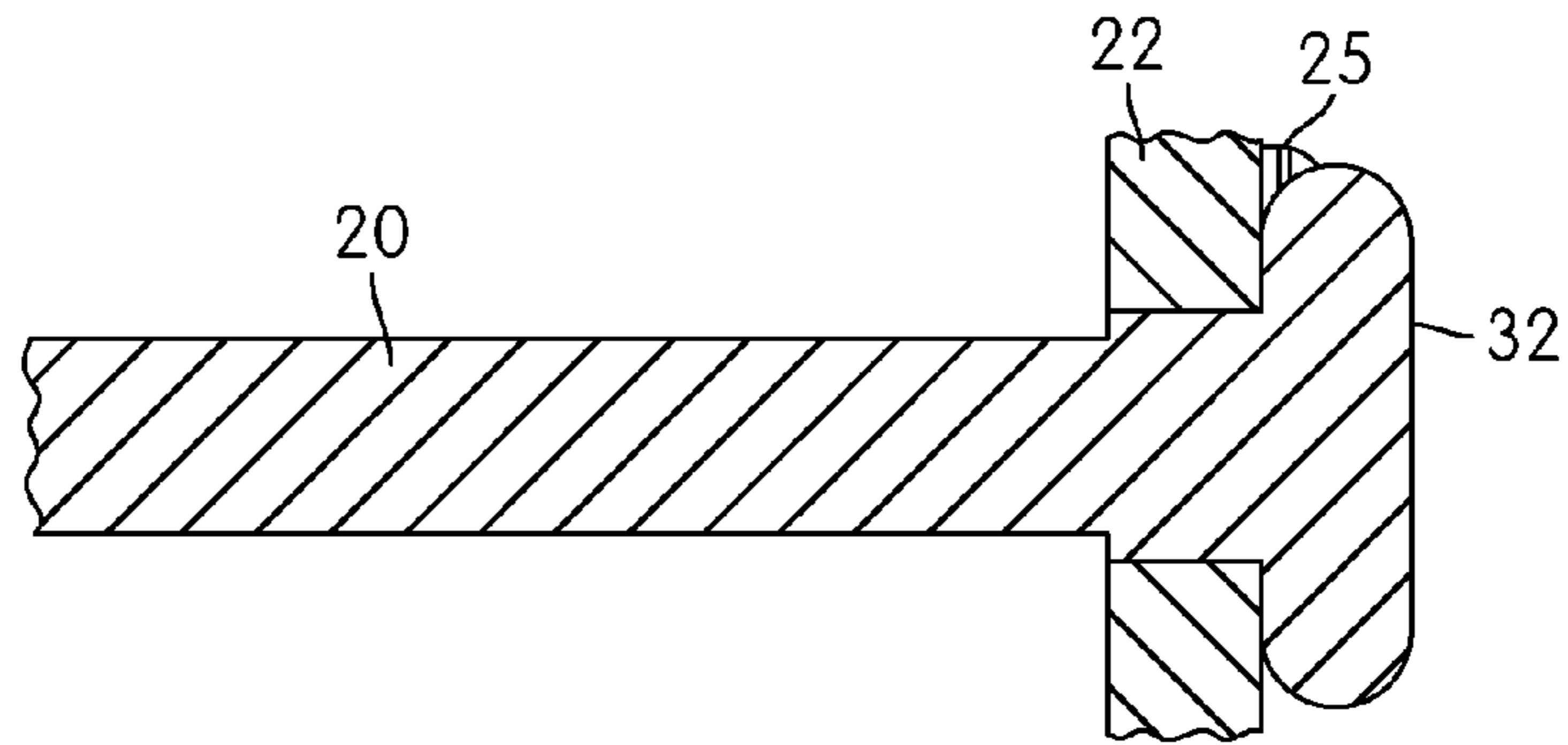
FIG. 5 (PRIOR ART)
