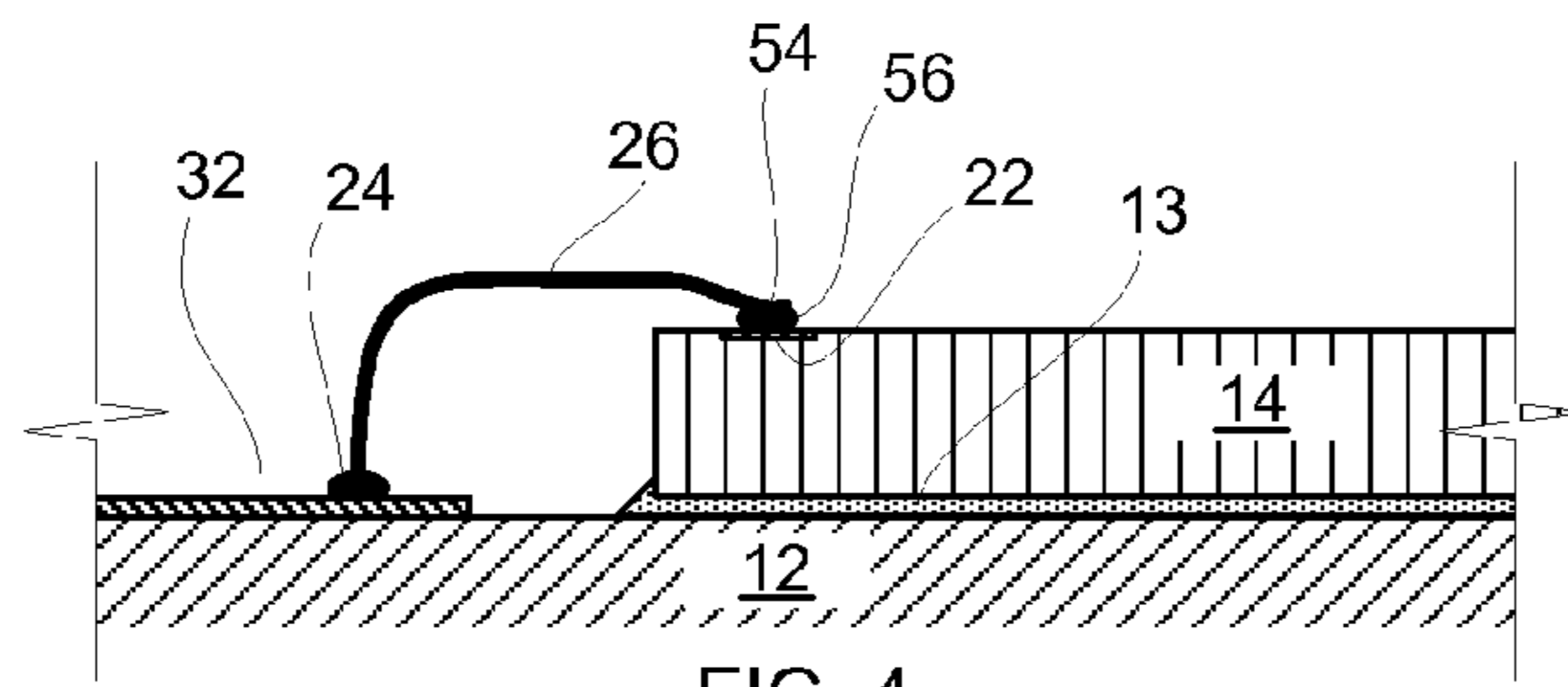
FIG. 4 (PRIOR ART)
