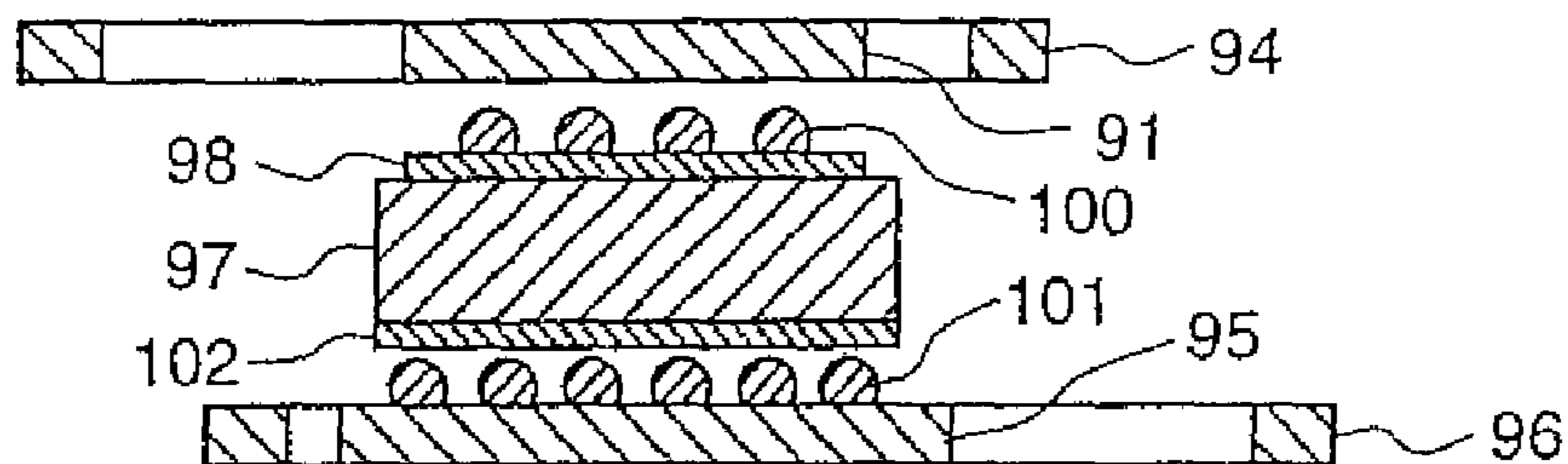
LAMINATED CROSS SECTIONAL STRUCTURE AT BONDING
