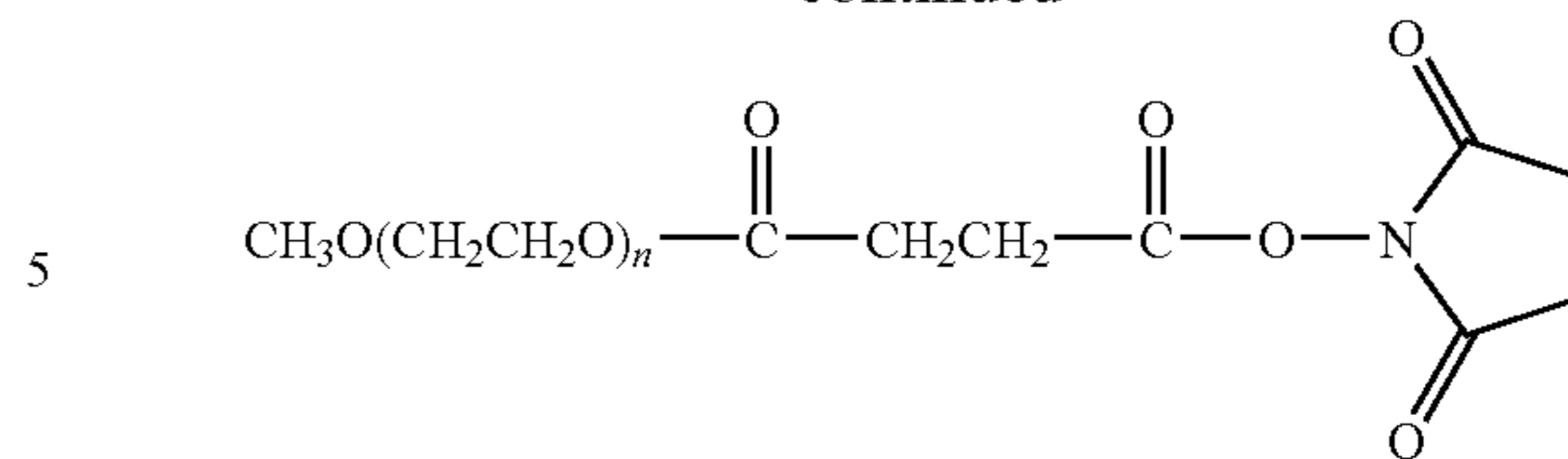
mPEG Succinimidyl succinate x = glutarate
