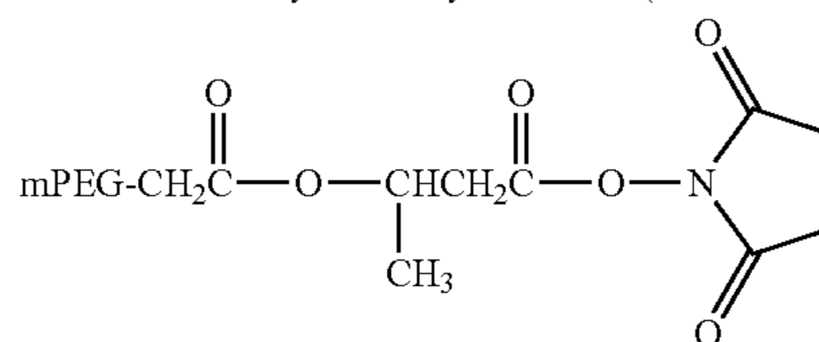
mPEG-CM-HBA-NHS (CM = carboxymethyl; HBA = Hydroxy butyric acid)
