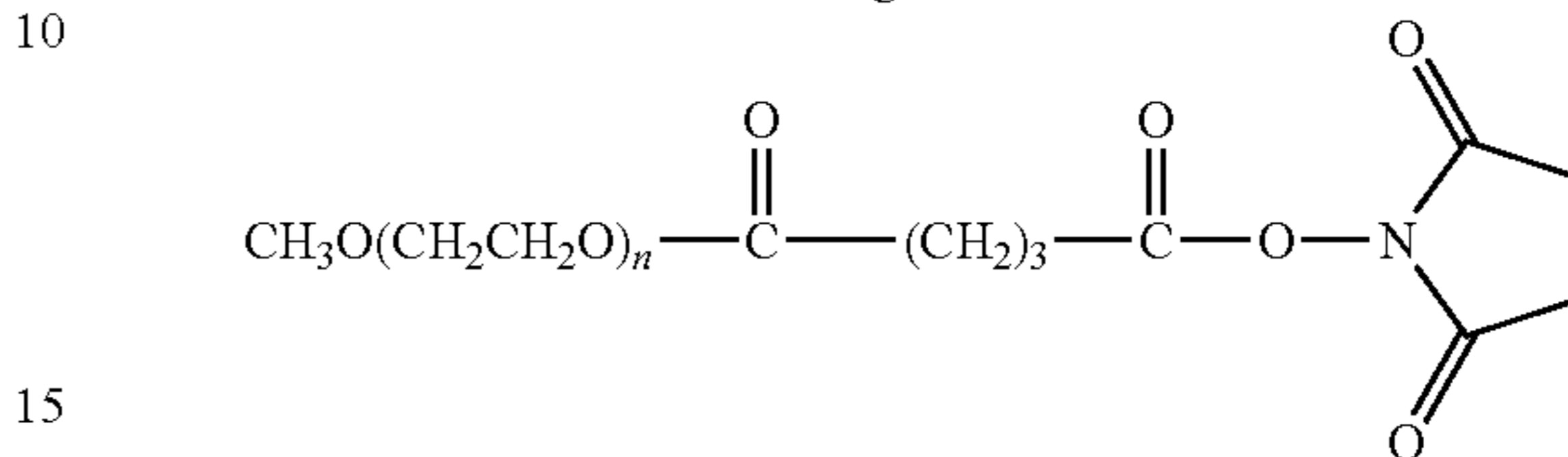
mPEG Succinimidyl glutarate
