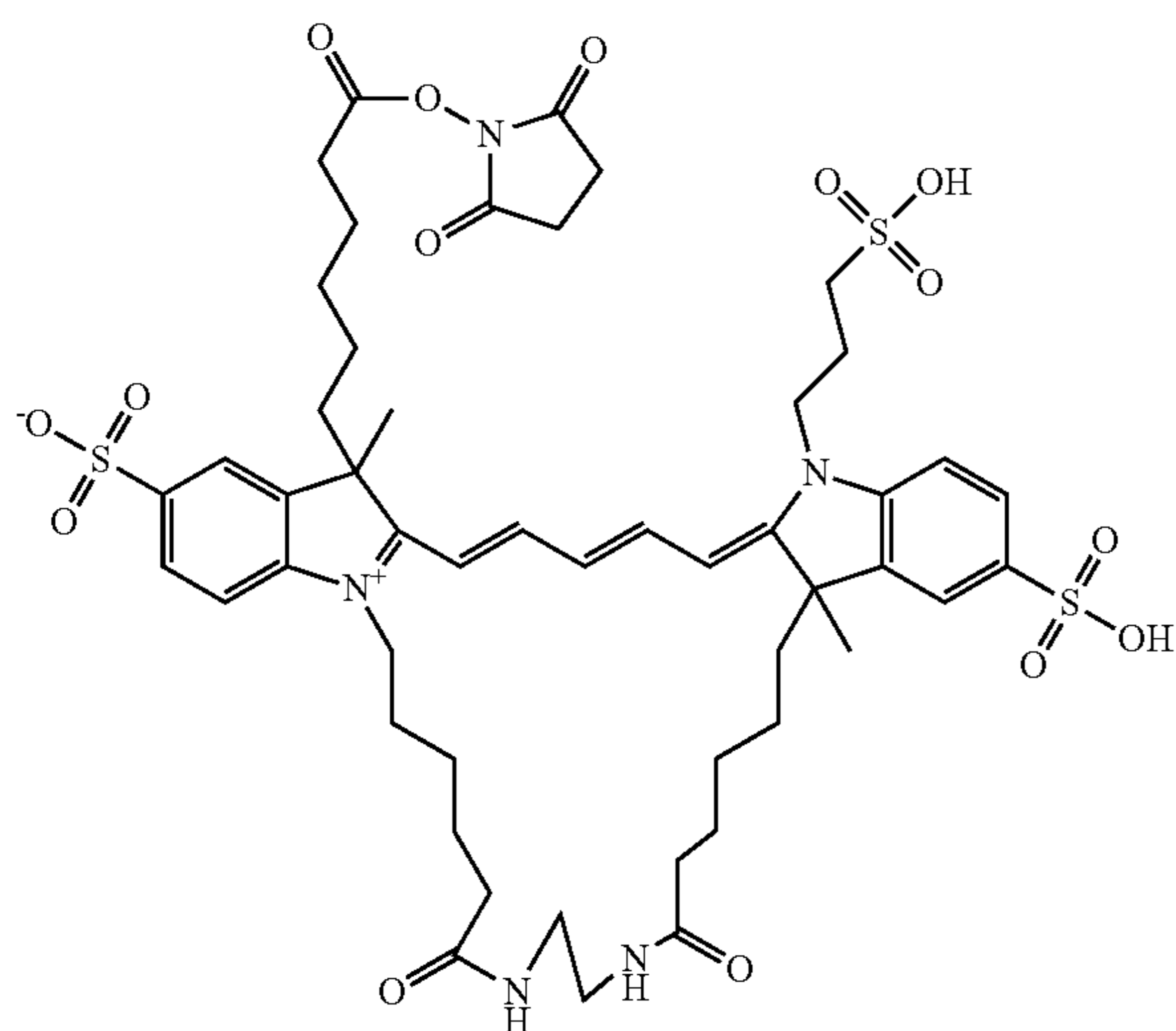
Compound 17
