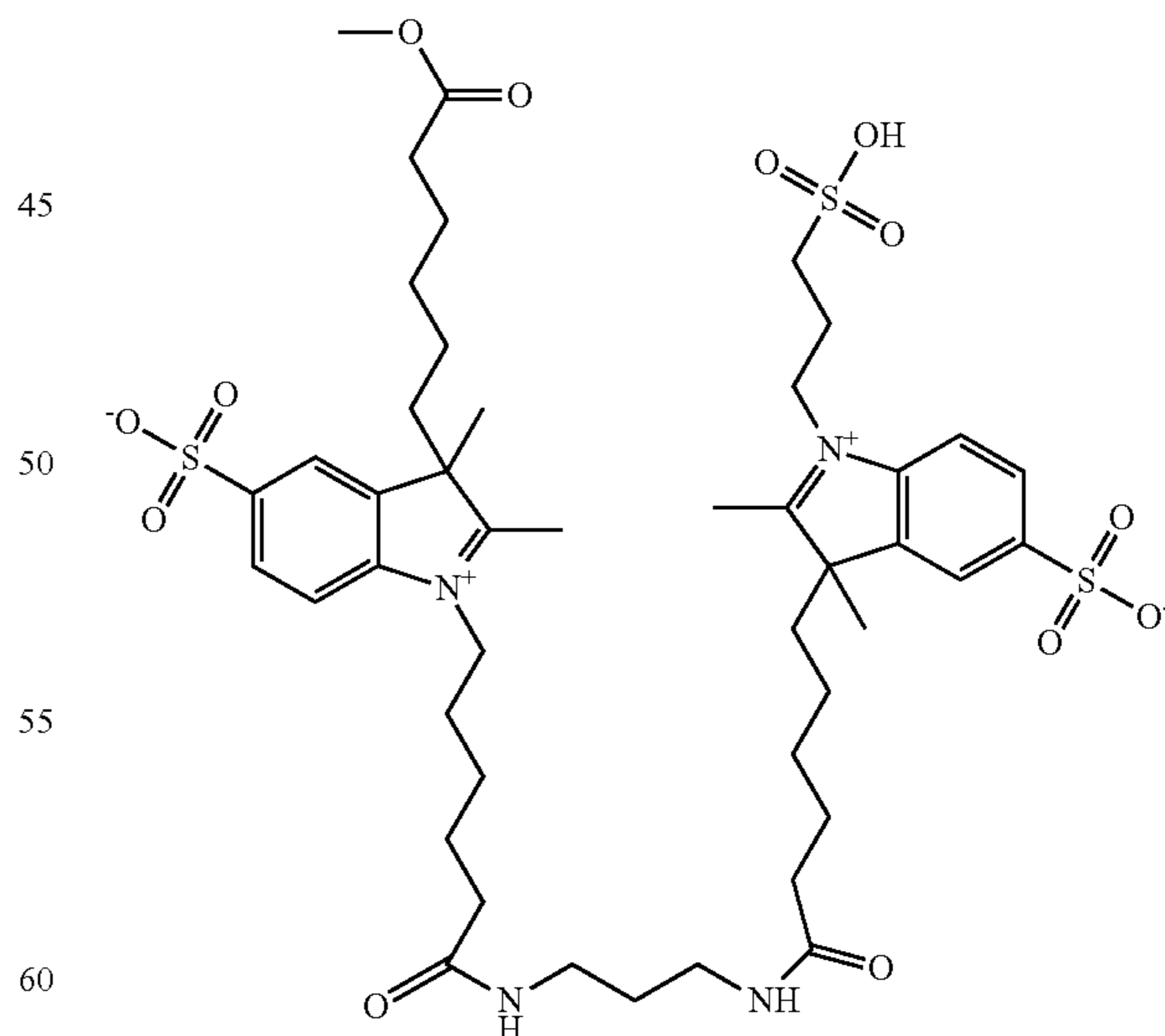
Compound 48
