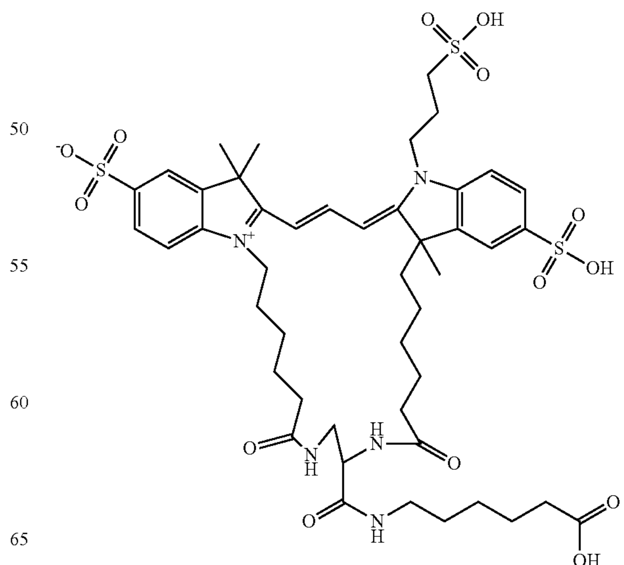
Compound 19
