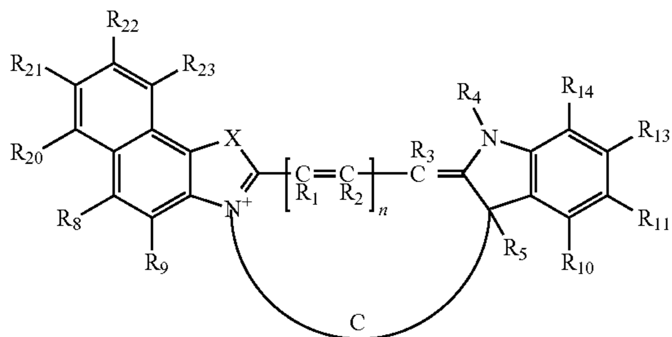
Formula VII
