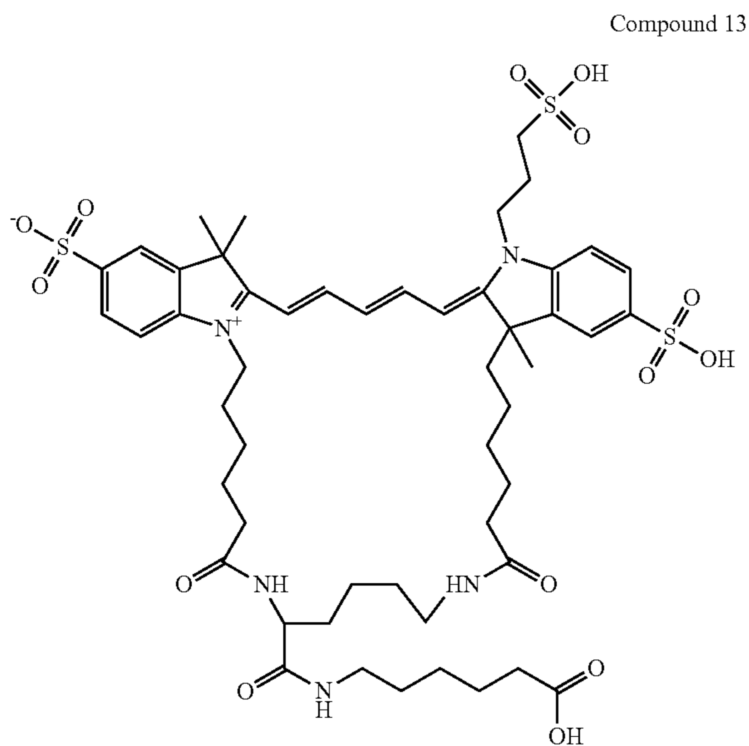
Example 14
