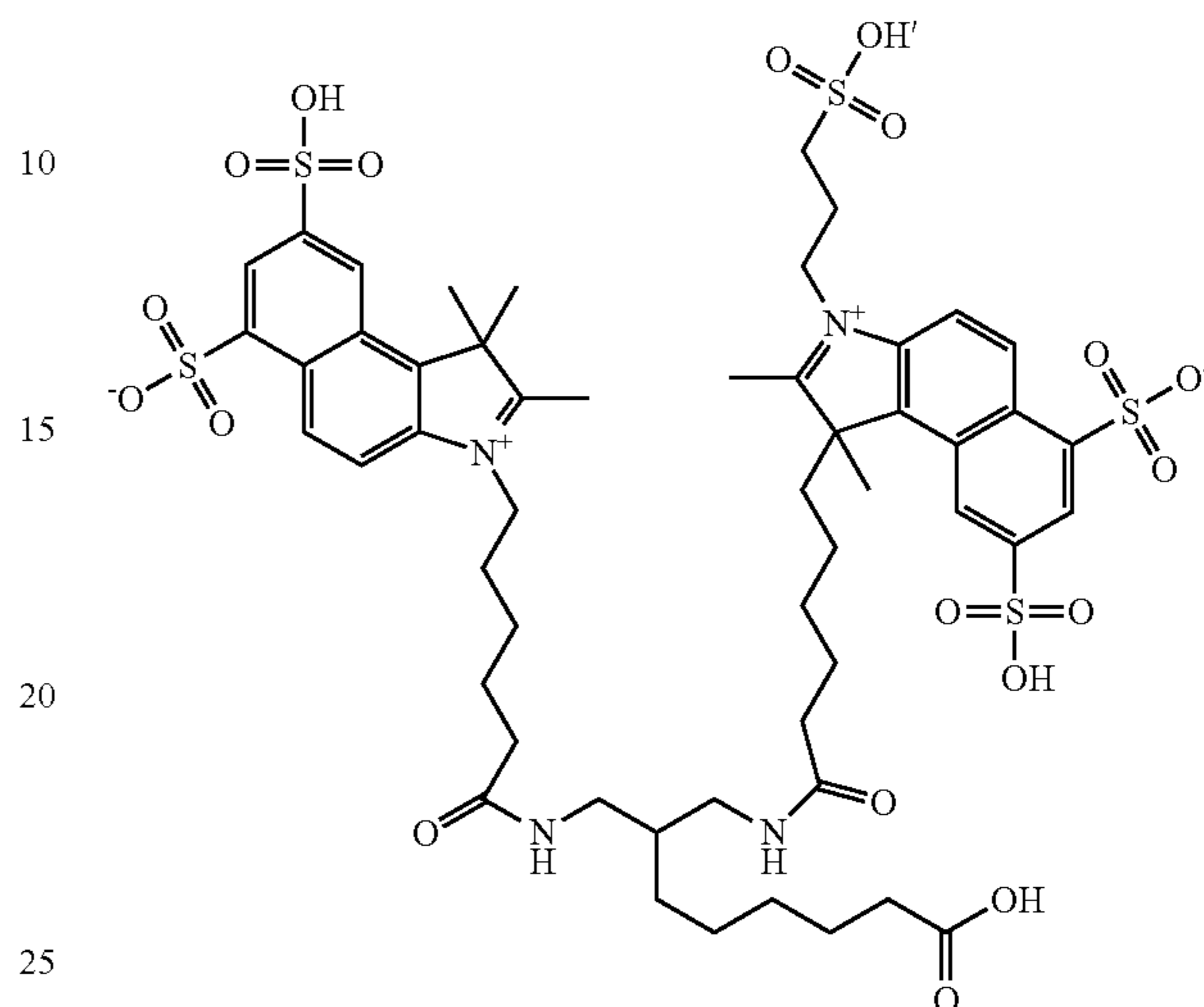
Compound 47
