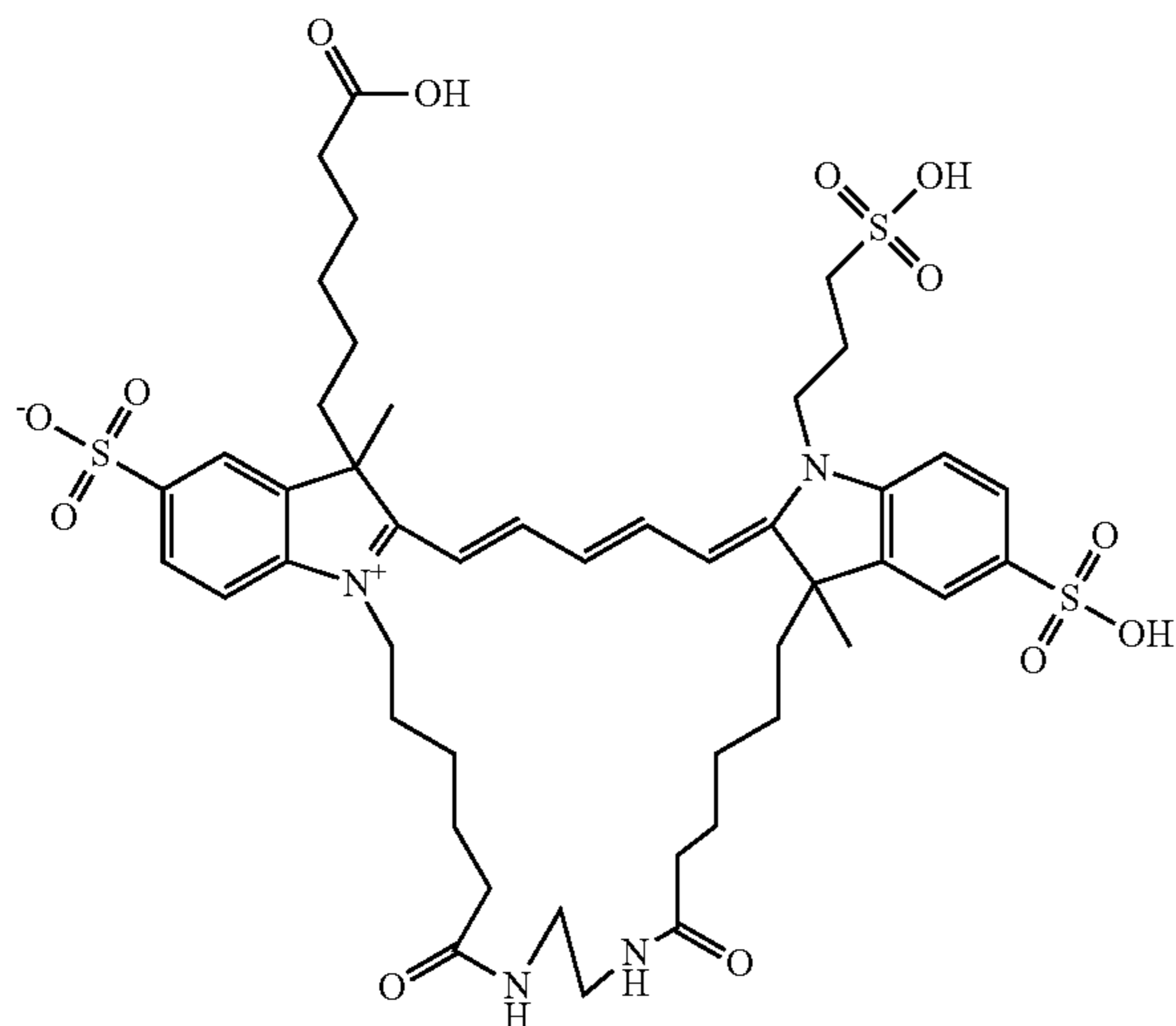
Compound 16
