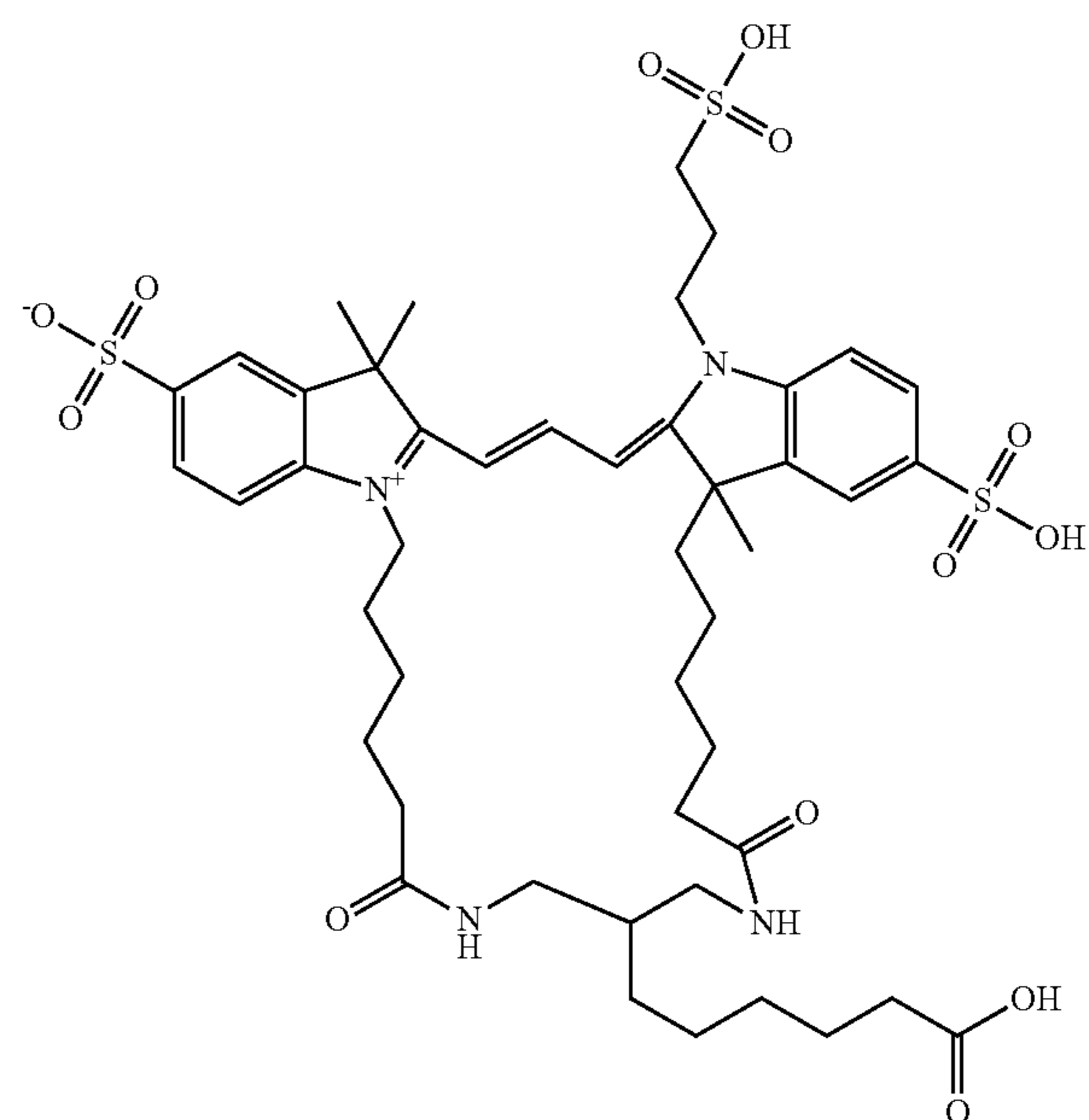
Compound 51
