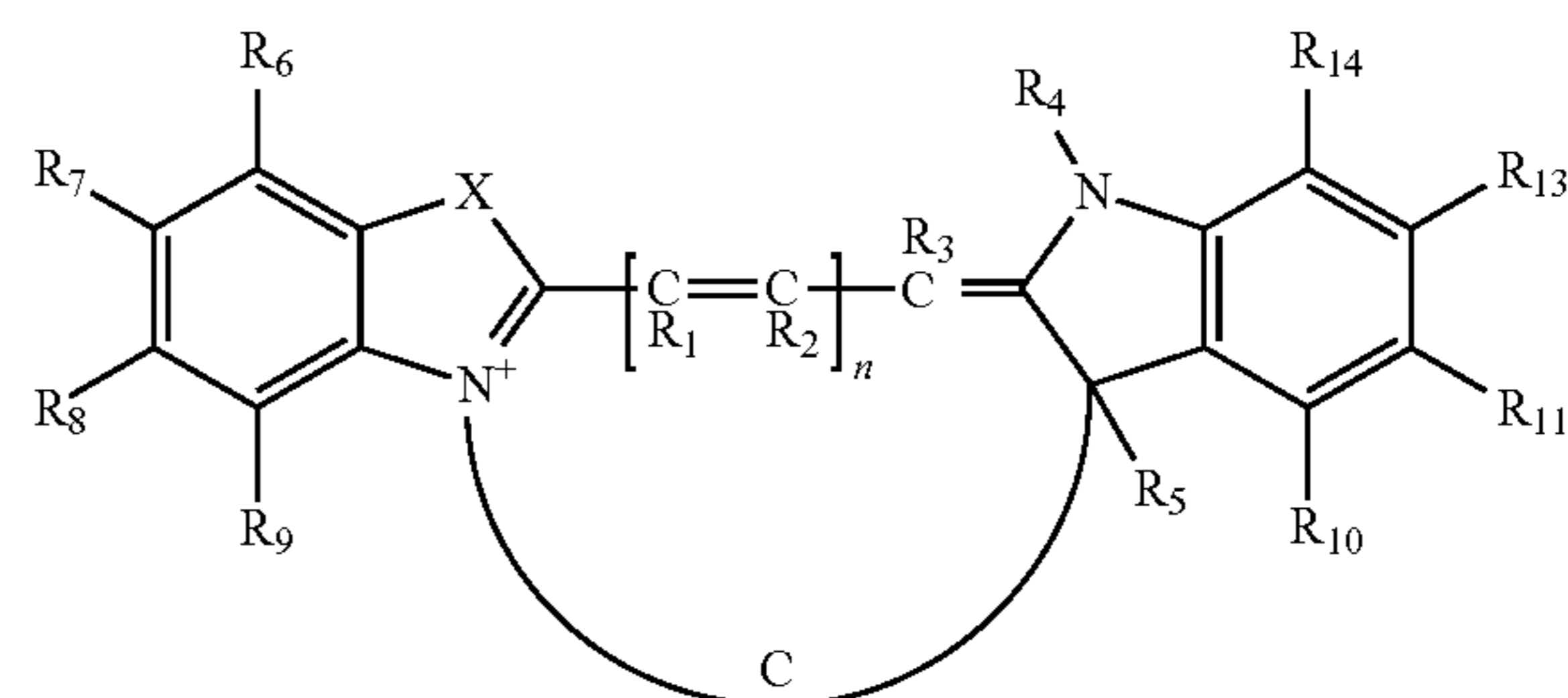
Formula II
