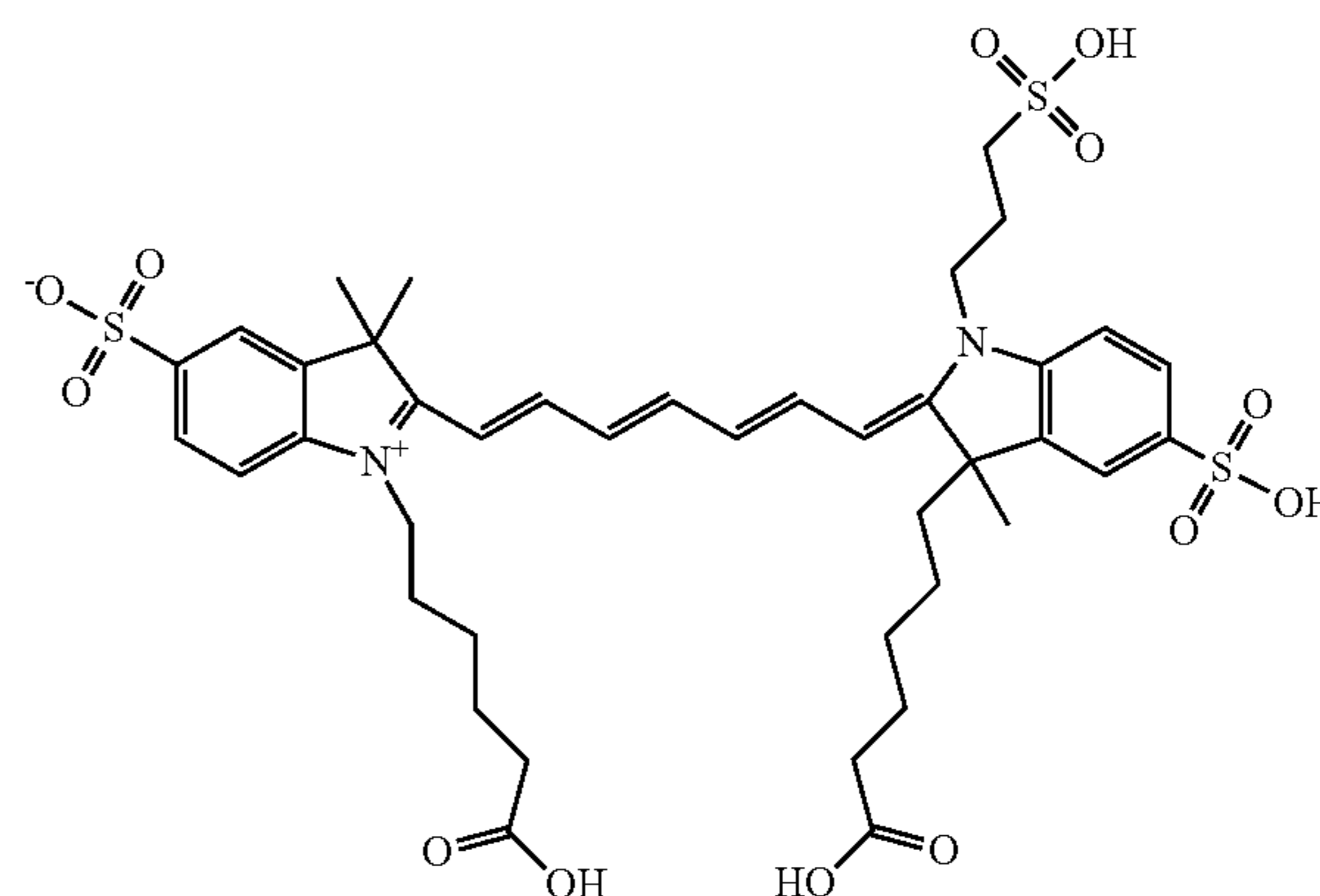
Compound 21
