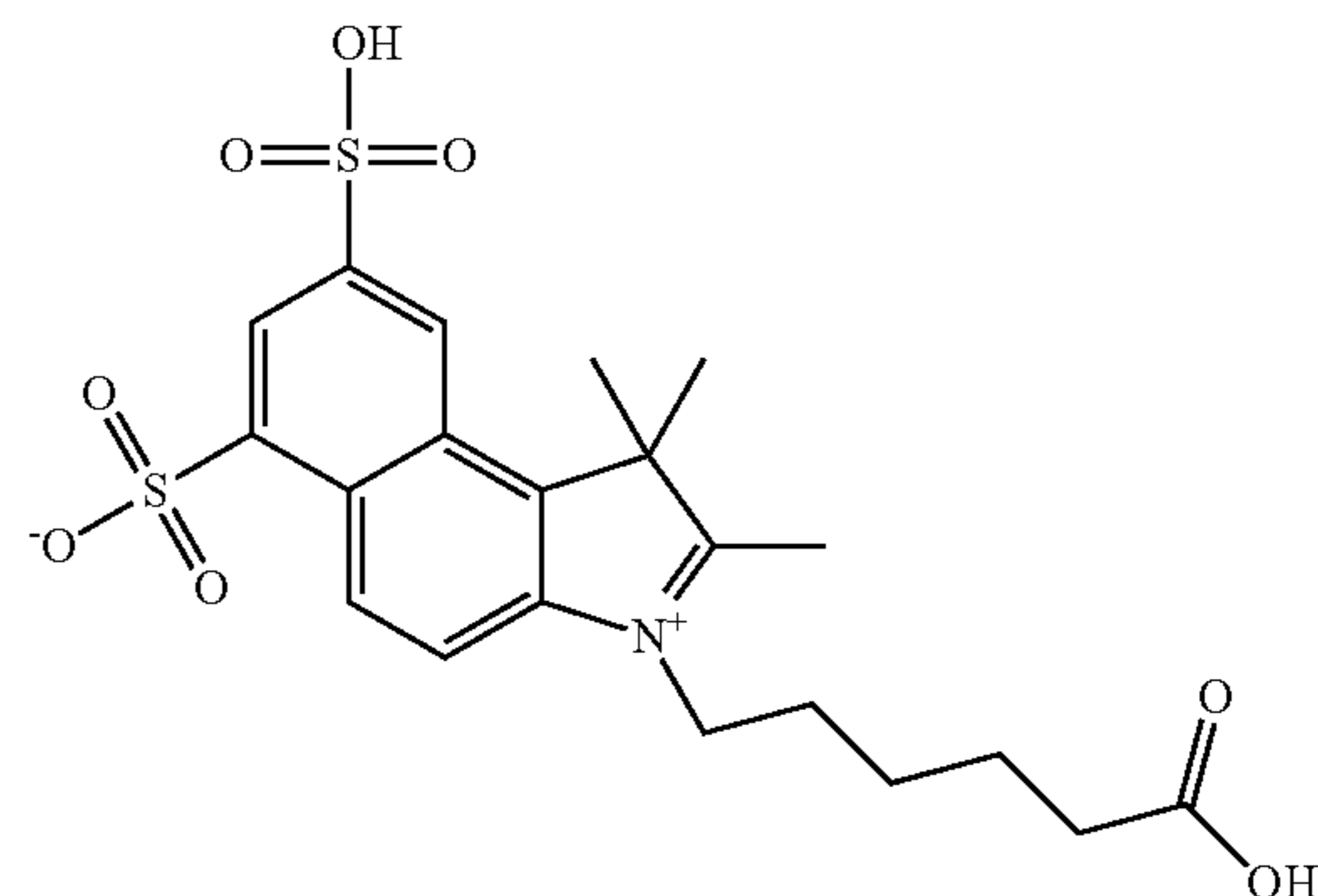
Compound 27
