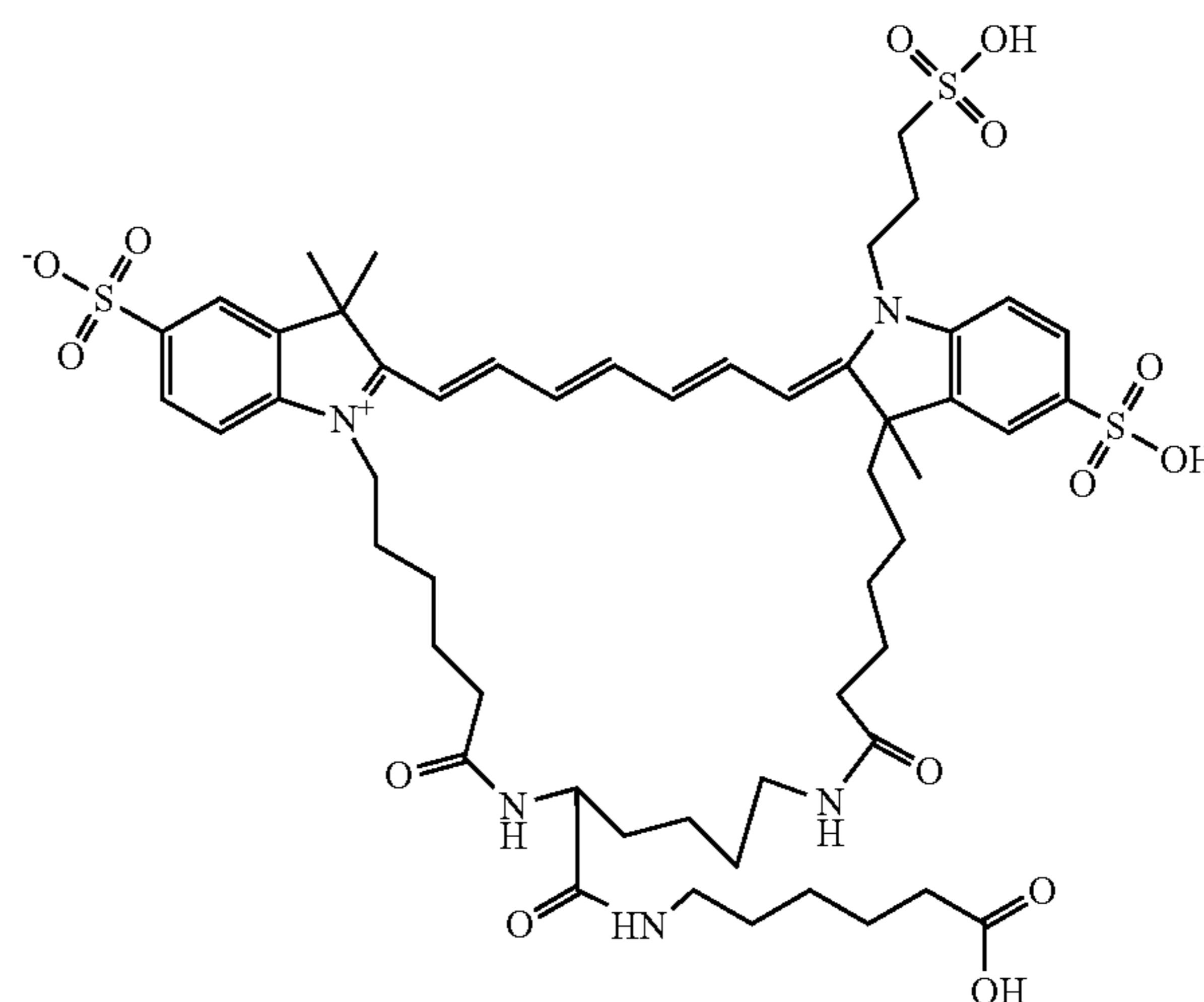
Compound 22
