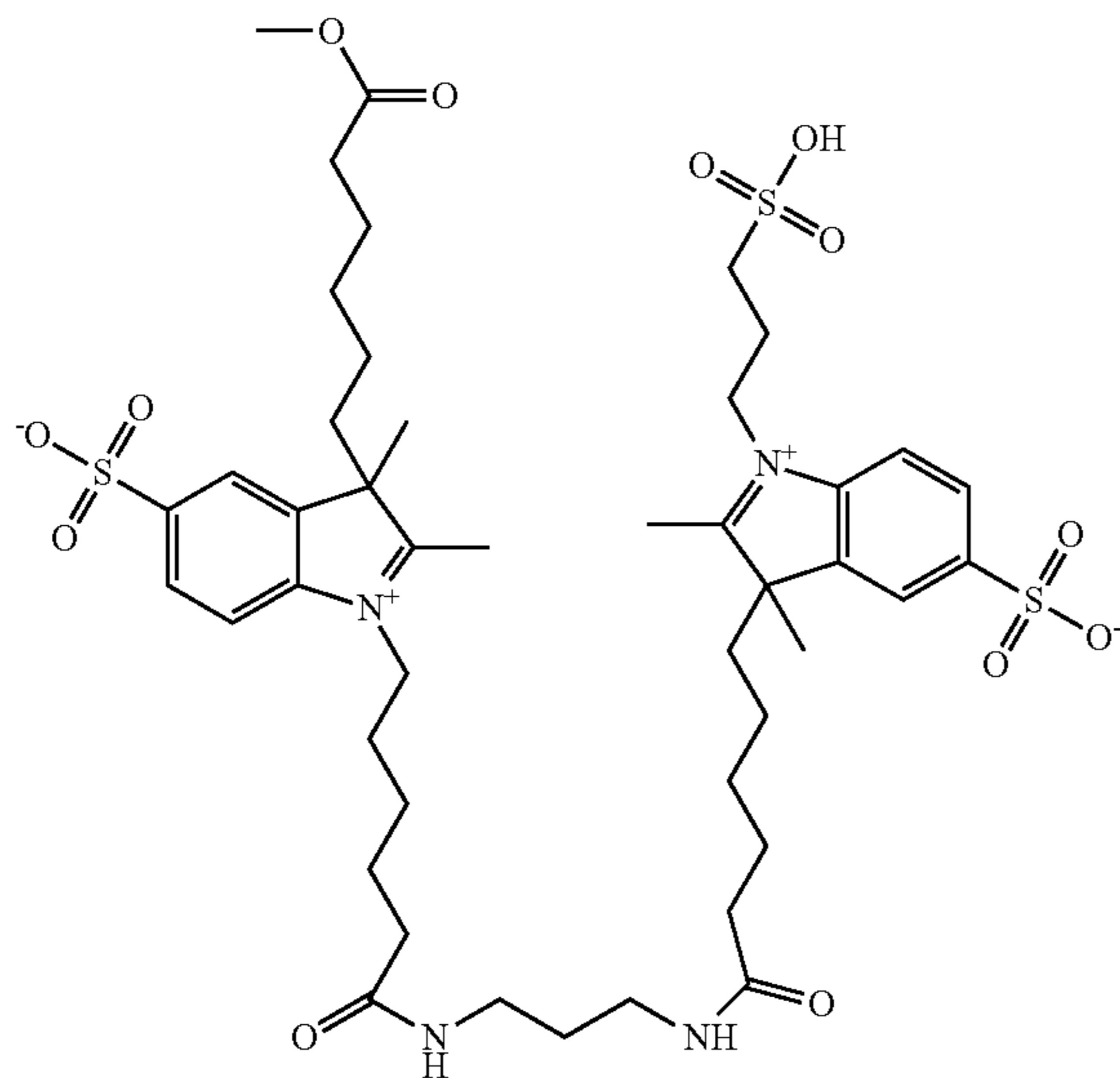
Example 49
