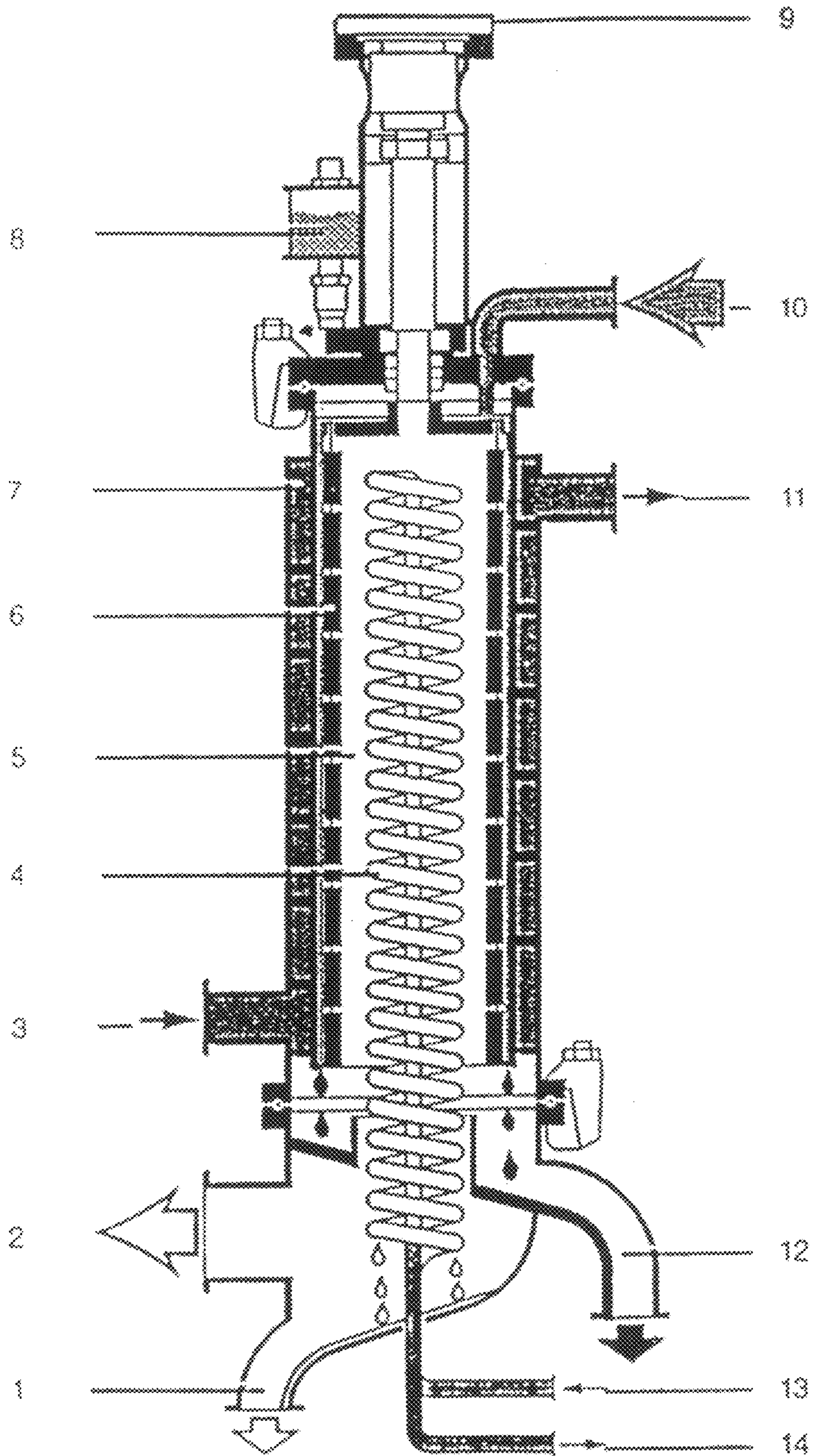
SHORT PATH DISTILLATION APPARATUS
