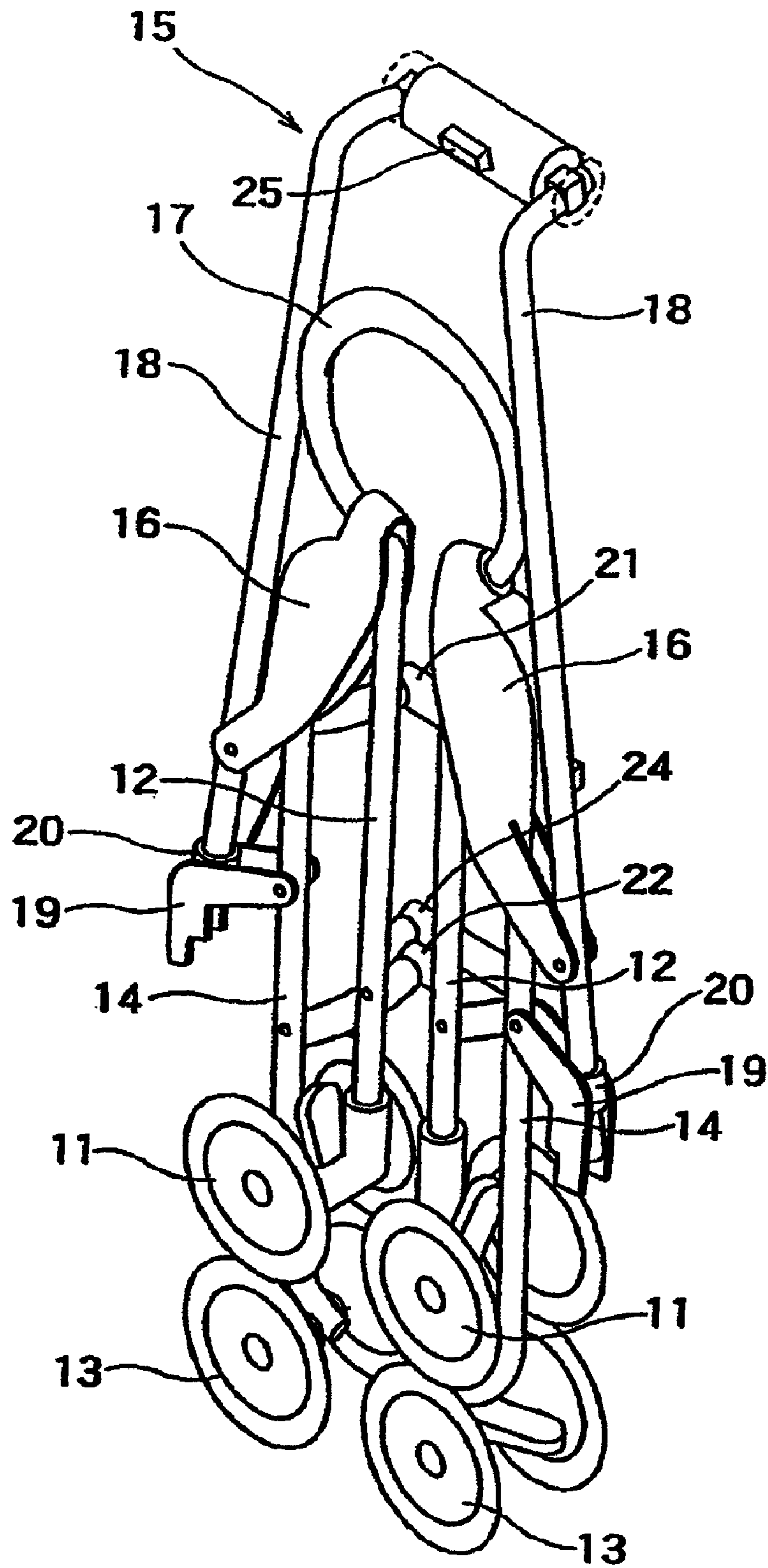
FIG. 15 (PRIOR ART)
