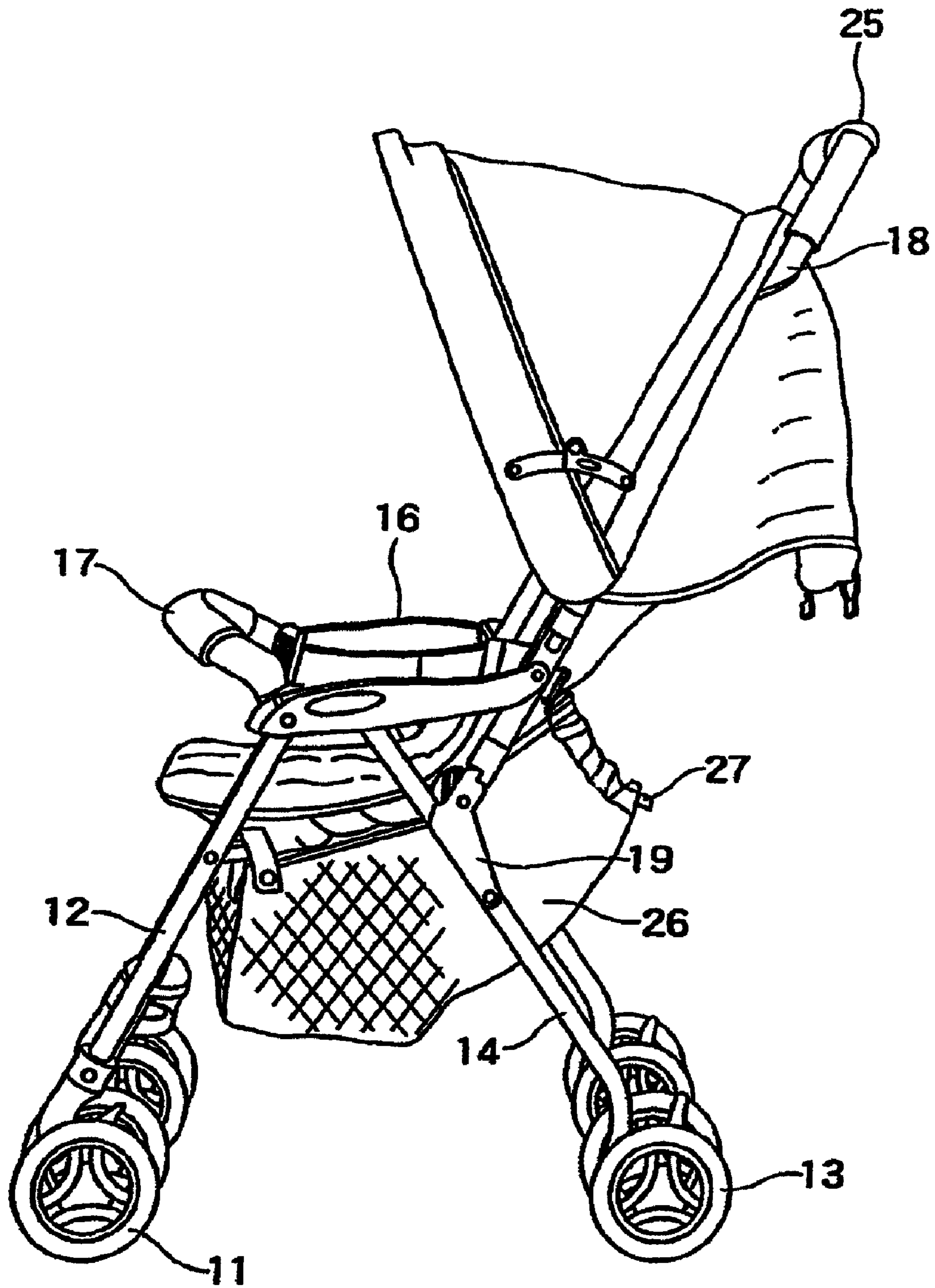
FIG. 16 (PRIOR ART)
