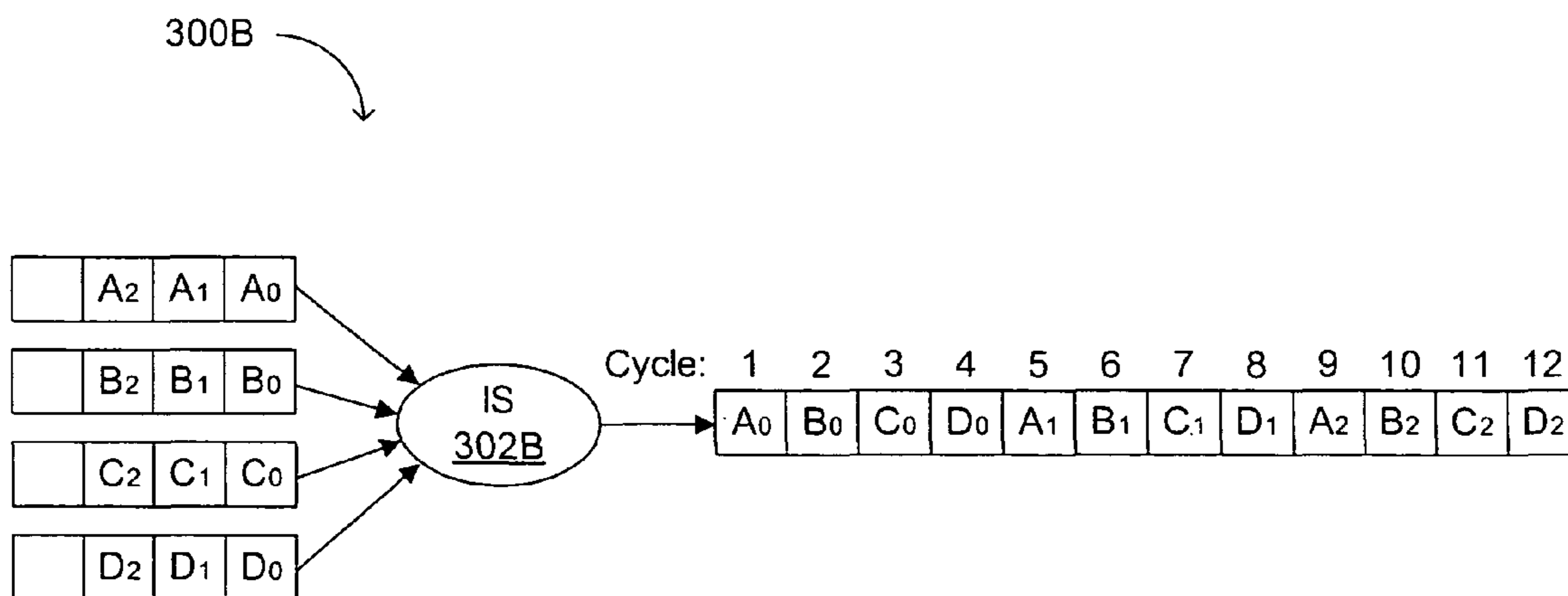
FIG. 3B (conventional)
