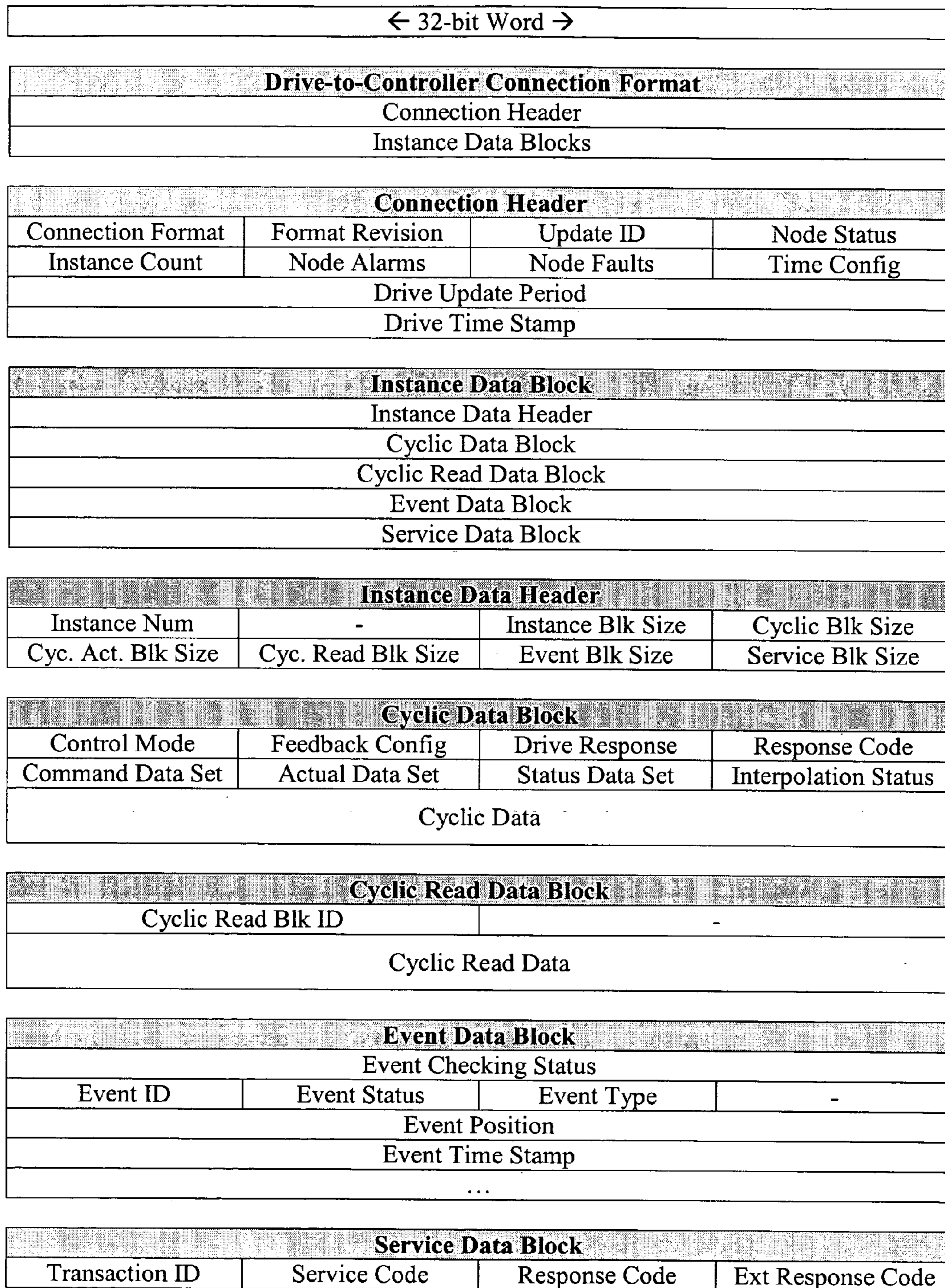
Figure 1-2 — Drive-to-Controller Connection Format
