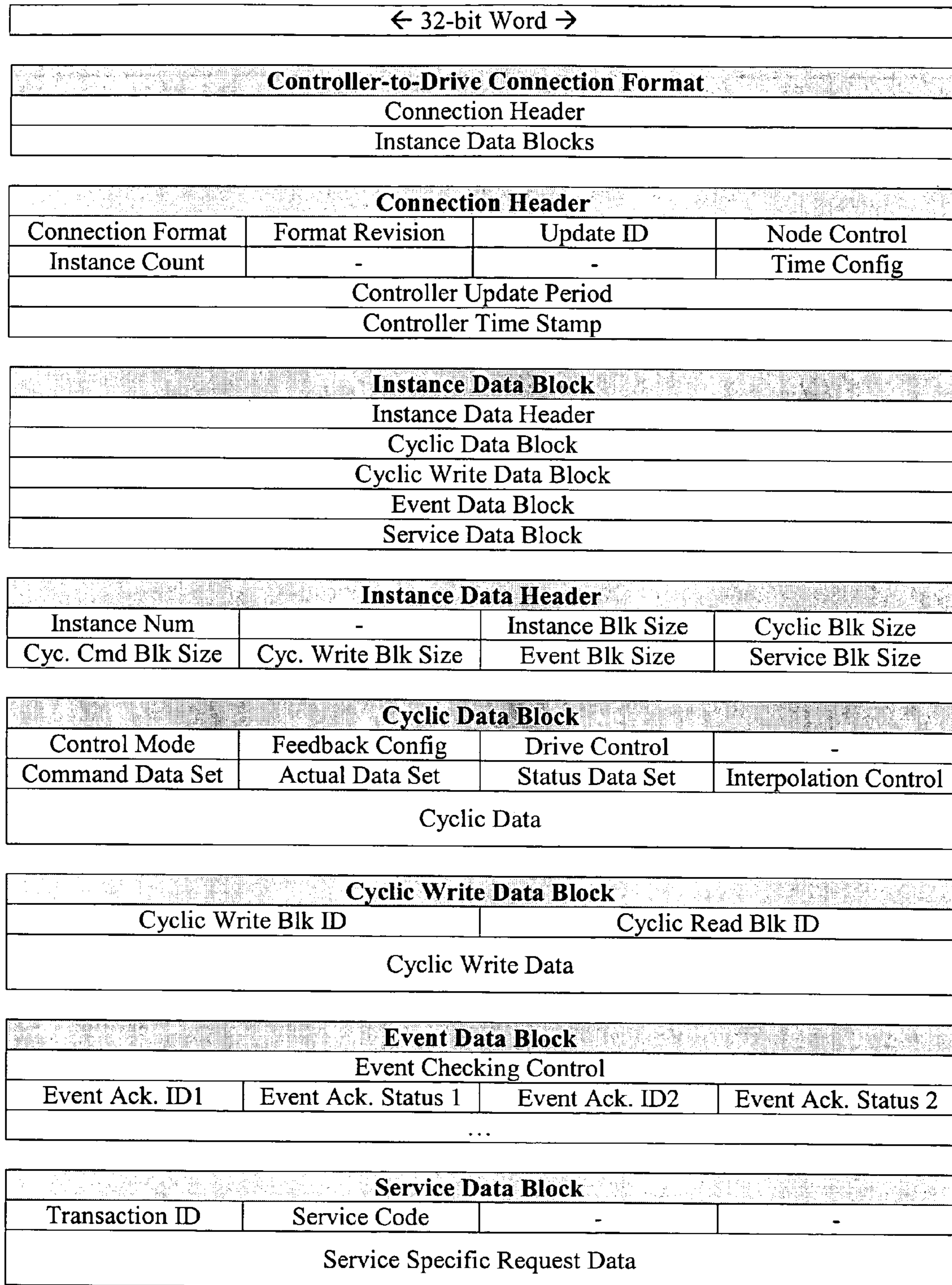
Figure 1-1 — Controller-to-Drive Connection Format
