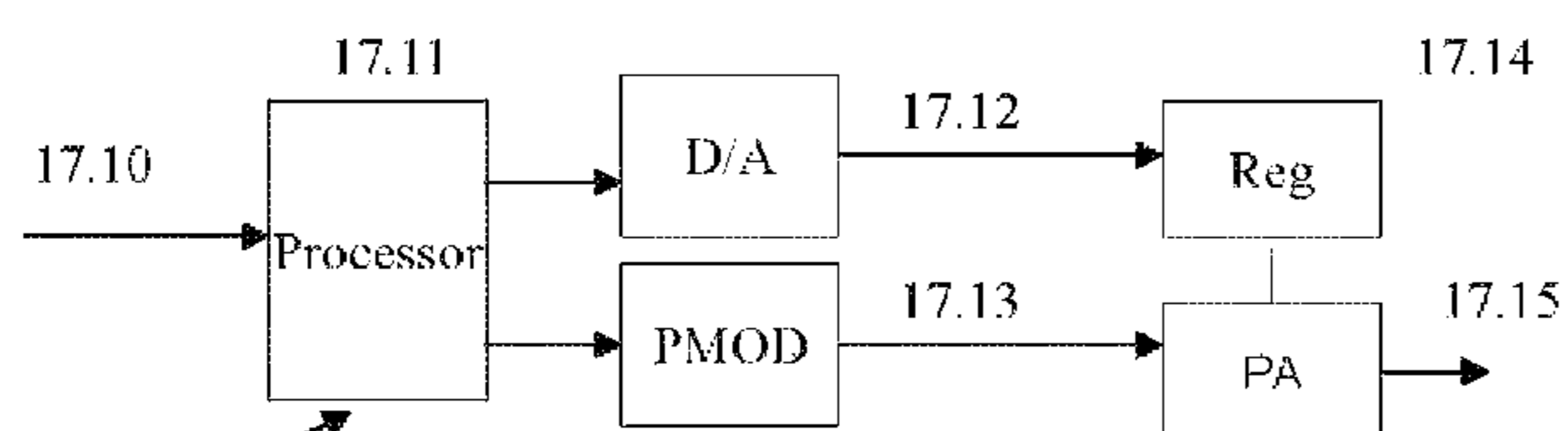
Fig. 17b A prior art Non Quadrature -Polar Modulator
