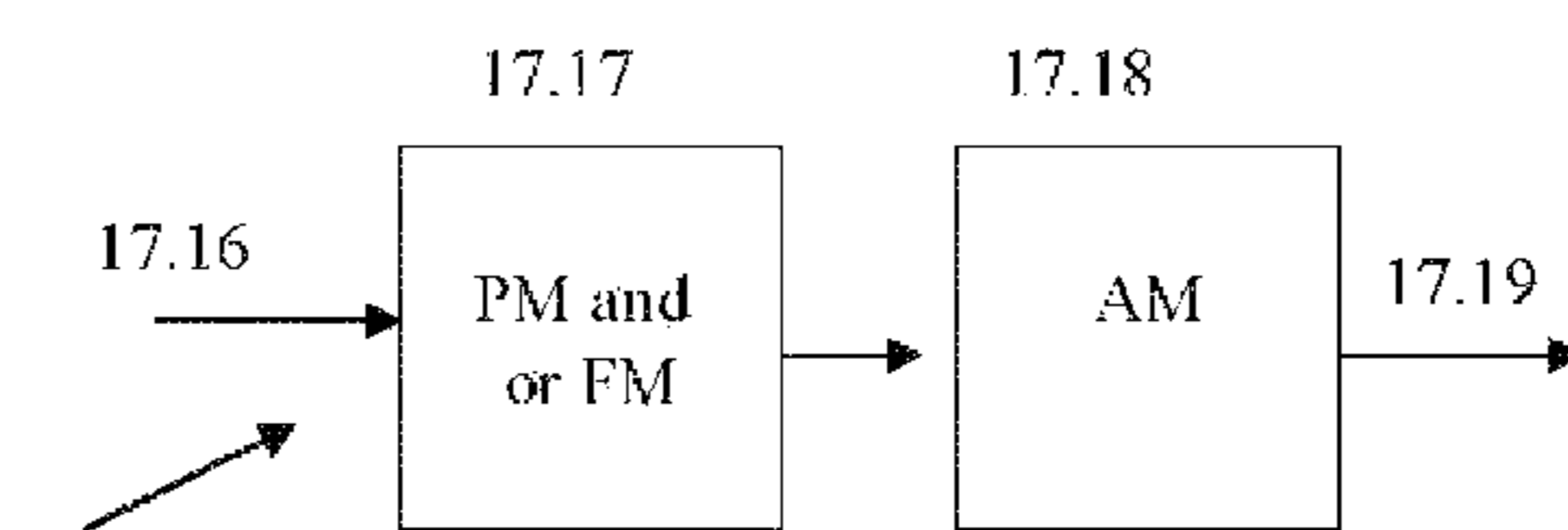
Fig. 17c An other prior art Non Quadrature Modulator
