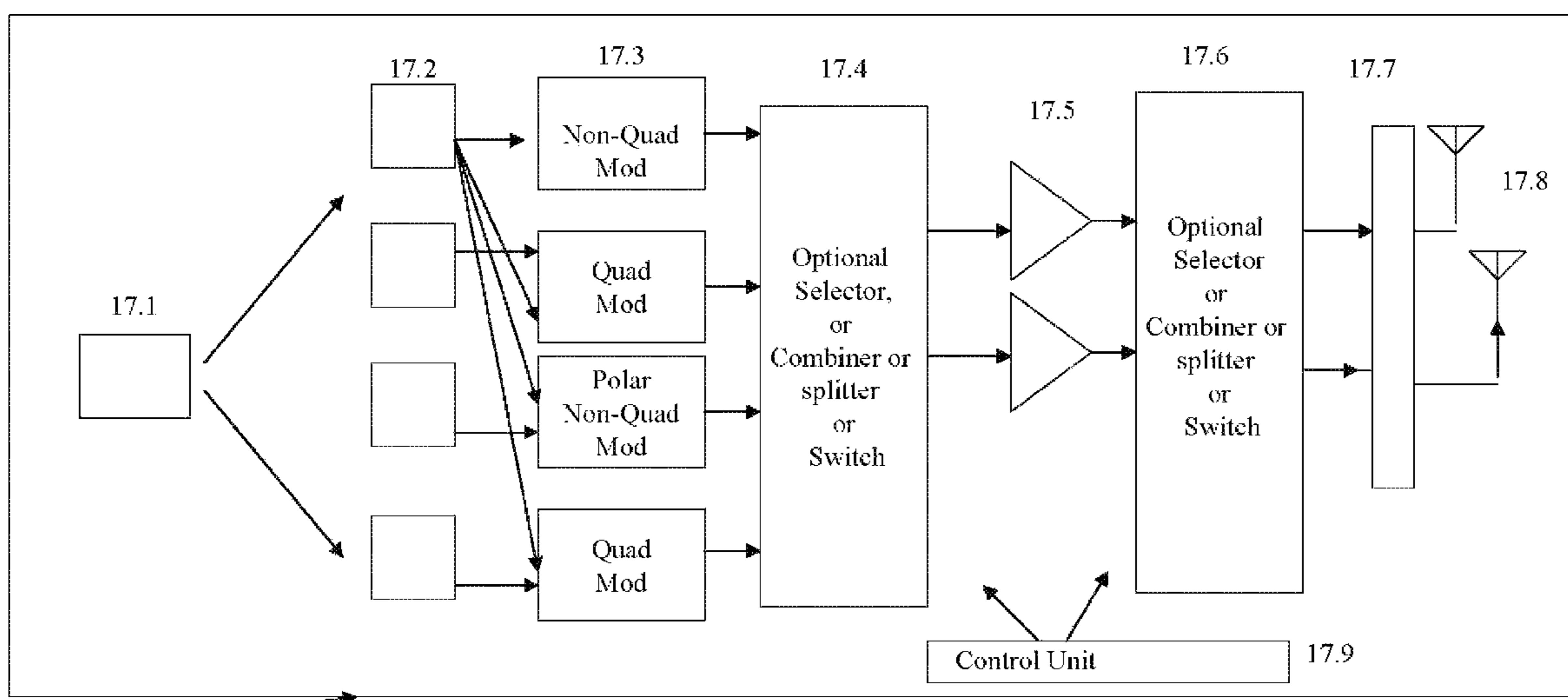
Fig. 17a Multi-mode quad and non-Quad modulators , including polar modulators
