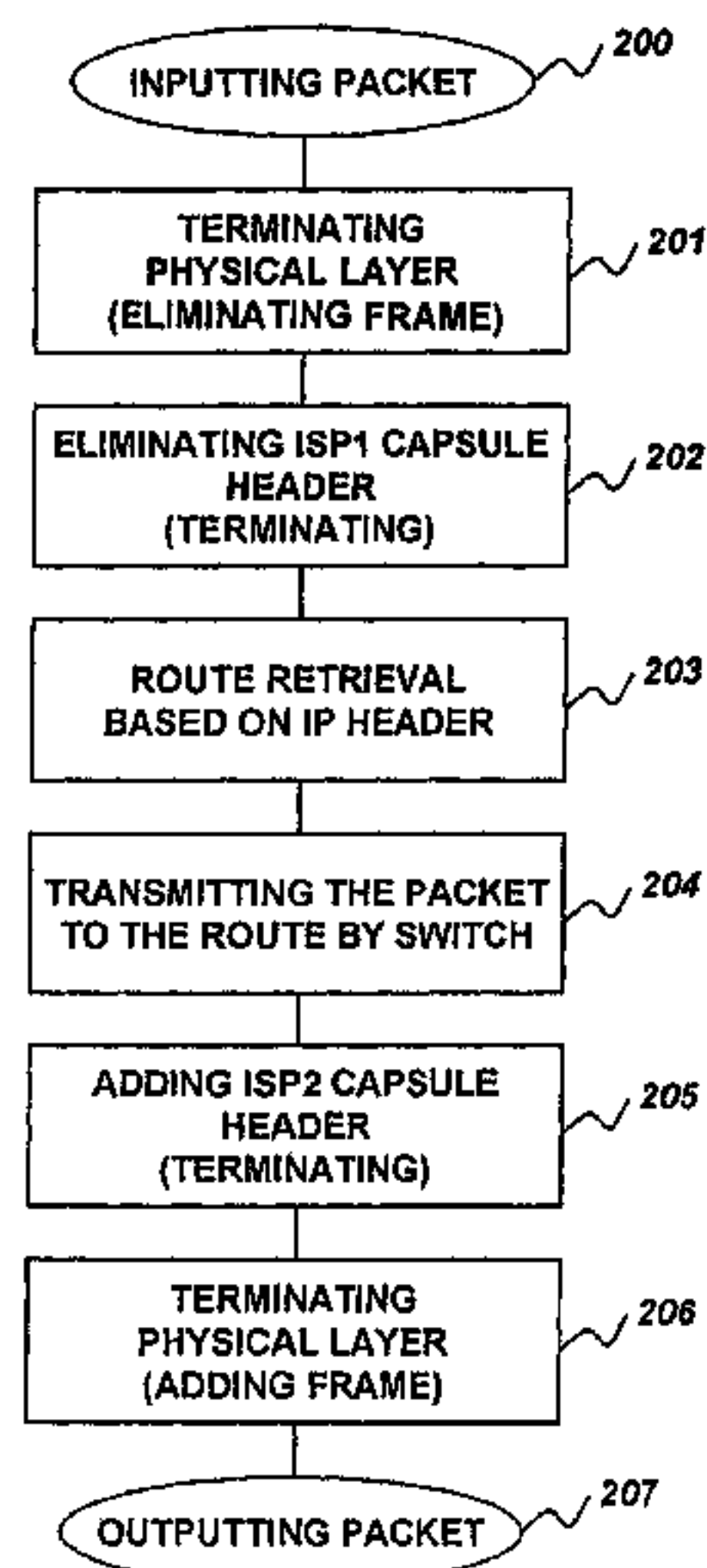
PROCESSING FLOW IN ROUTER
