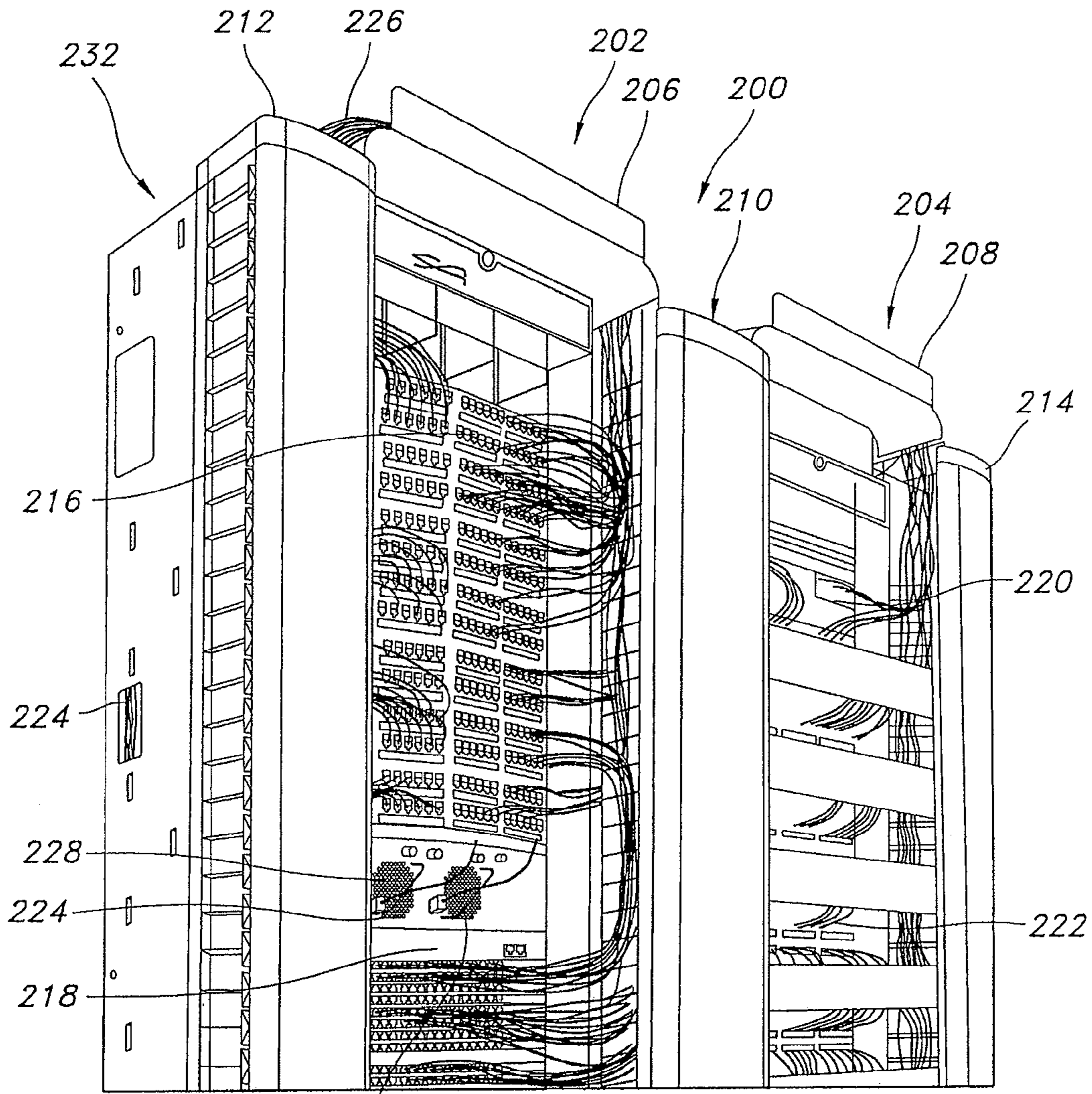
FIG. 2 (Prior Art)
