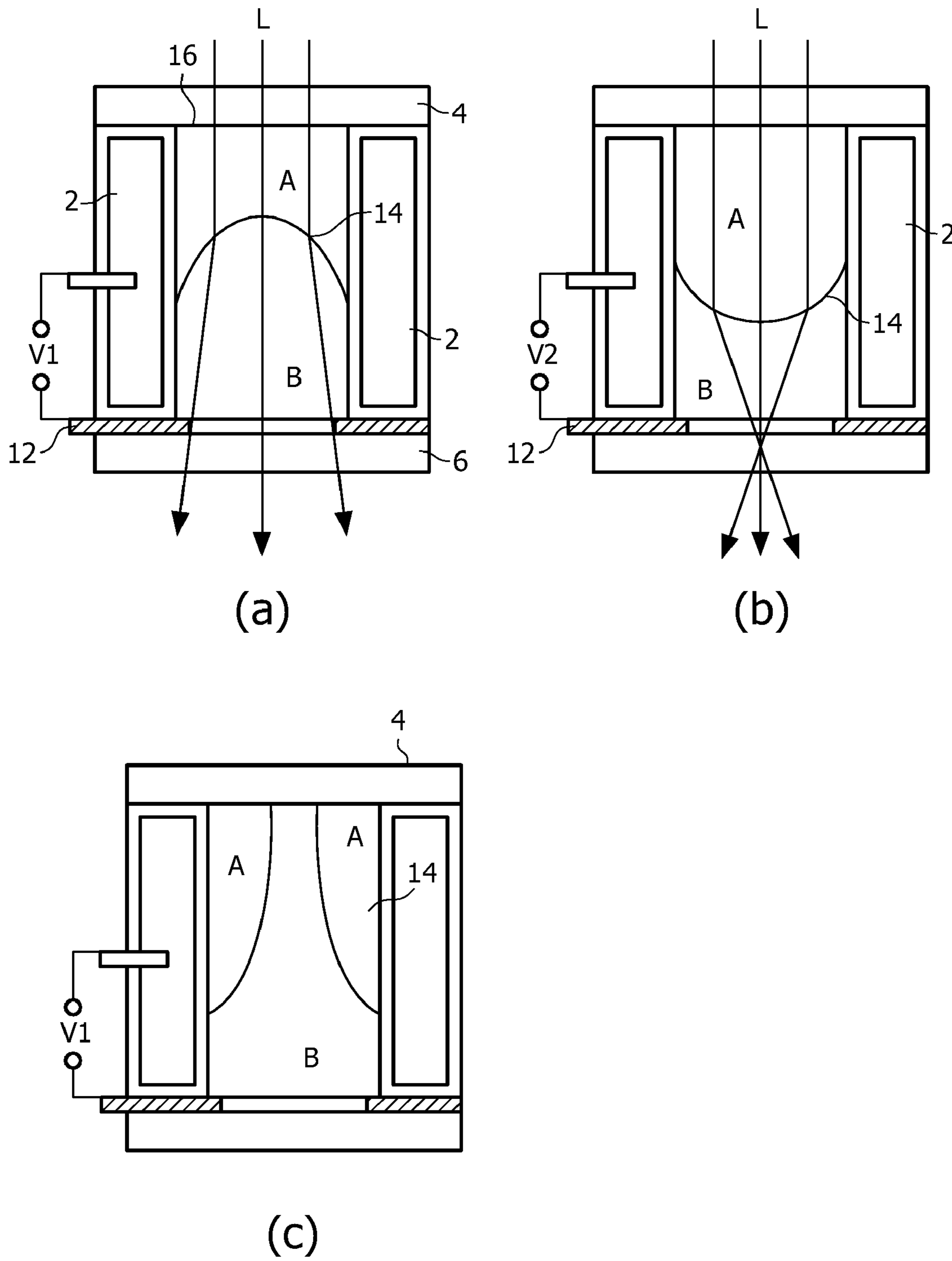
FIG. 1 (prior art)
