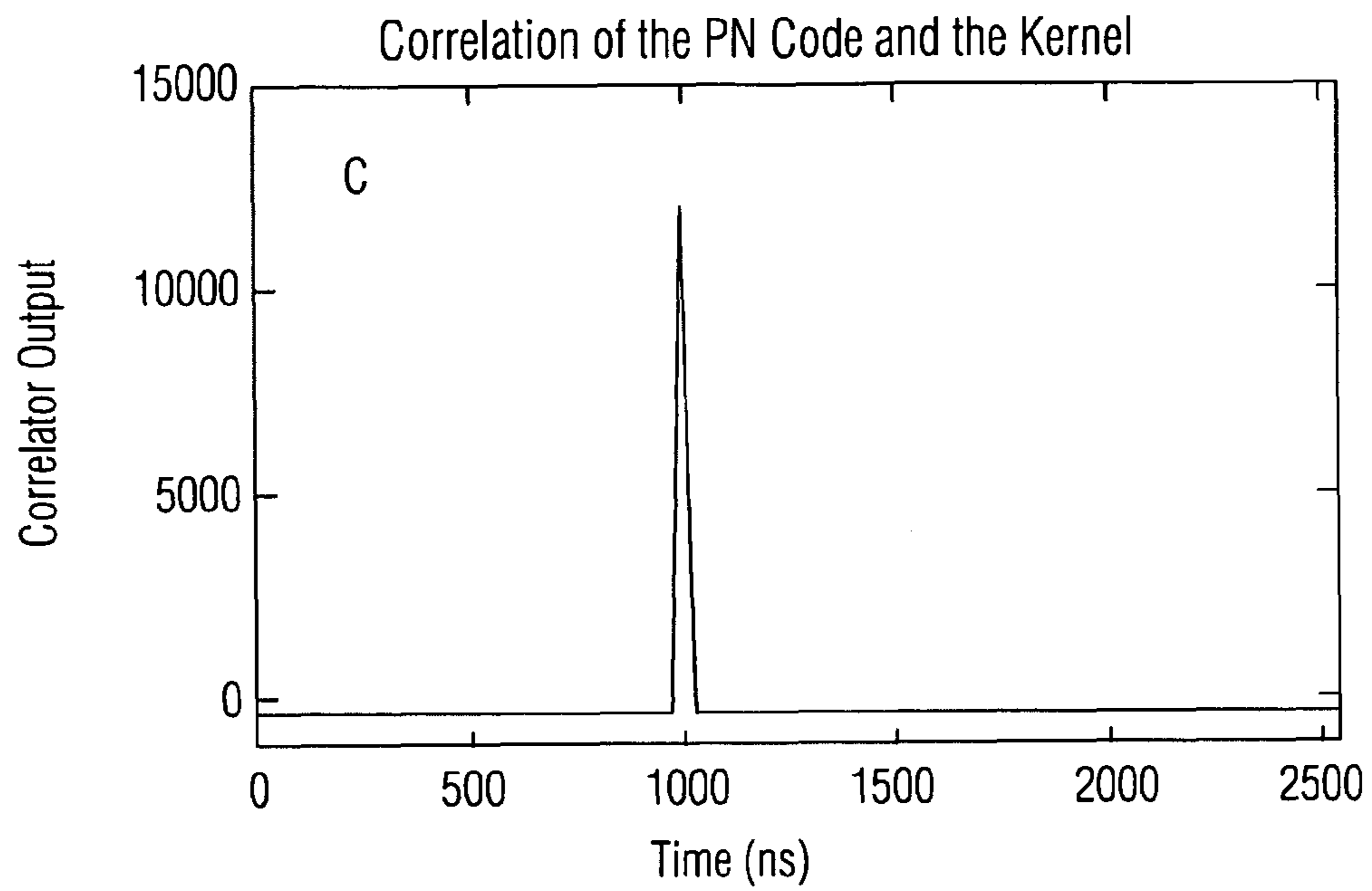
PRIOR ART Fig. 2C
