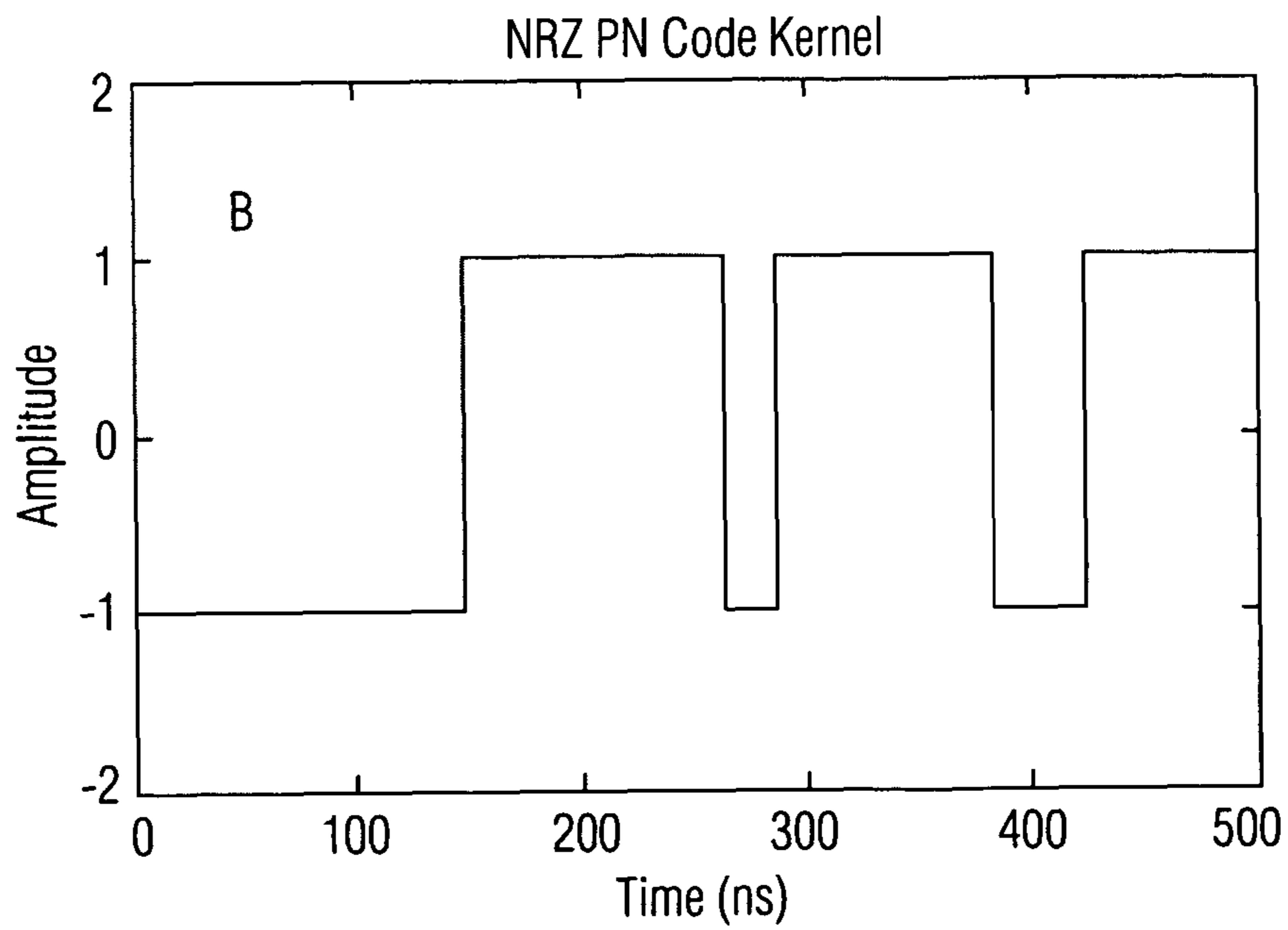
PRIOR ART Fig. 2F
