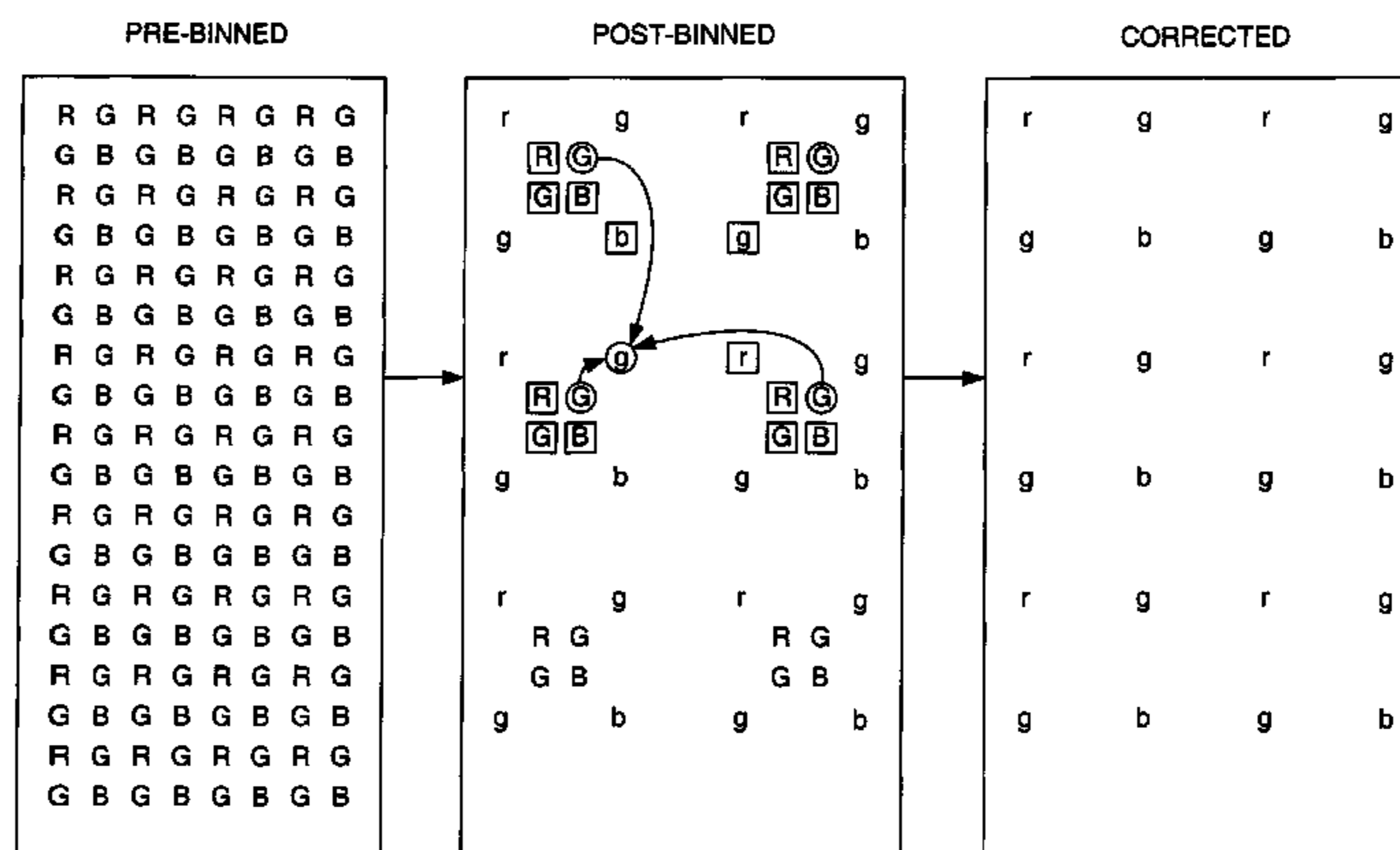
POSITION CORRECTION OF PIXELS AFTER 2X HORIZONTAL AND 2X VERTICAL BINNING
