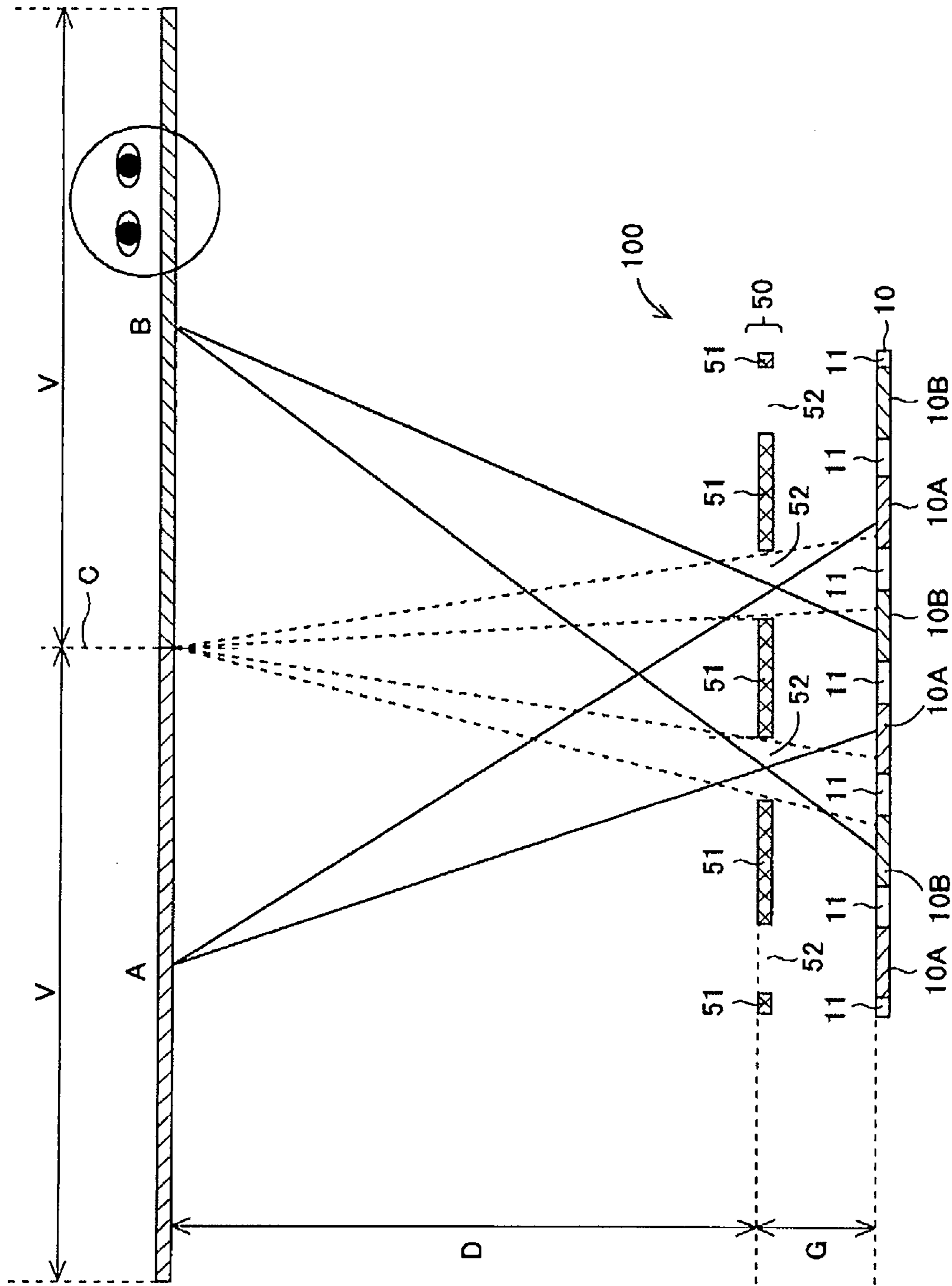
FIG. 12 PRIOR ART
