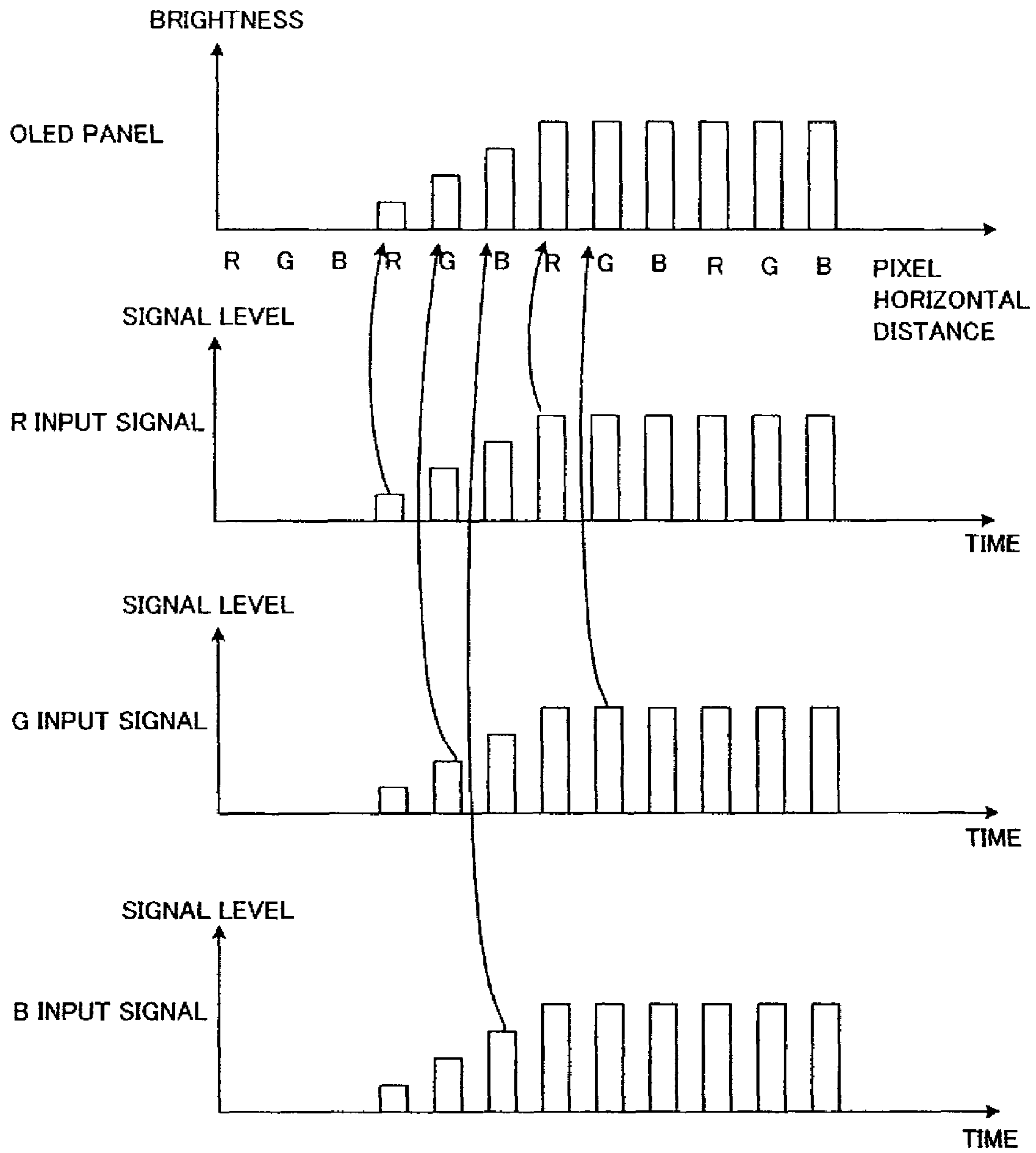
Fig. 5 (PRIOR ART)
