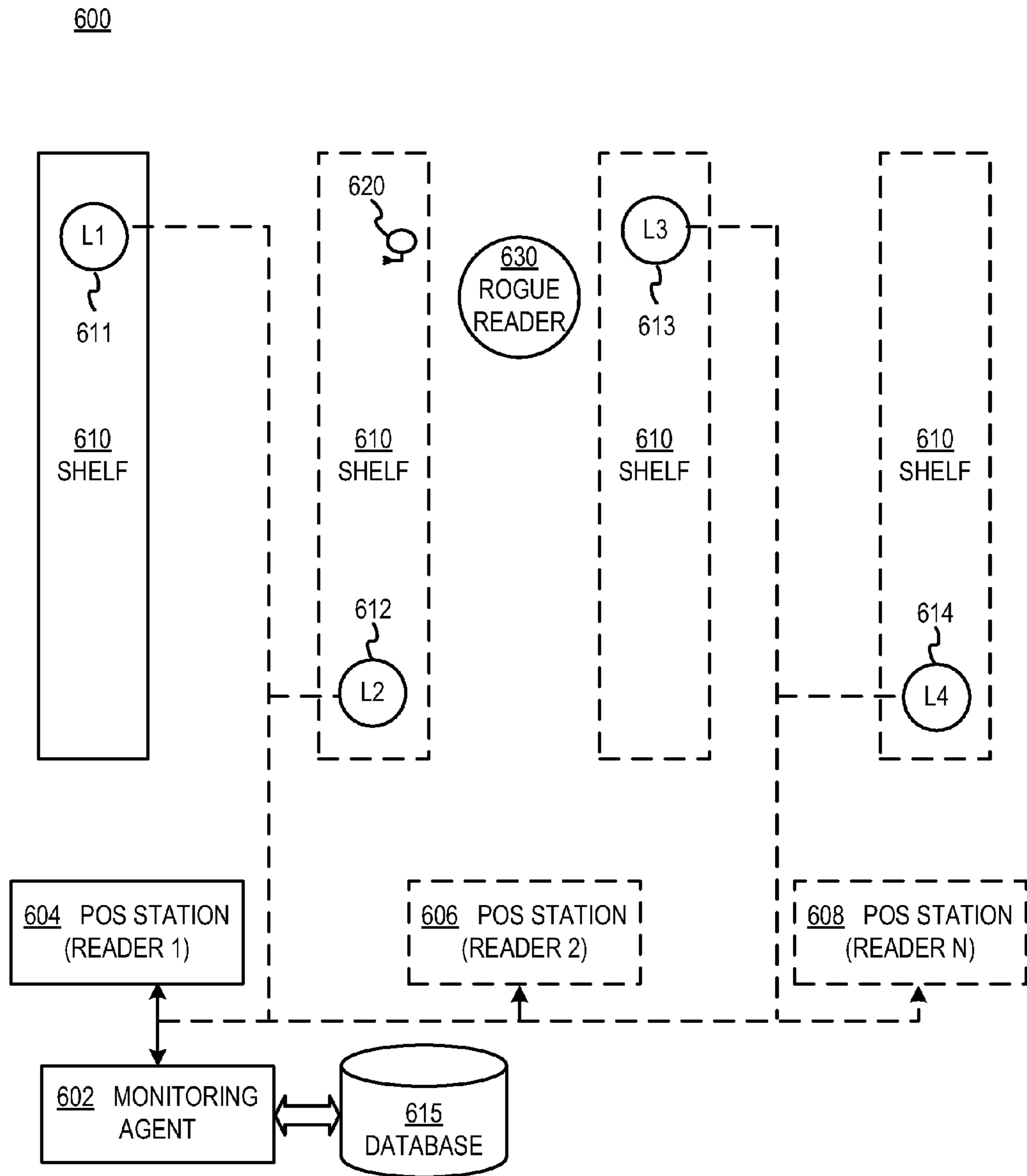
EXEMPLARY SYSTEM SETUP FOR ROGUE READER DETECTION
