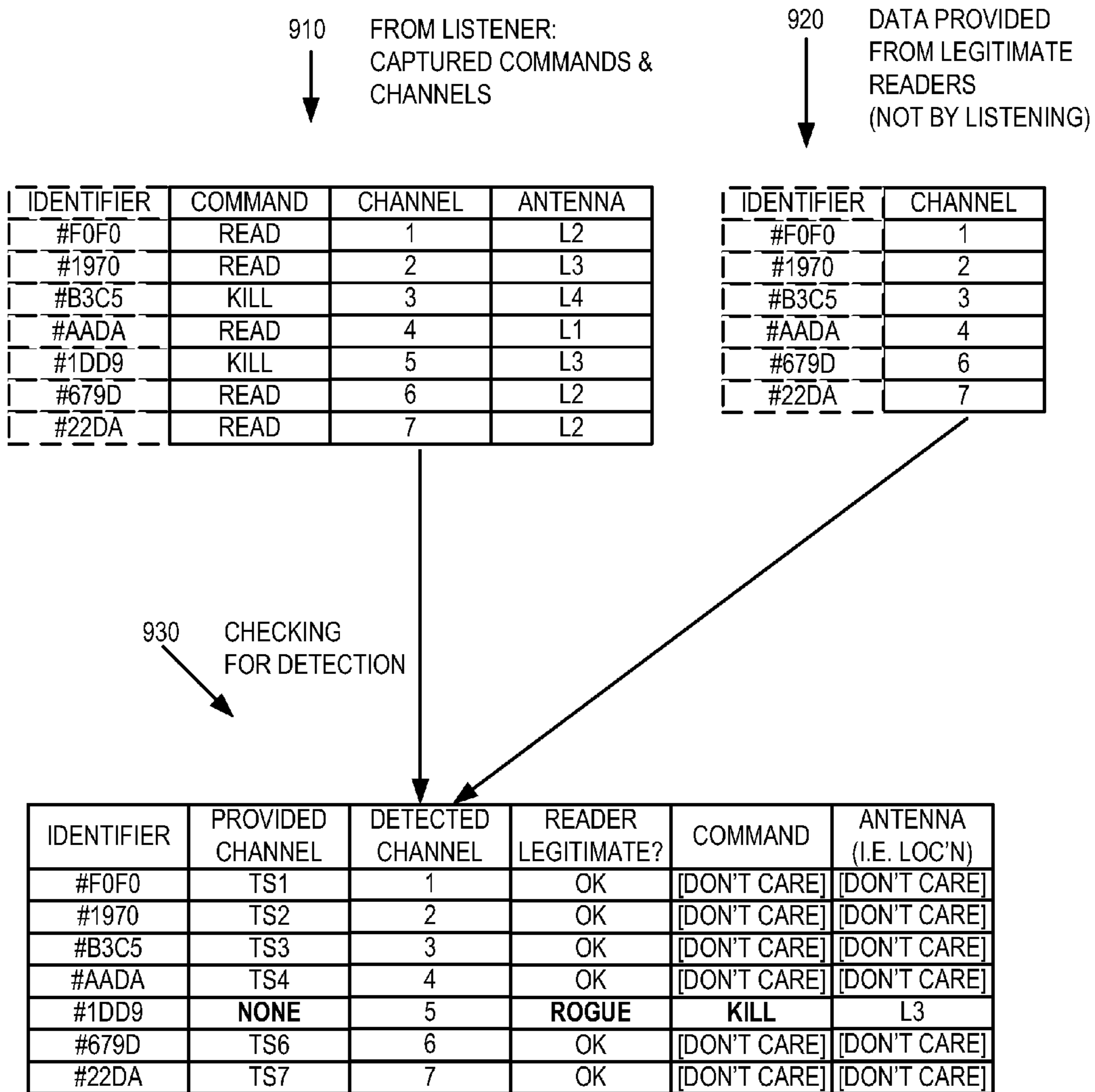
EXAMPLE OF ROGUE READER DETECTION USING CHANNELS
