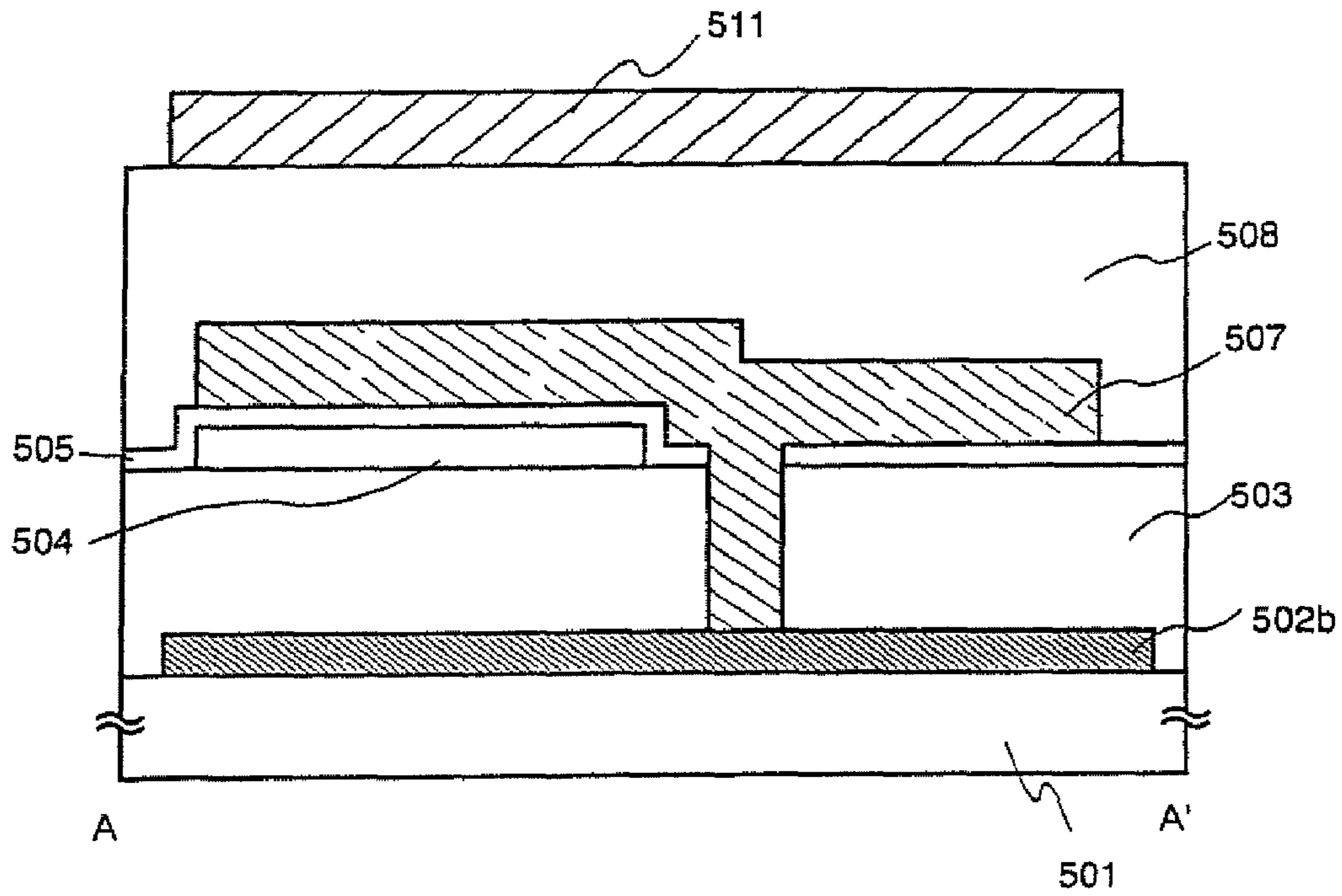
Fig. 15A A-A' Cross sectional view
