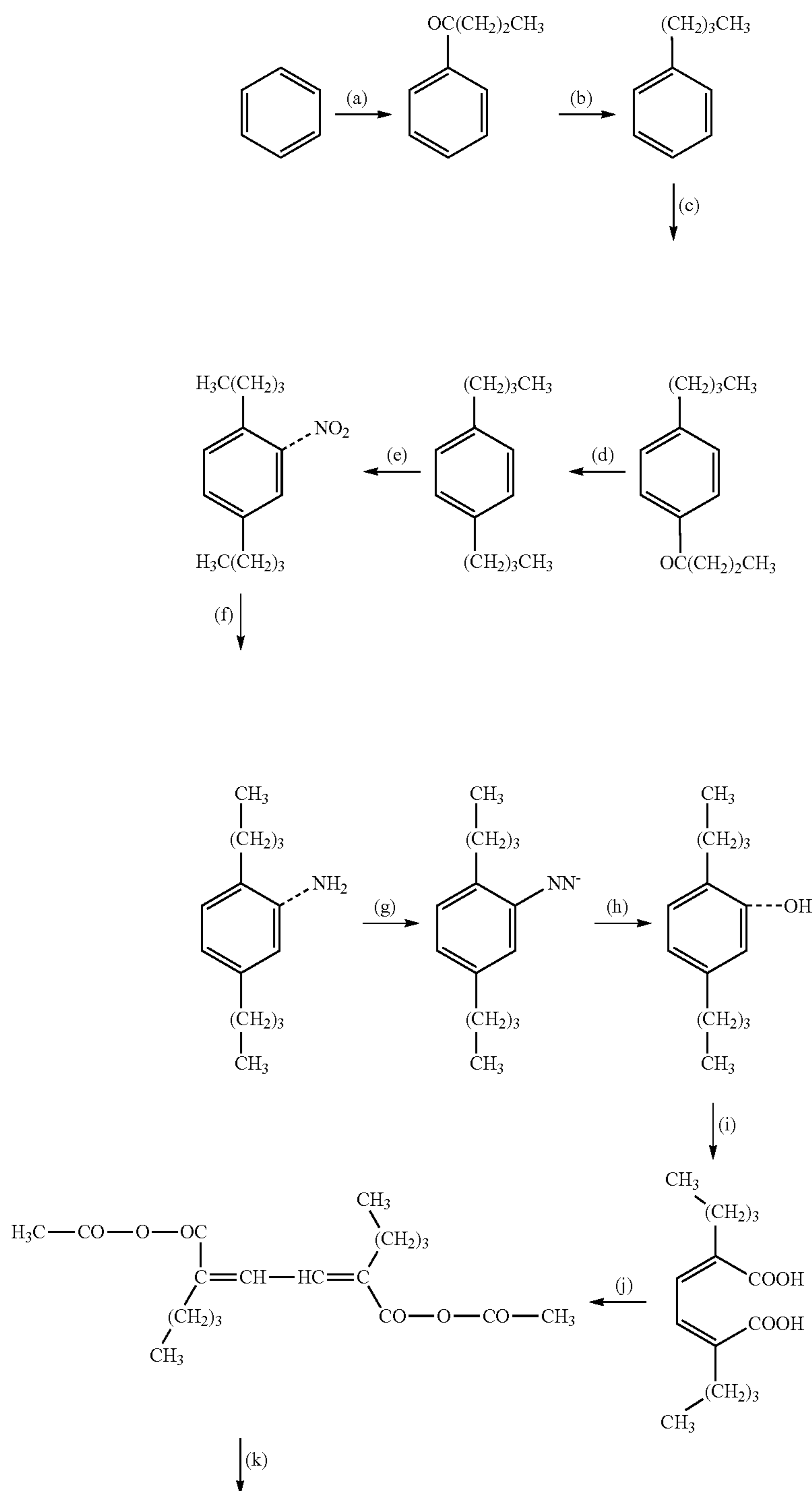
Scheme One
