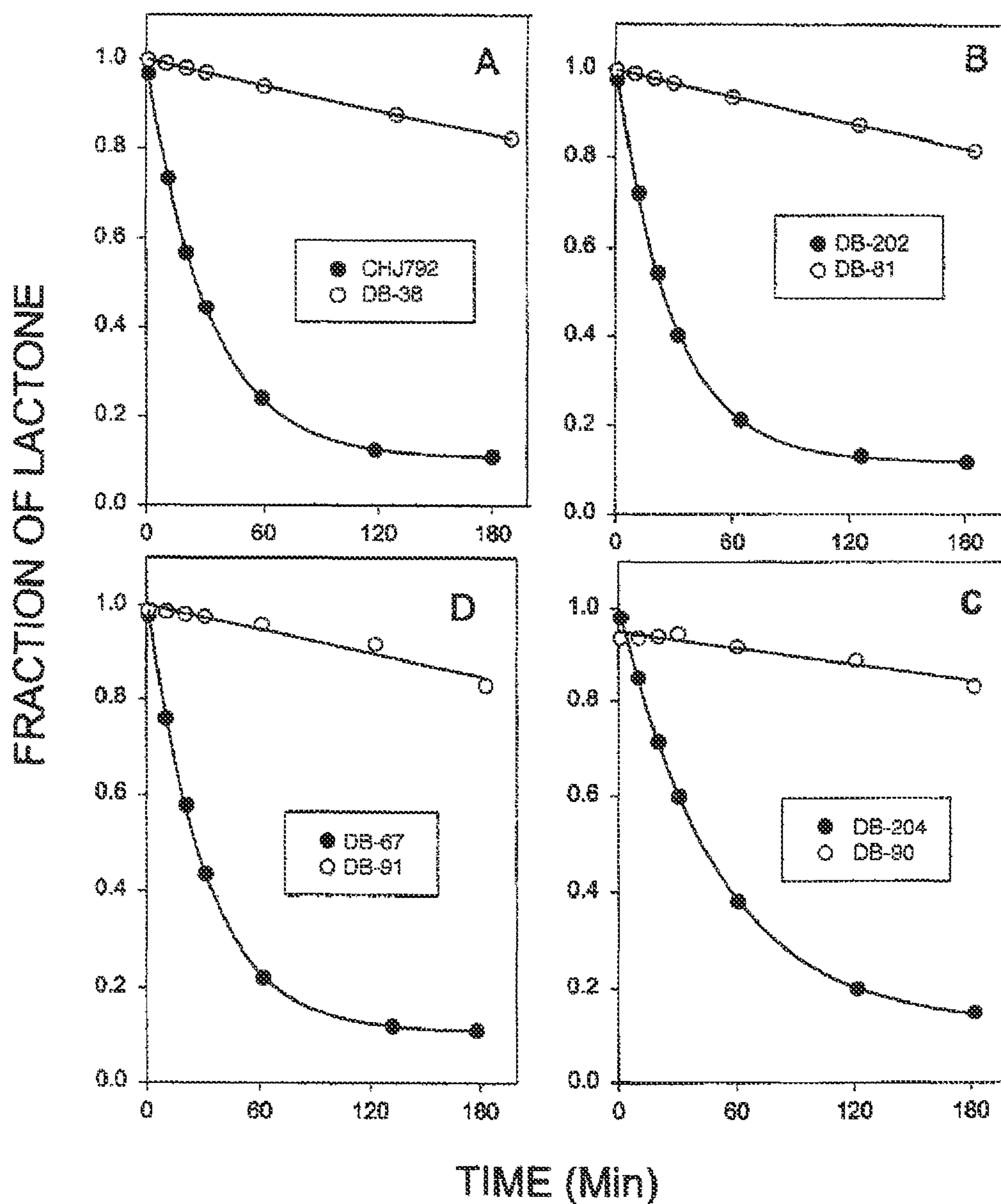
Comparison of the Stabilities of \alpha -Lactone Silatecans with their corresponding Homosilatecans in PBS Buffer at 37°C
