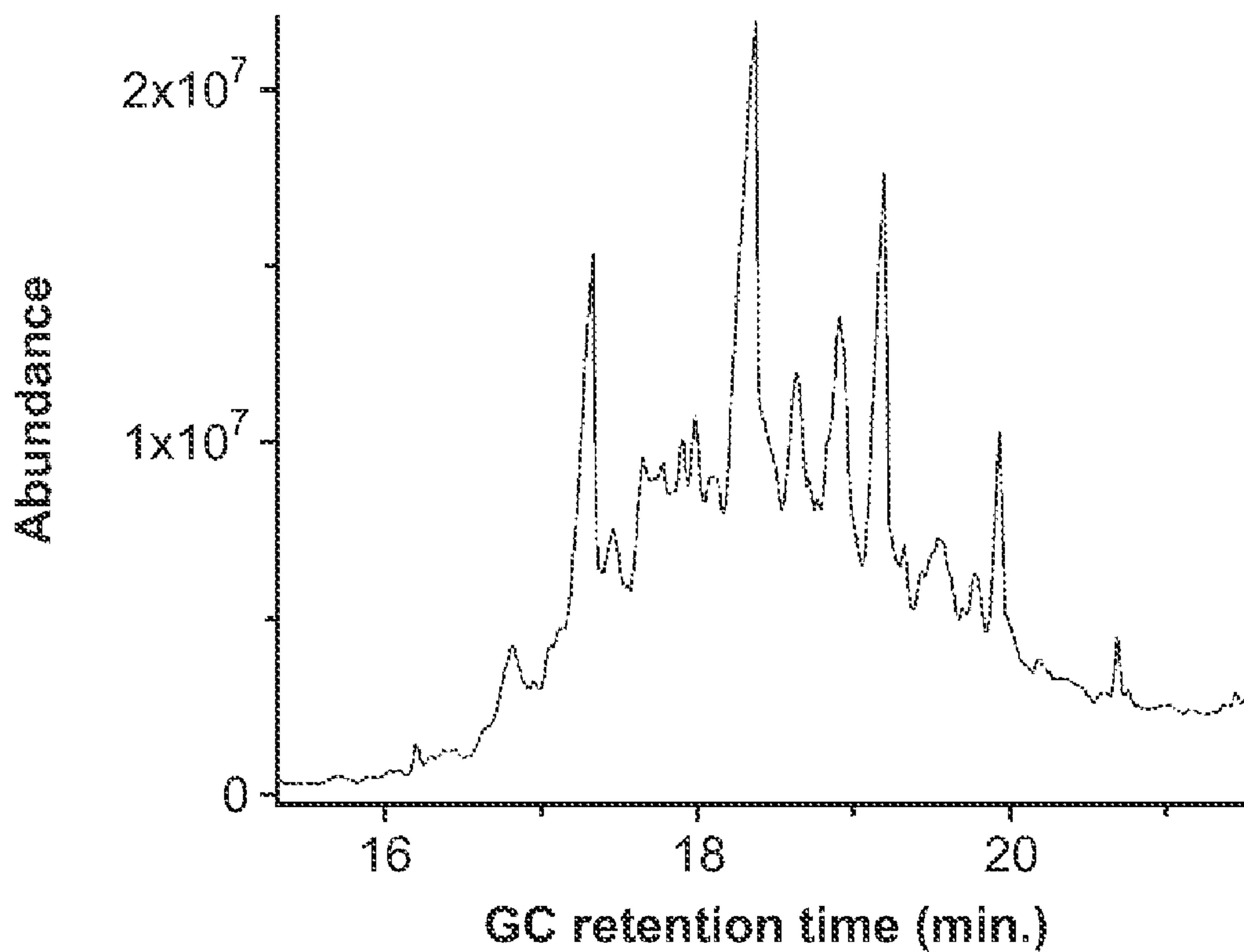
TIC of the aza tetramantanes contained mixture
