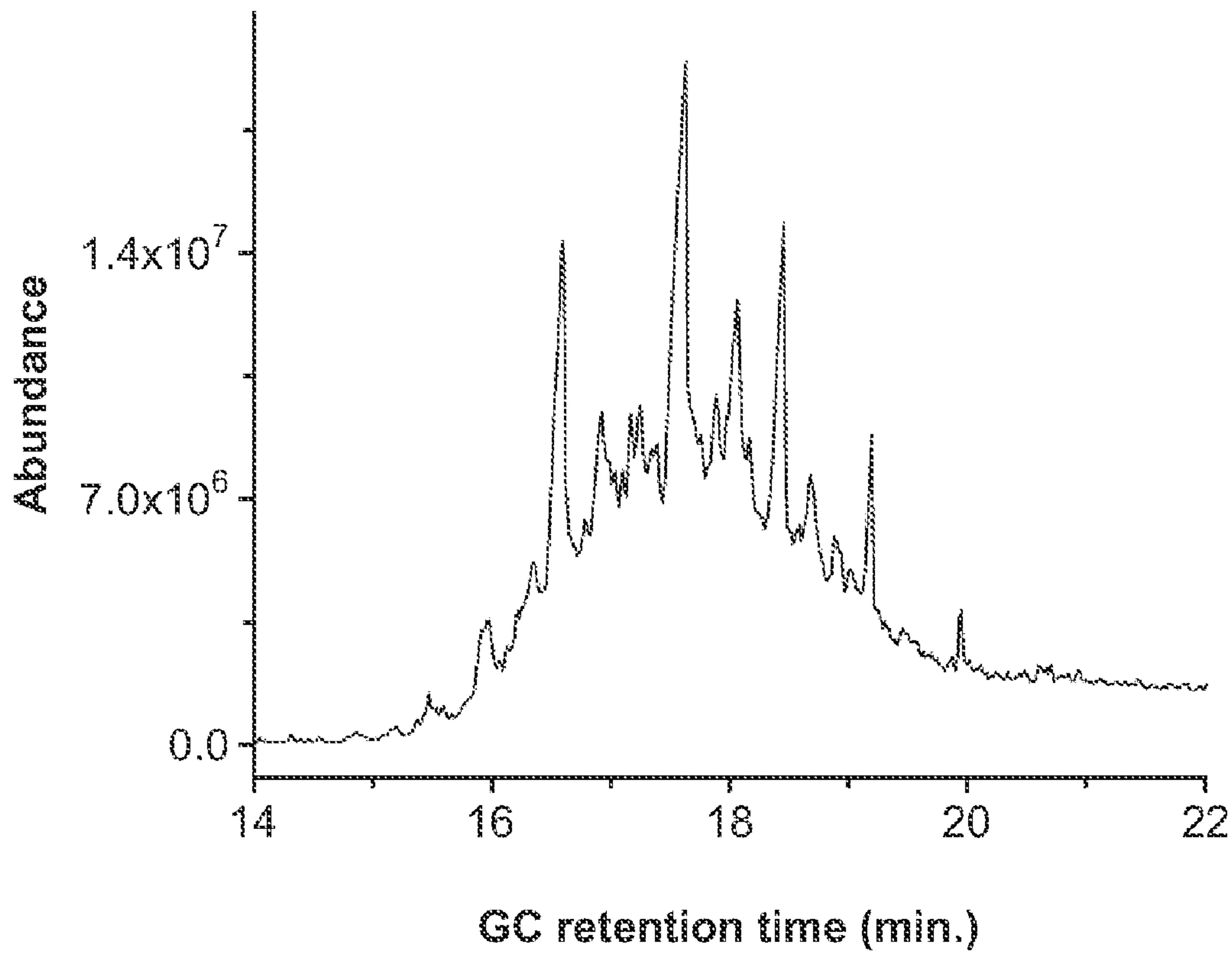
TIC of the N-formyl aza tetramantanes contained mixture
