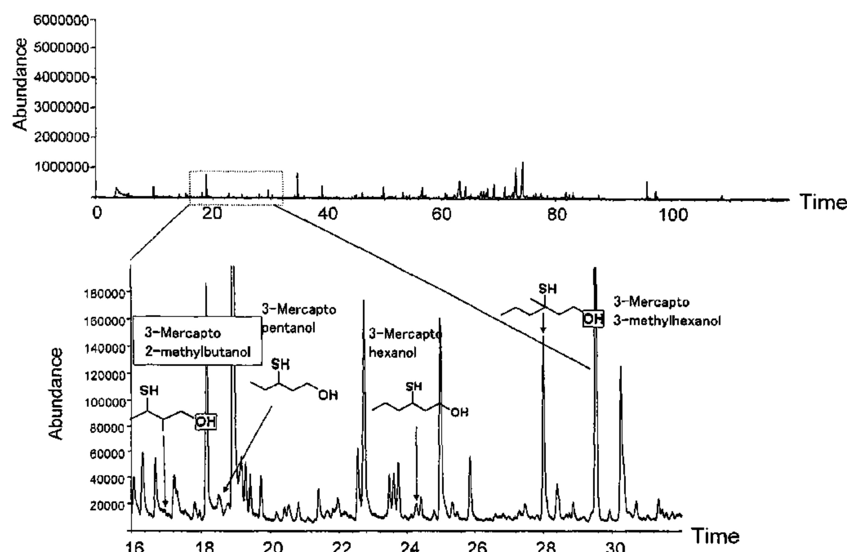
Total ion chromatogram of volatile components in incubated perspiration of a person having an apocrine odor
