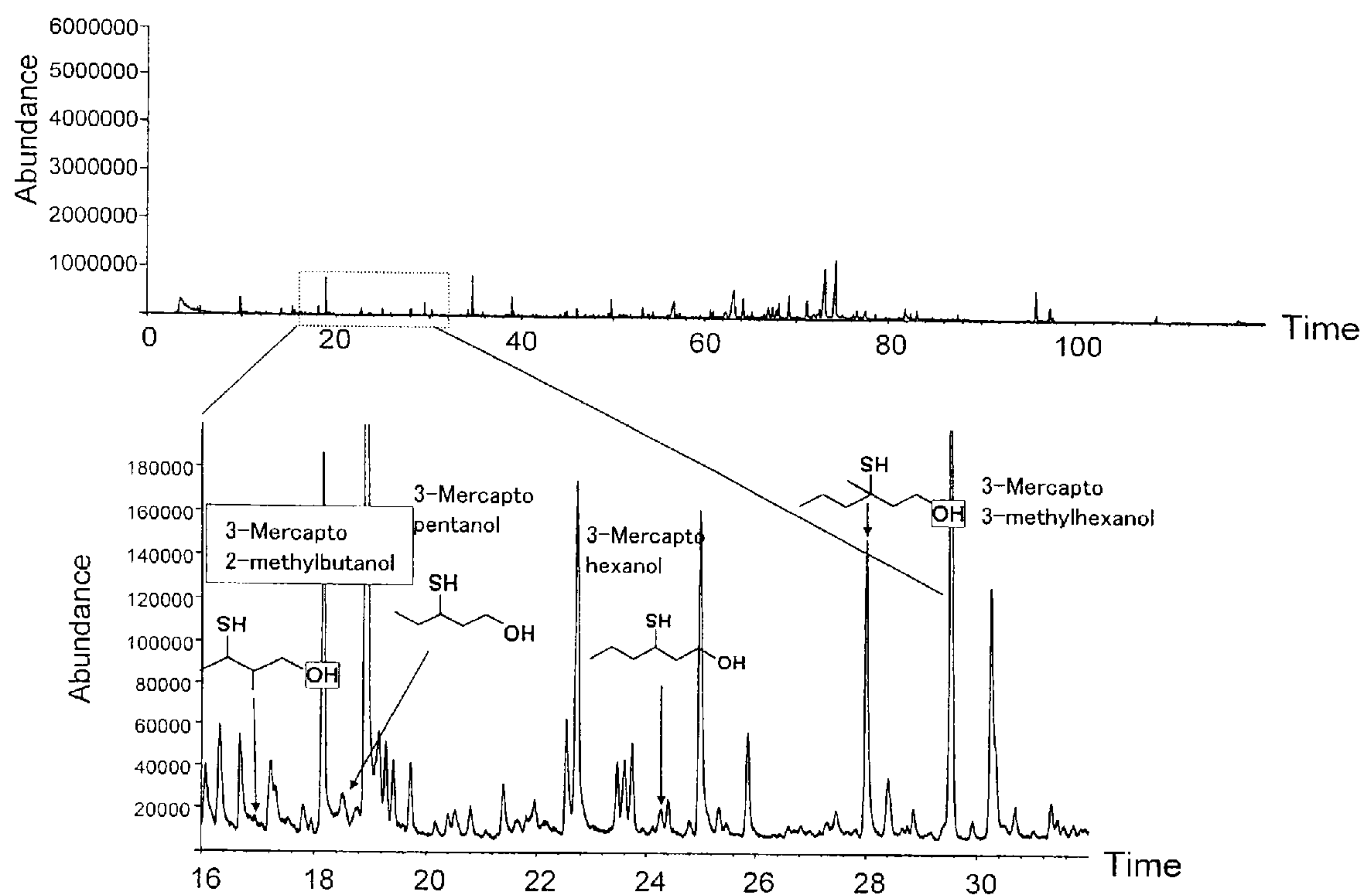
Total ion chromatogram of volatile components in incubated perspiration of a person having an apocrine odor
