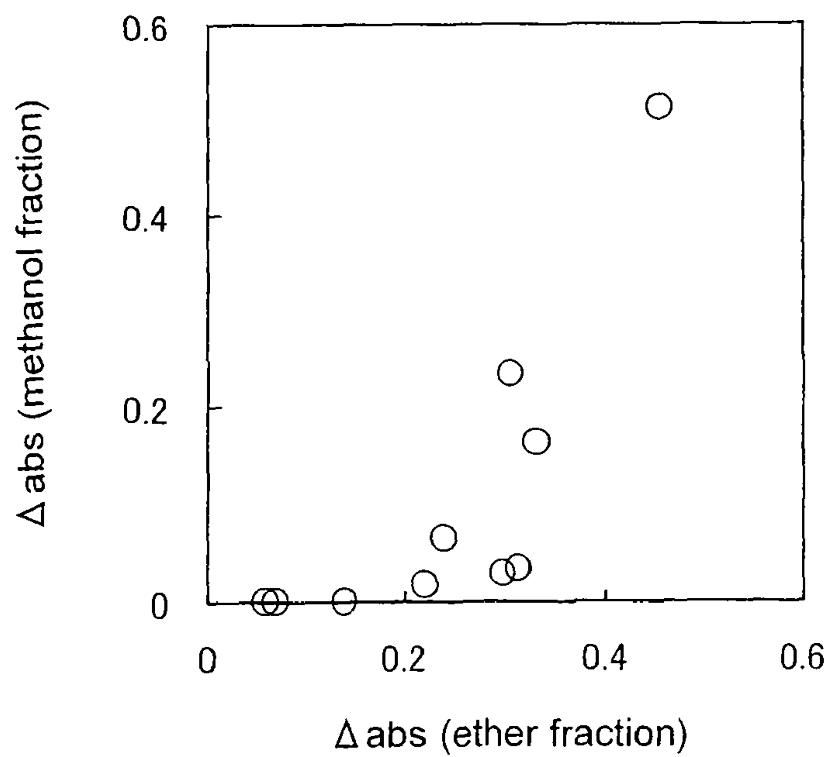
Absorbance of methanol fraction and ether fraction
