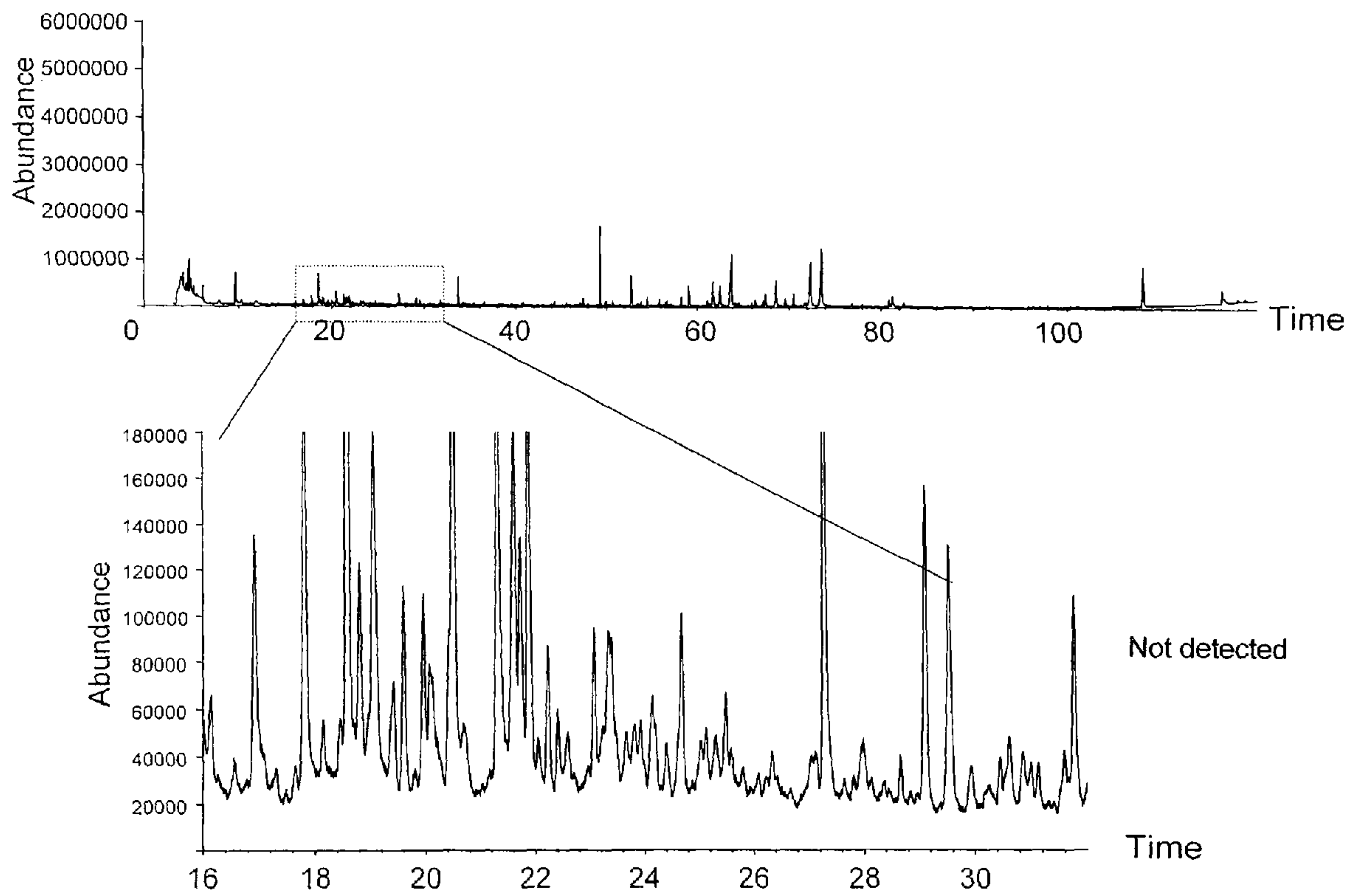
Total ion chromatogram of volatile components in perspiration of a person having no apocrine odor
