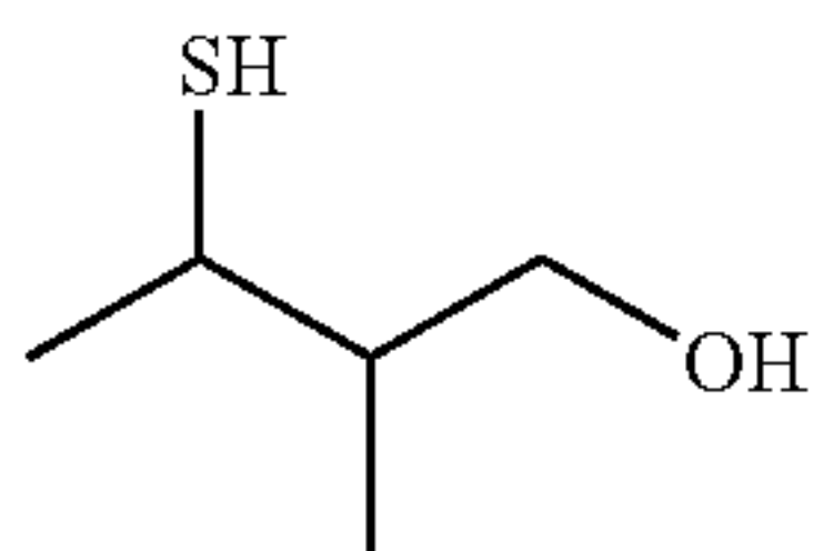
3-mercapto-2-methylbutanol
