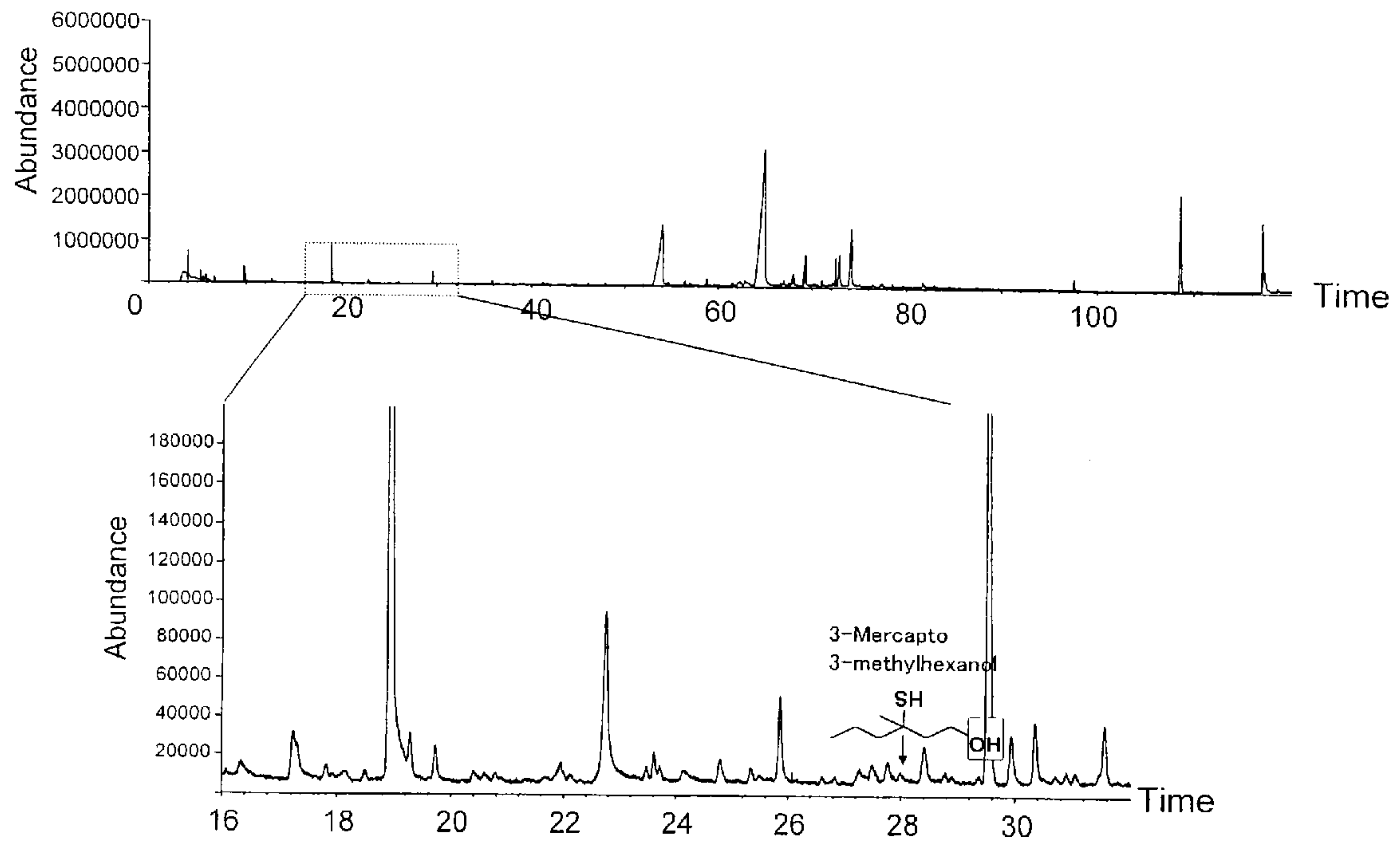
Total ion chromatogram of volatile components in perspiration of a person having an apocrine odor
