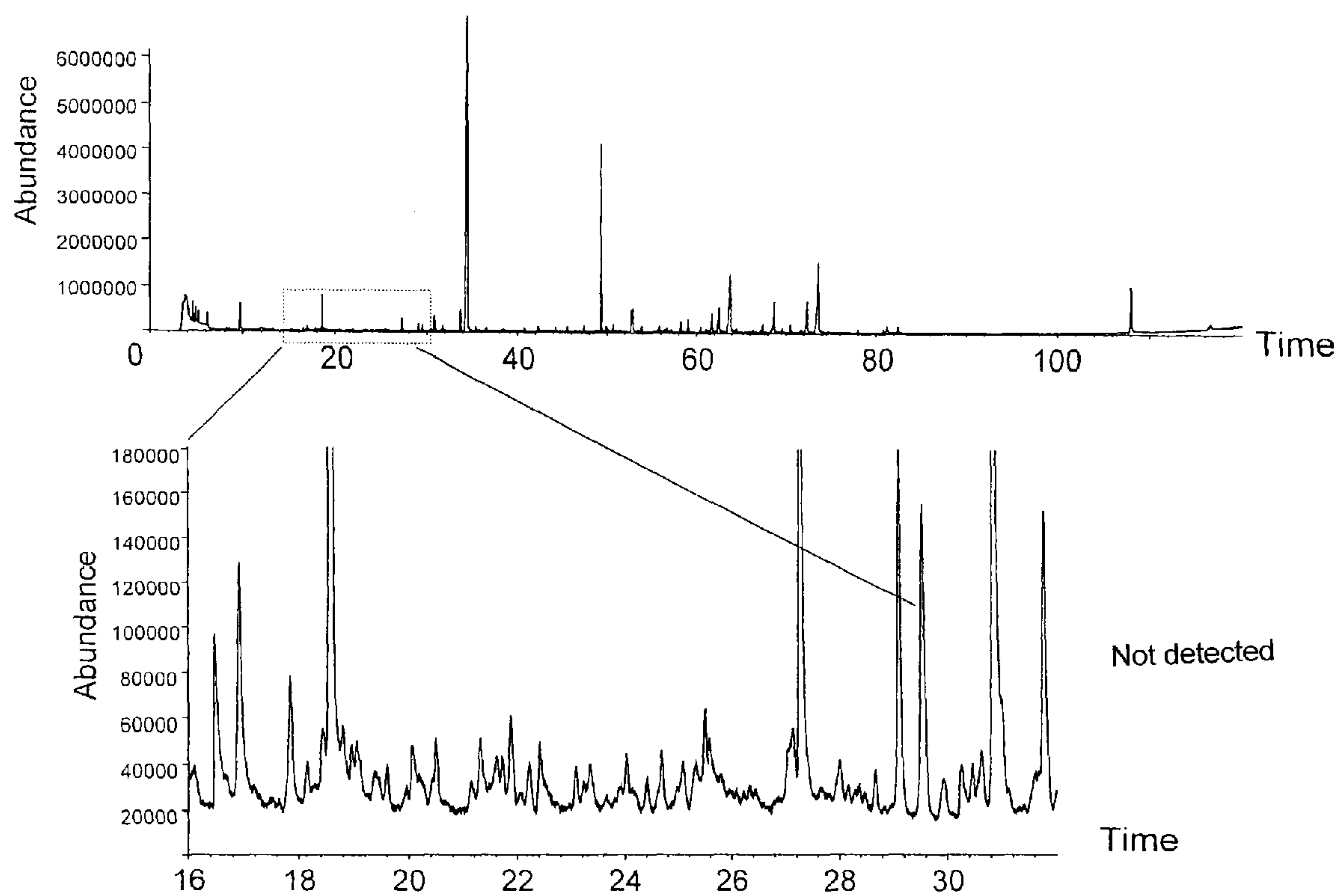
Total ion chromatogram of volatile components in incubated perspiration of a person having no apocrine odor
