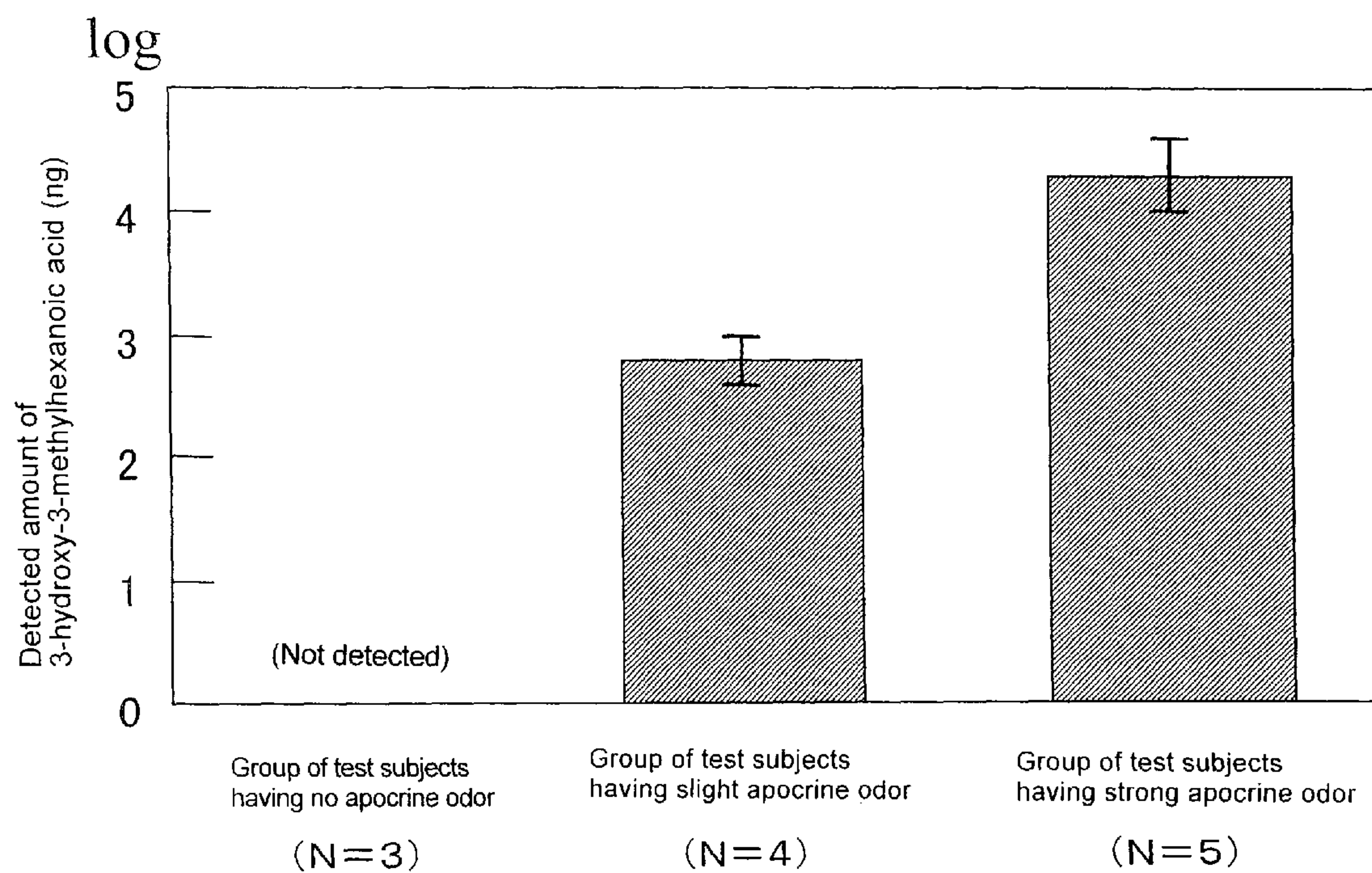
Relationship between 3-hydroxy-3-methylhexanoic acid and an apocrine odor
