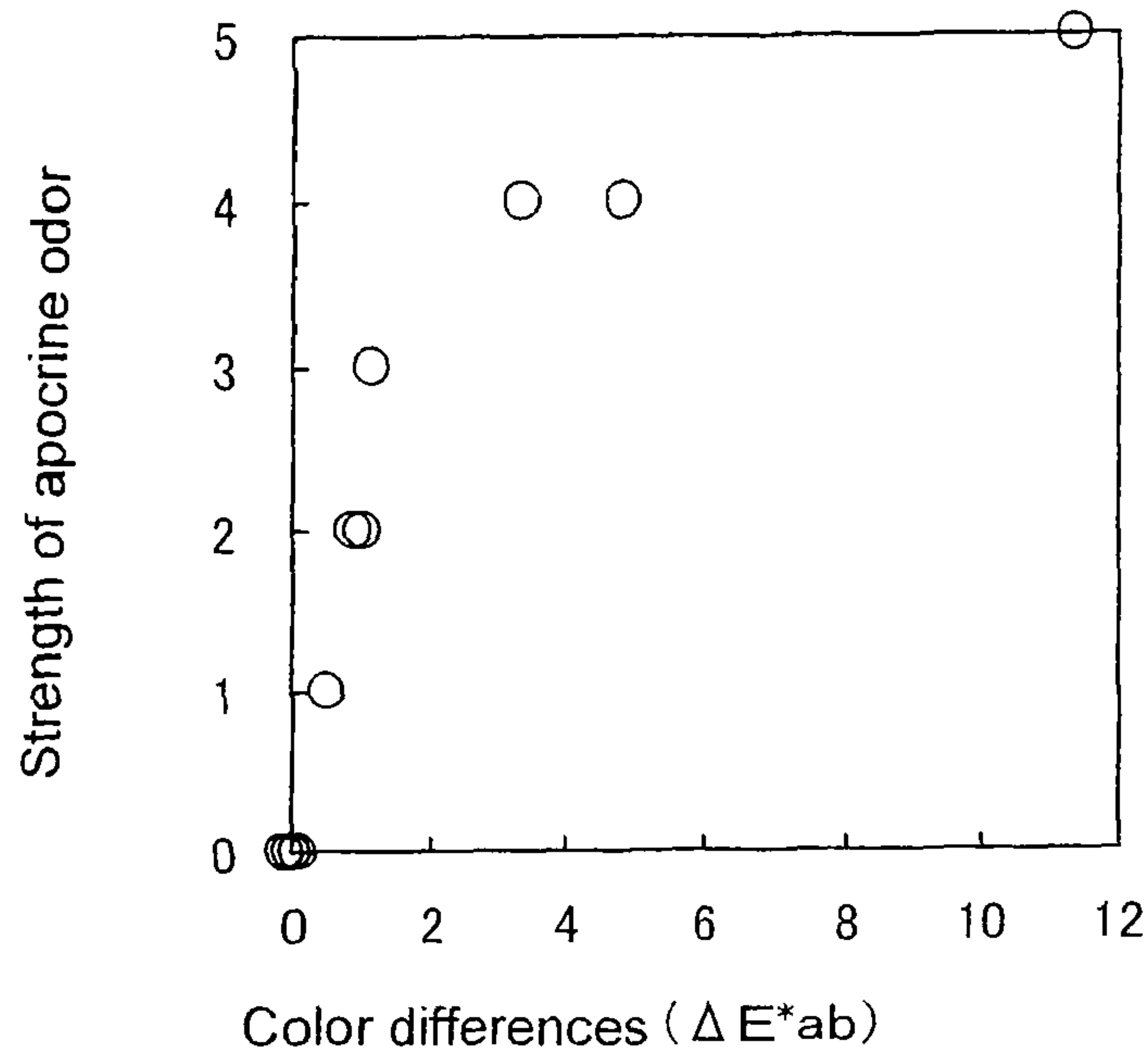
Relationship between strength of apocrine odor and color differences
