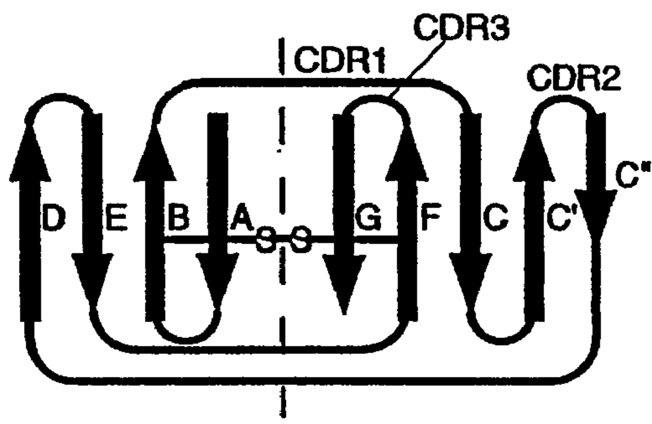
Immunoglobulin VH
