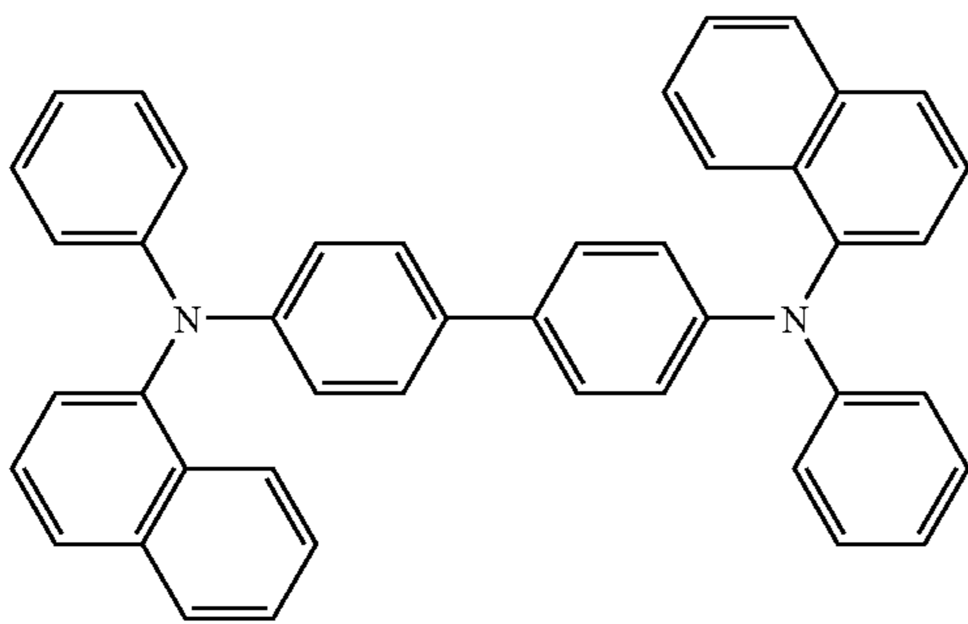
NPD
