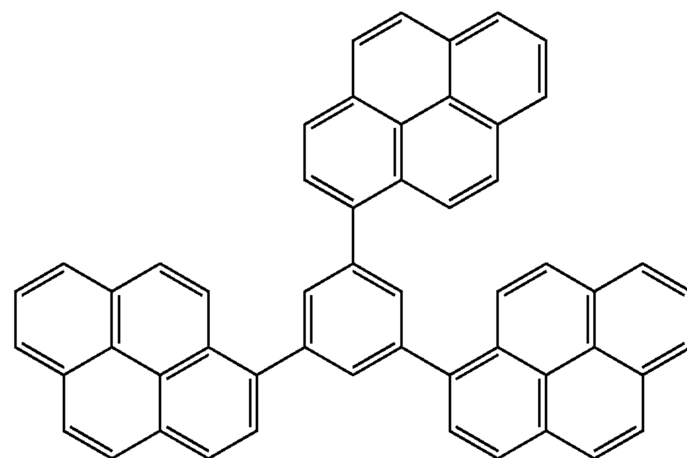
1,3,5-TPB
