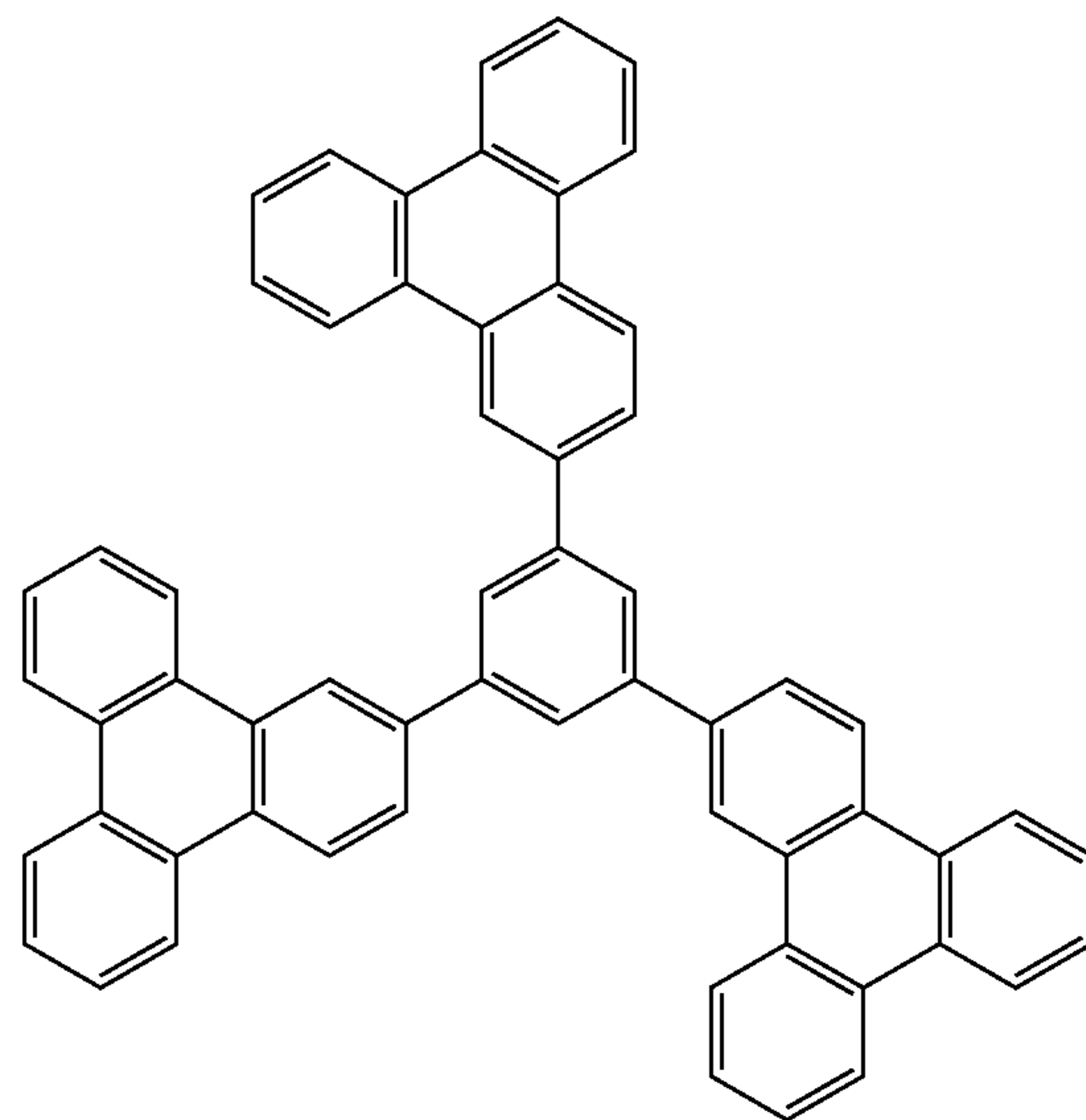
1,3,5-TTB
