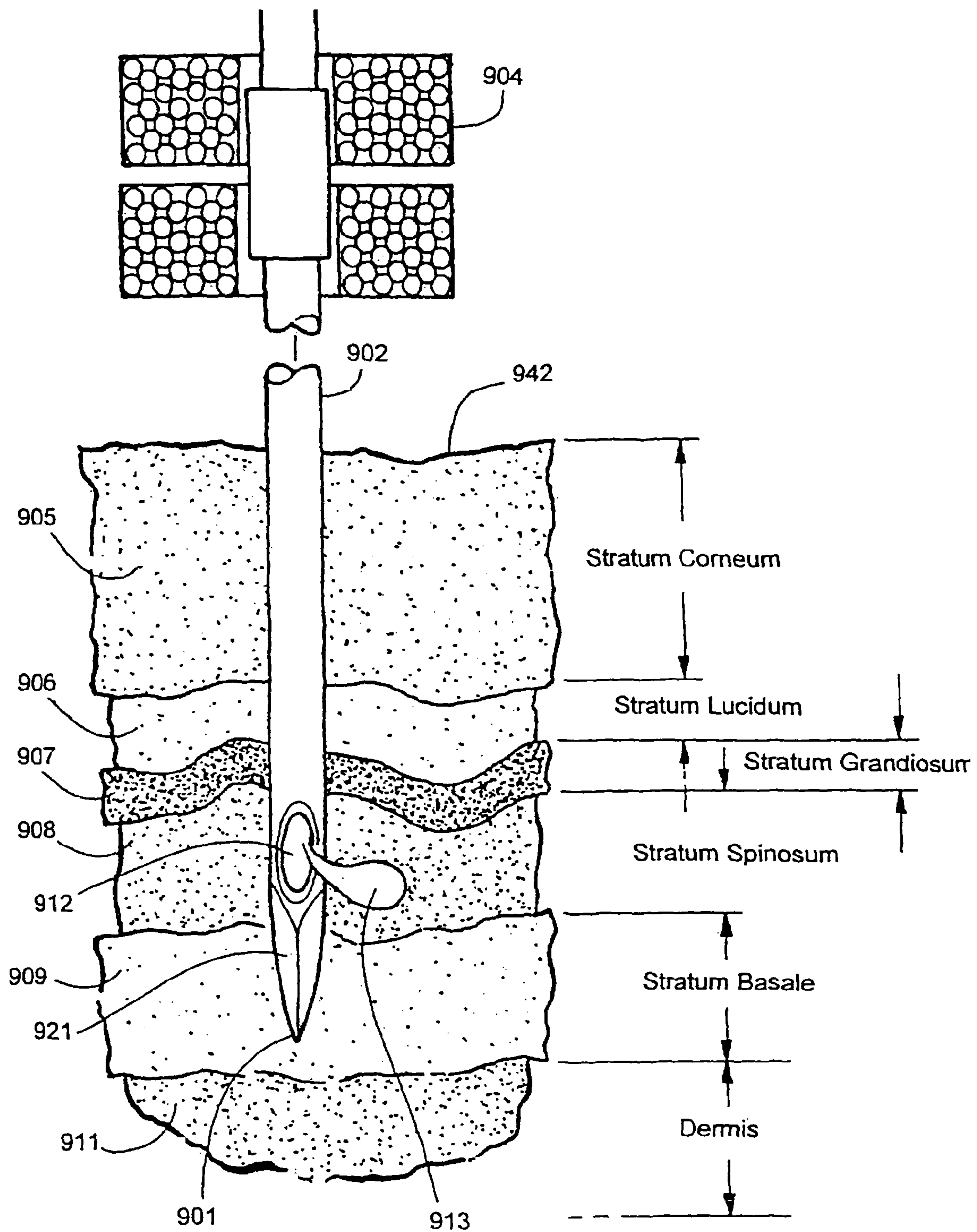
Syringe Needle
