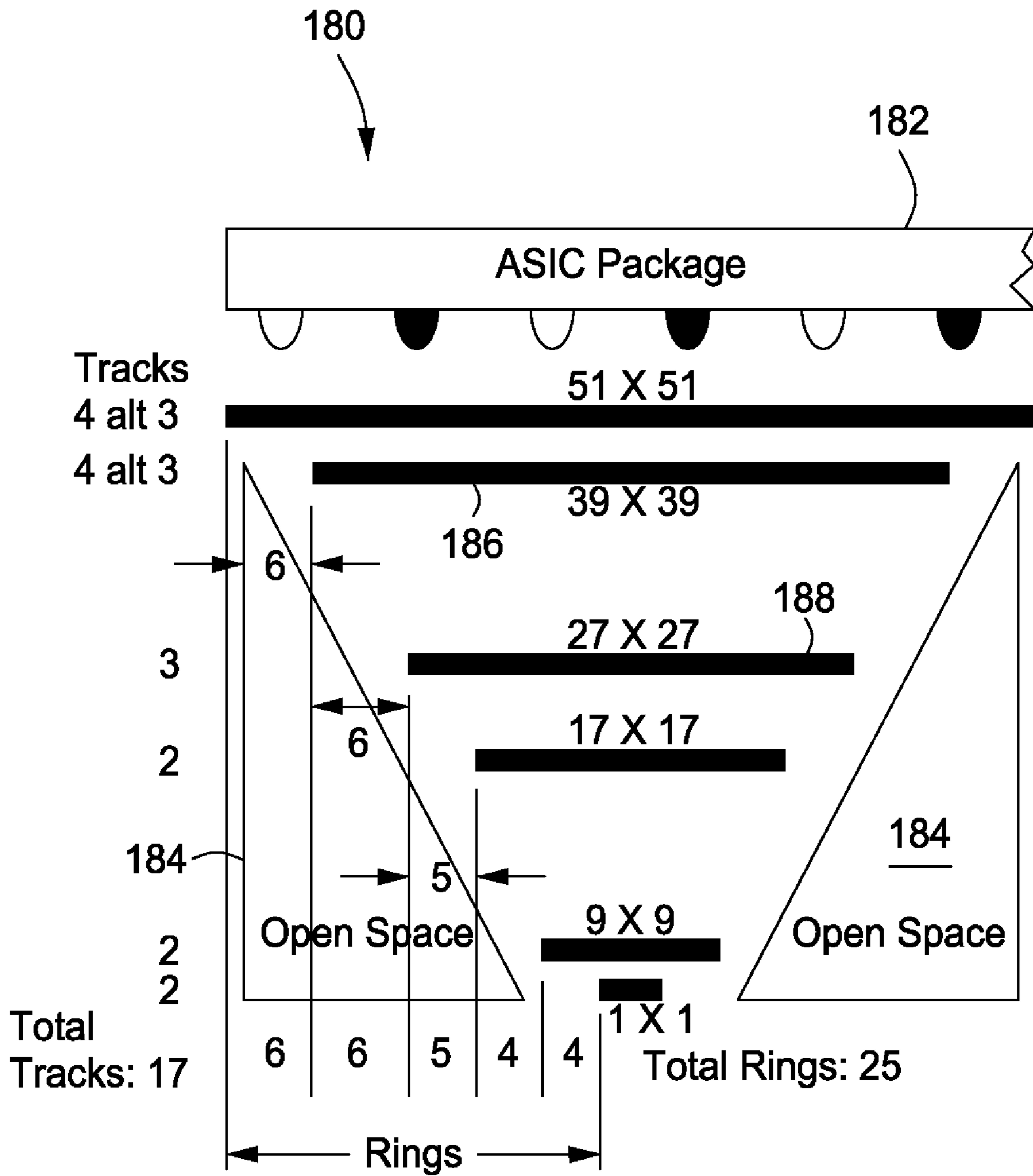
Escape Profile for 2,577 Pin 1mm CCGA
