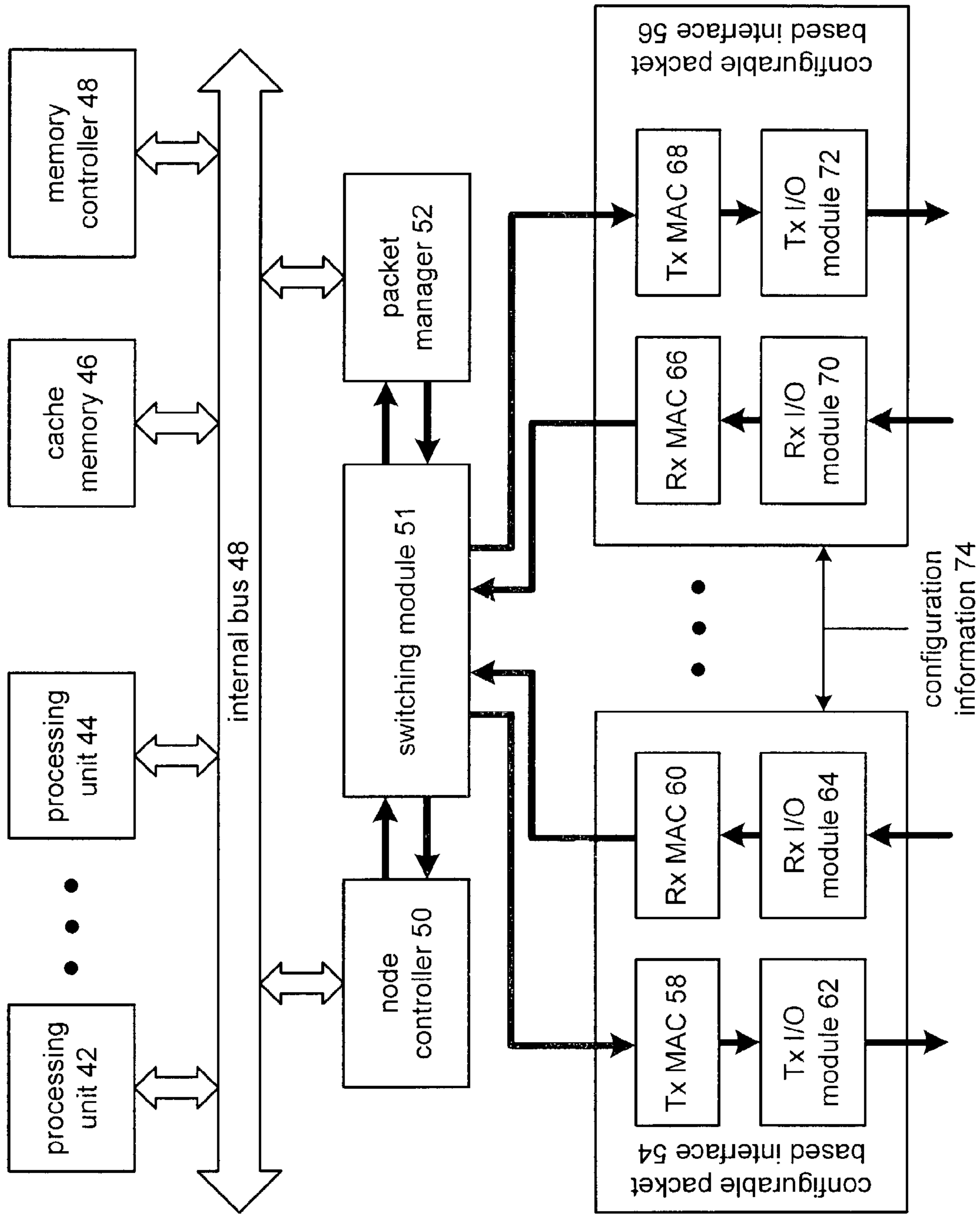
FIG. 4 multiple processor device 40
