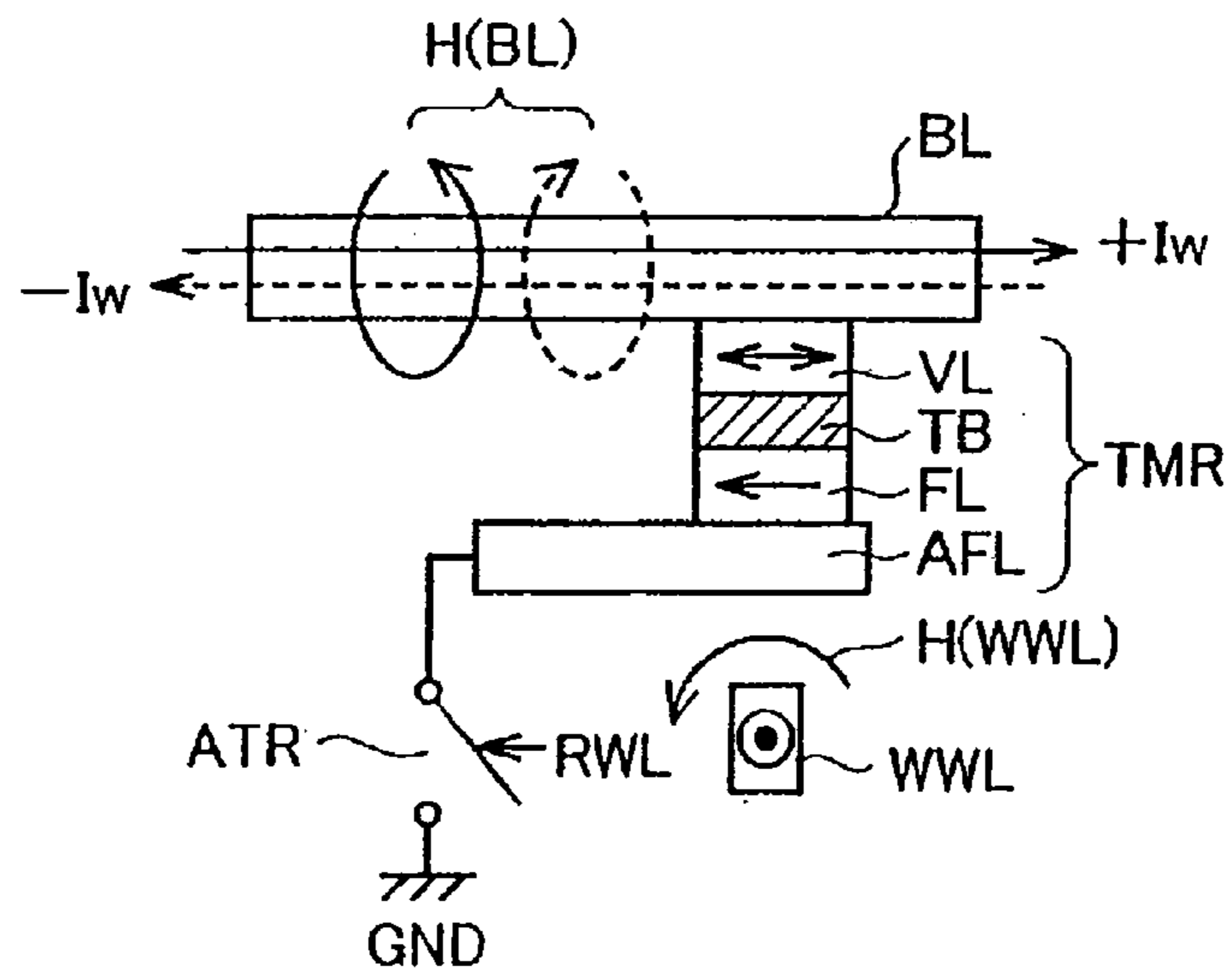
FIG.23 PRIOR ART
