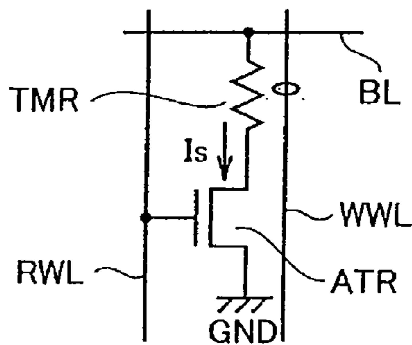
FIG.21 PRIOR ART
