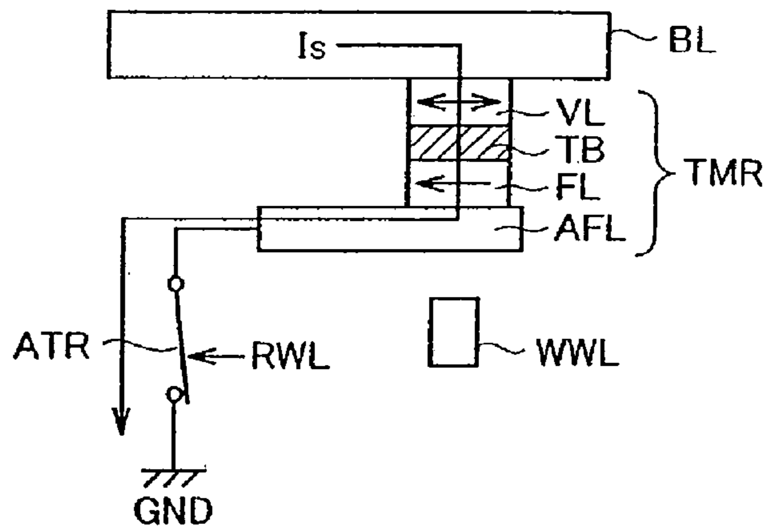
FIG.22 PRIOR ART
