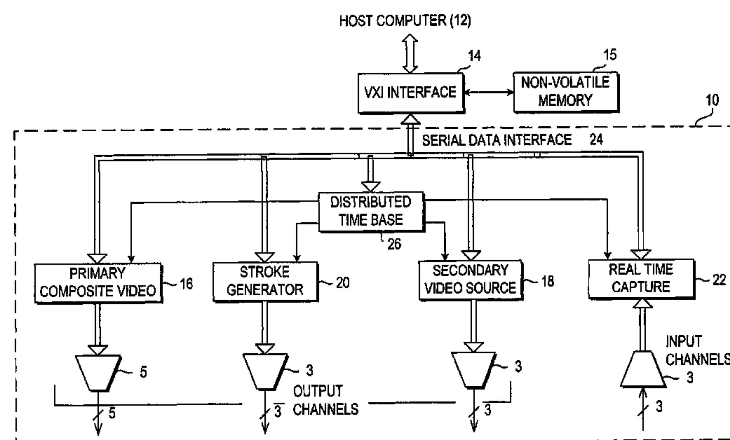
GENERAL ARRANGEMENT
