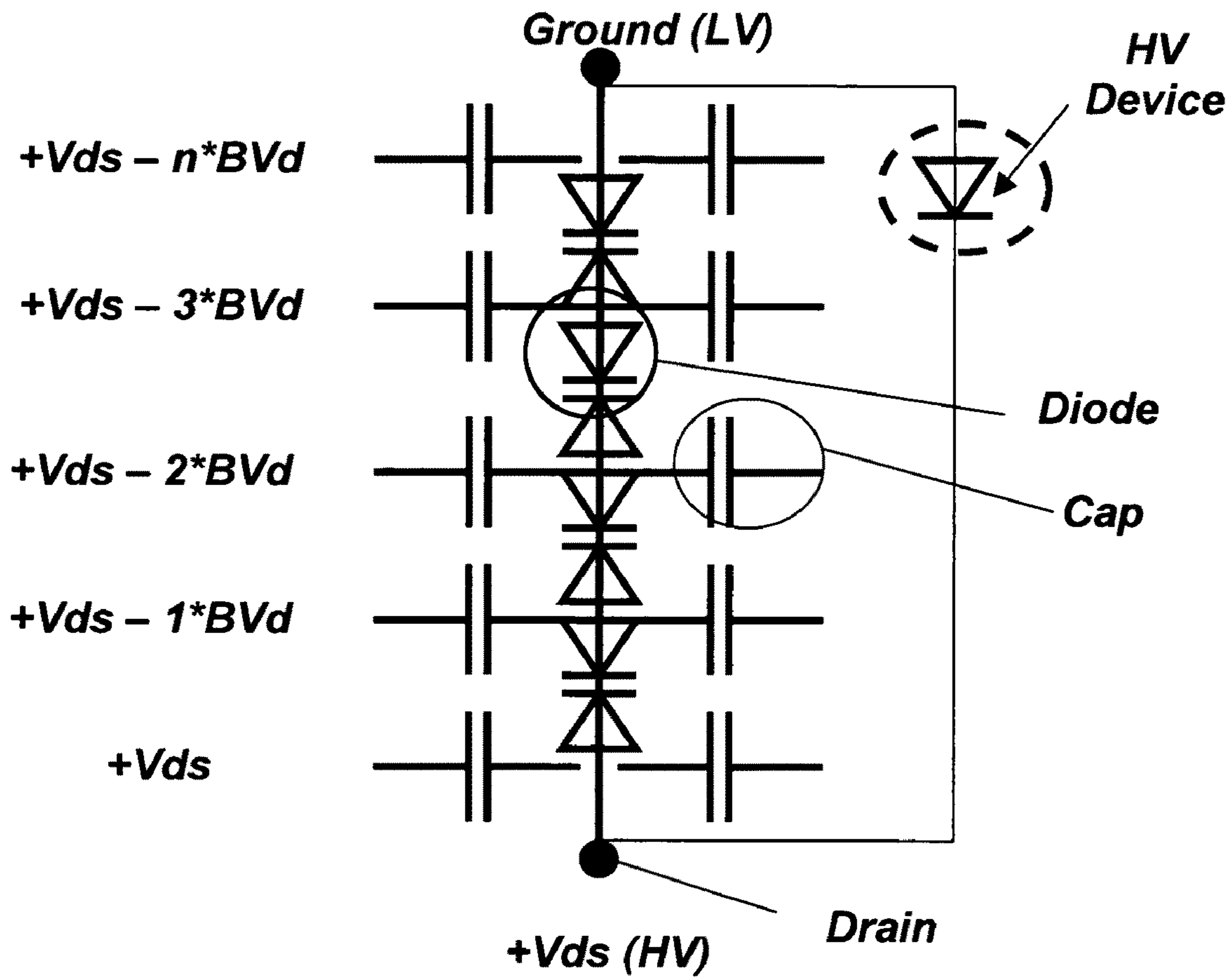
Fig. 3C-1 (Prior Art)
