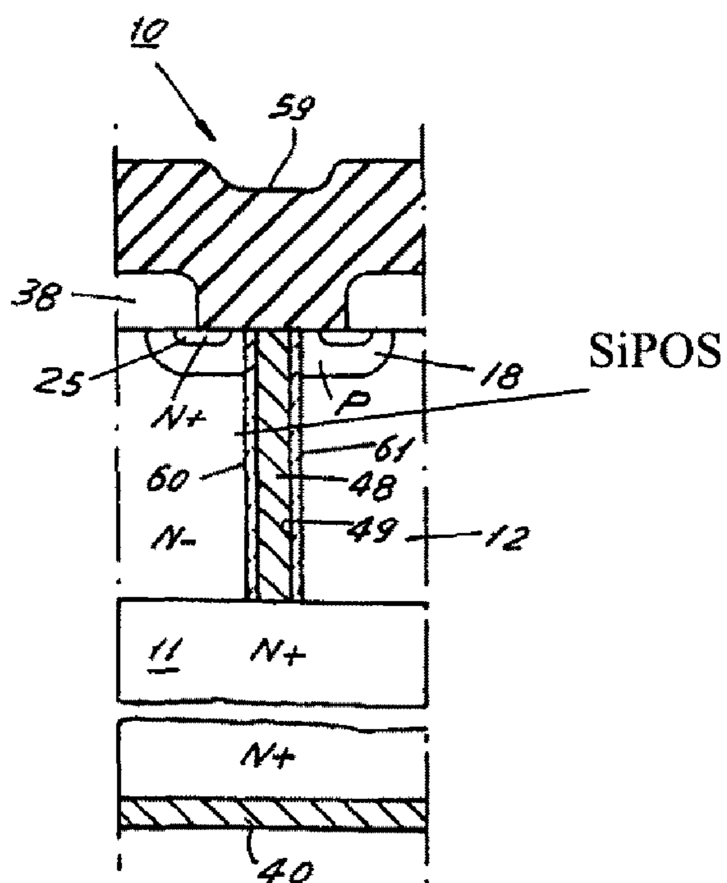
Fig. 3A-2 (Prior Art)
