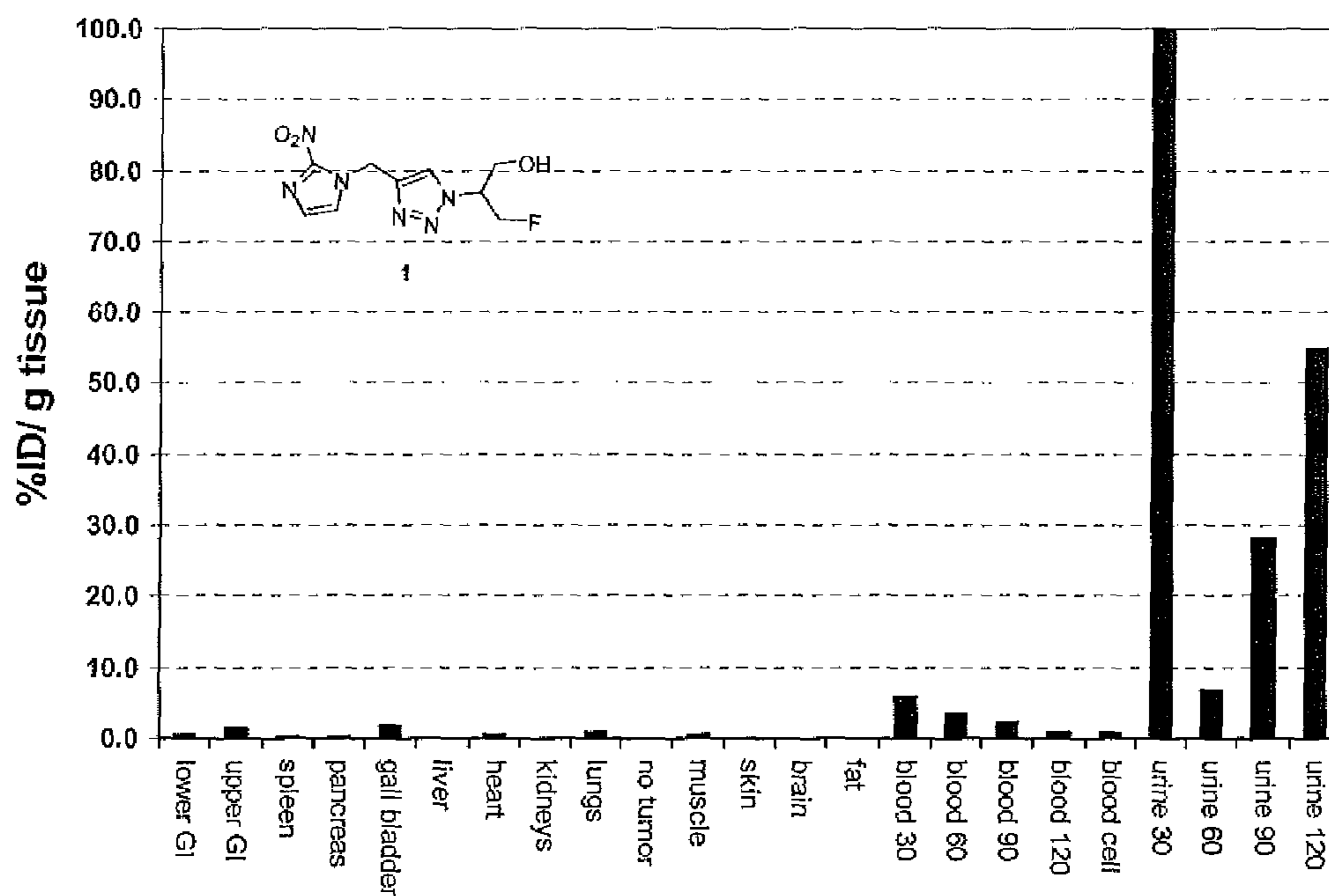
Figure 1: Bio-distribution of Compound 1 in male white mouse 120 min post IV injection (200 \mu l of a 5 mM solution).
