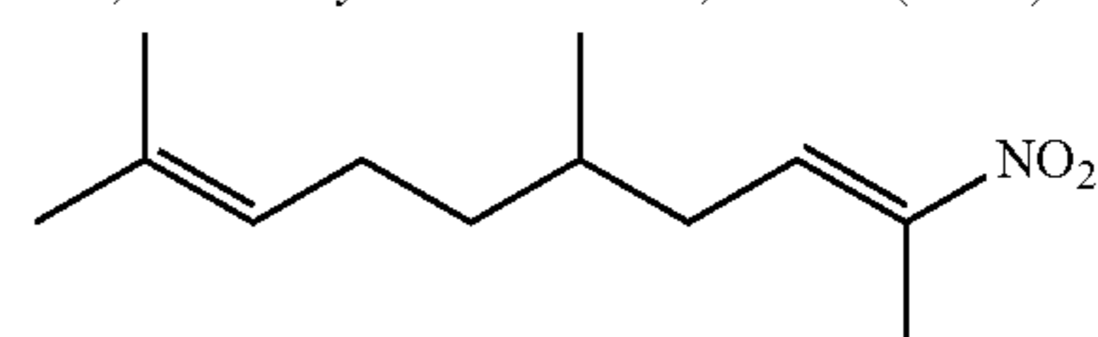
5,9-Dimethyl-2-nitrodeca-2,8-diene (RG-14)
