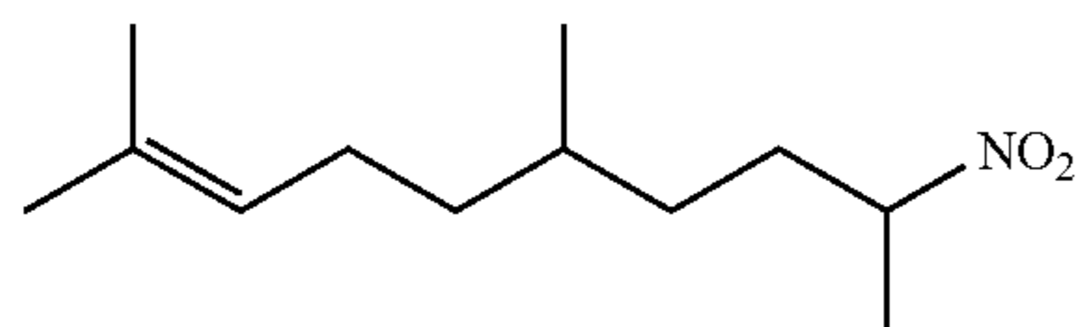
5,9-Dimethyl-2-nitro-8-decene (SRG-8)
