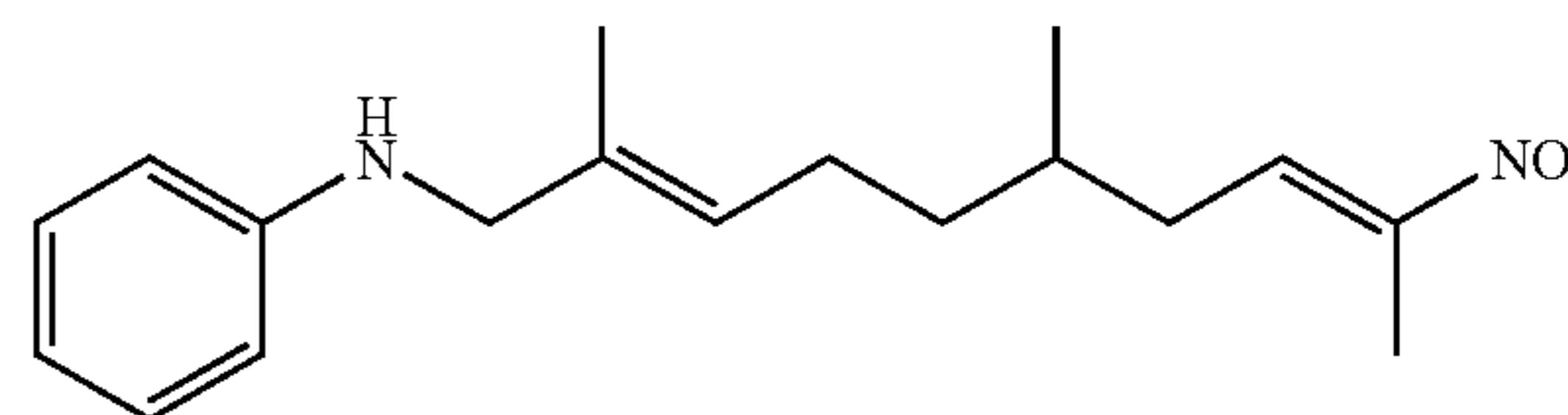
5,9-Dimethyl-2-nitro-10-(phenylamino)-deca-2,8-diene
