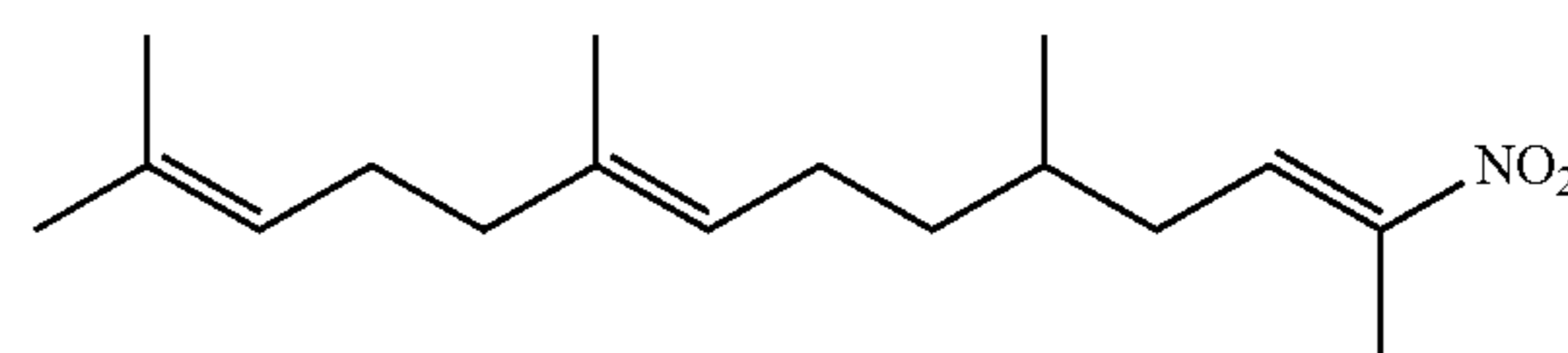
5,9,13-Trimethyl-2-nitrotetradeca-2,8,12-triene (RG-4)
