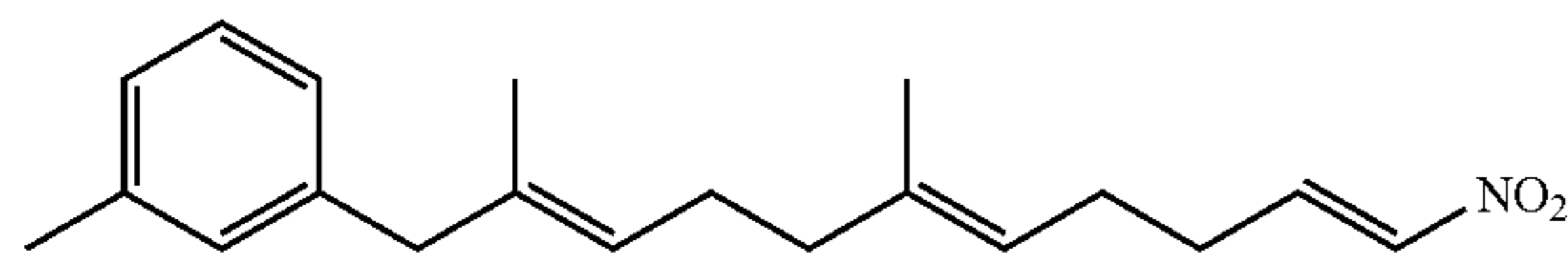
6,10-Dimethyl-11-(3-methylphenyl)-1-nitroundeca-1,5,9-triene
