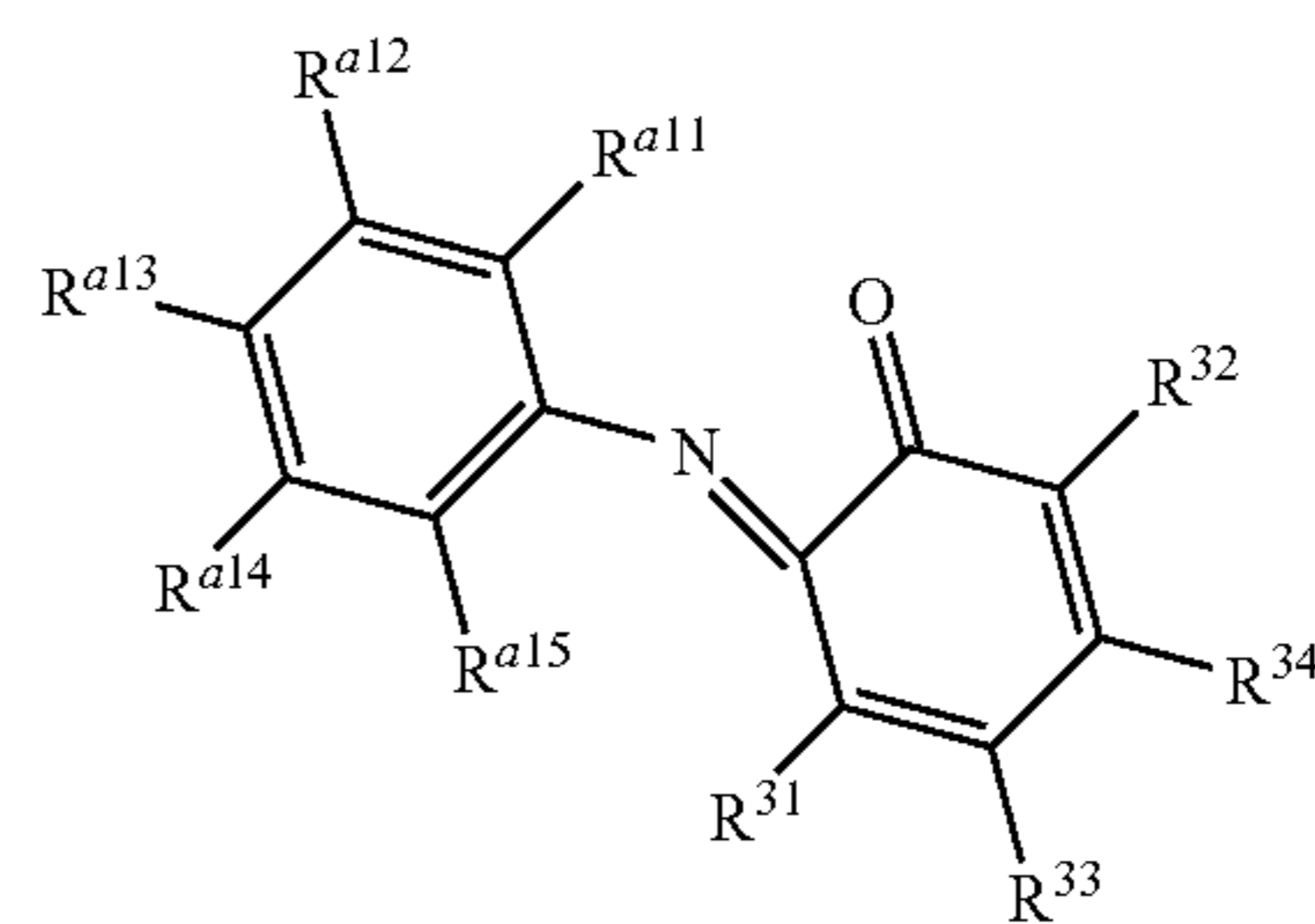
Structure 33b
