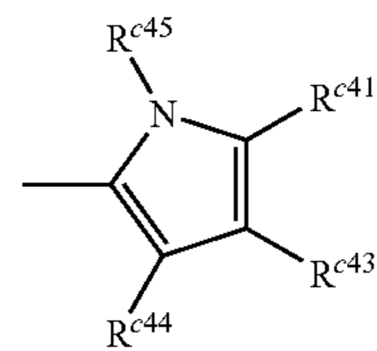
Structure 17c
