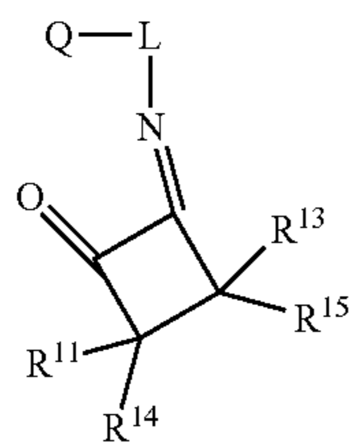
Structure 16b
