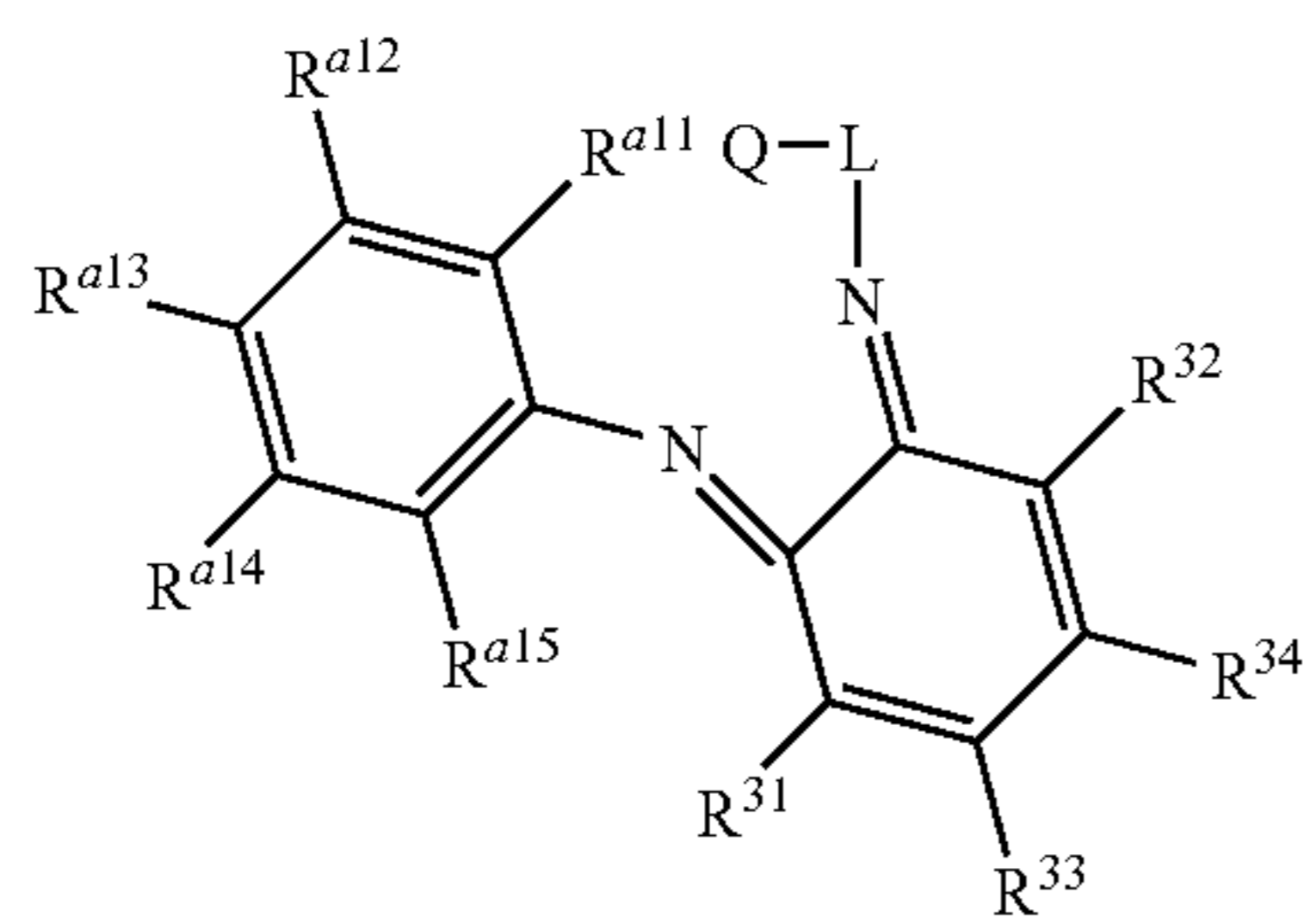
Structure 33f
