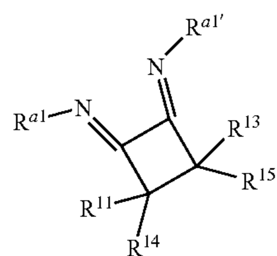
Structure 3f
