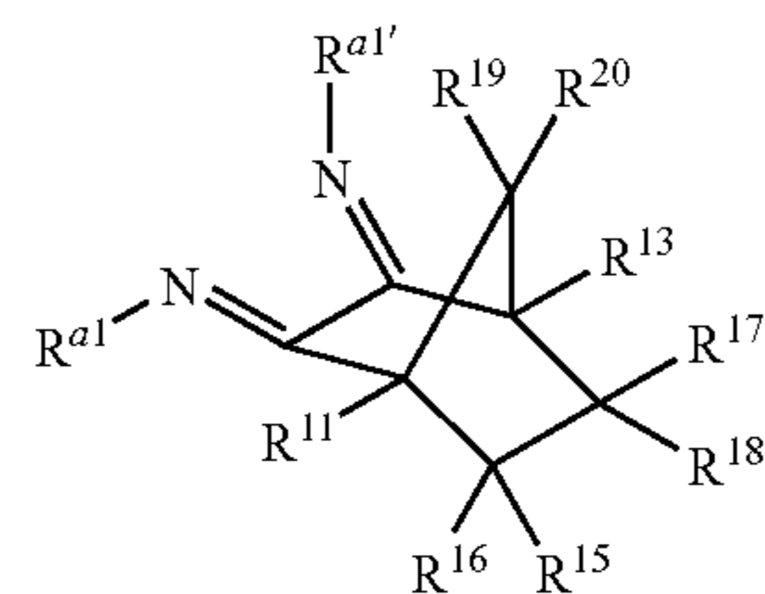
Structure 6f
