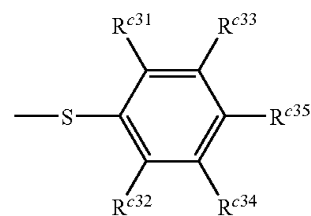
Structure 15c
