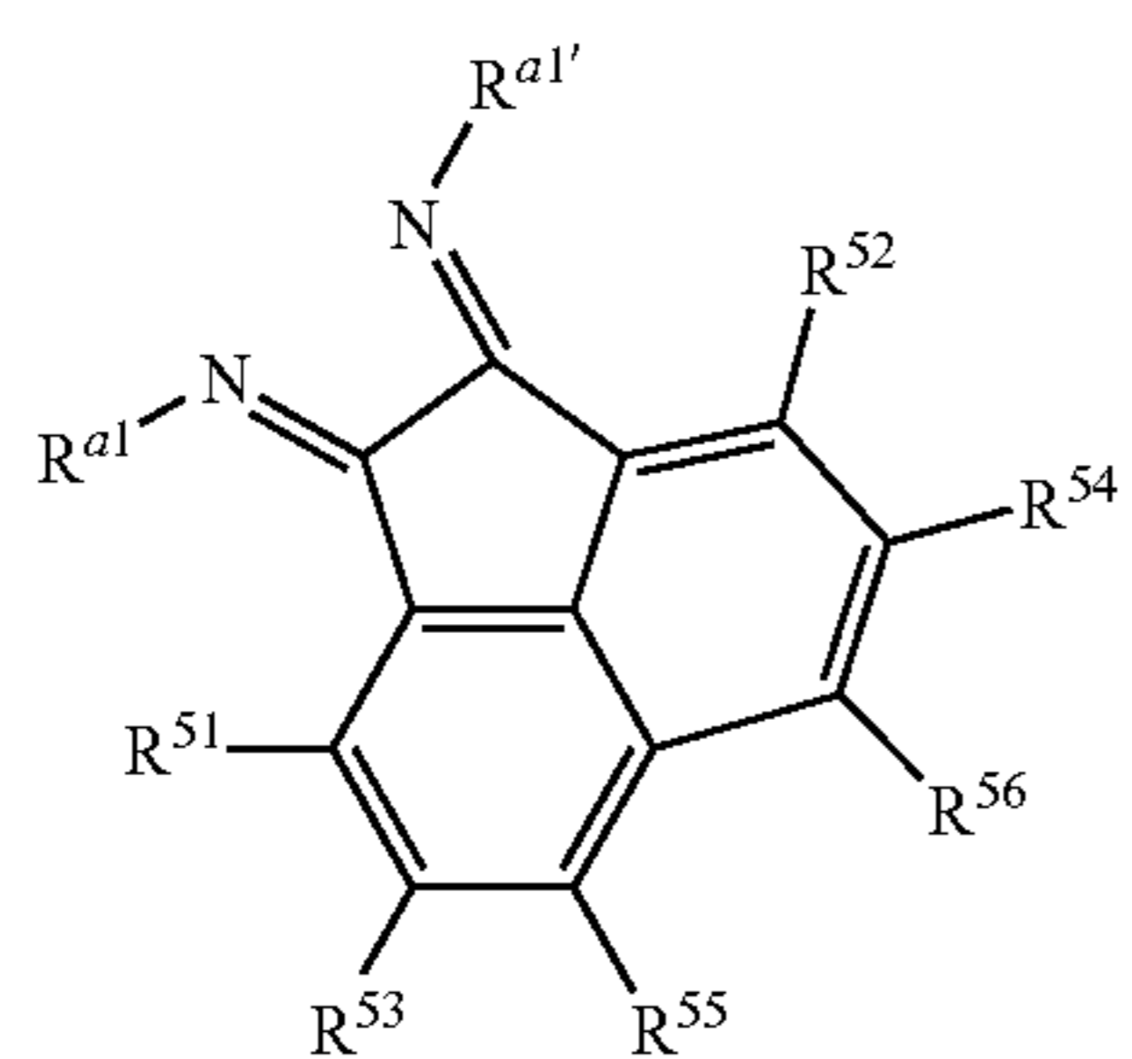
Structure 11f
