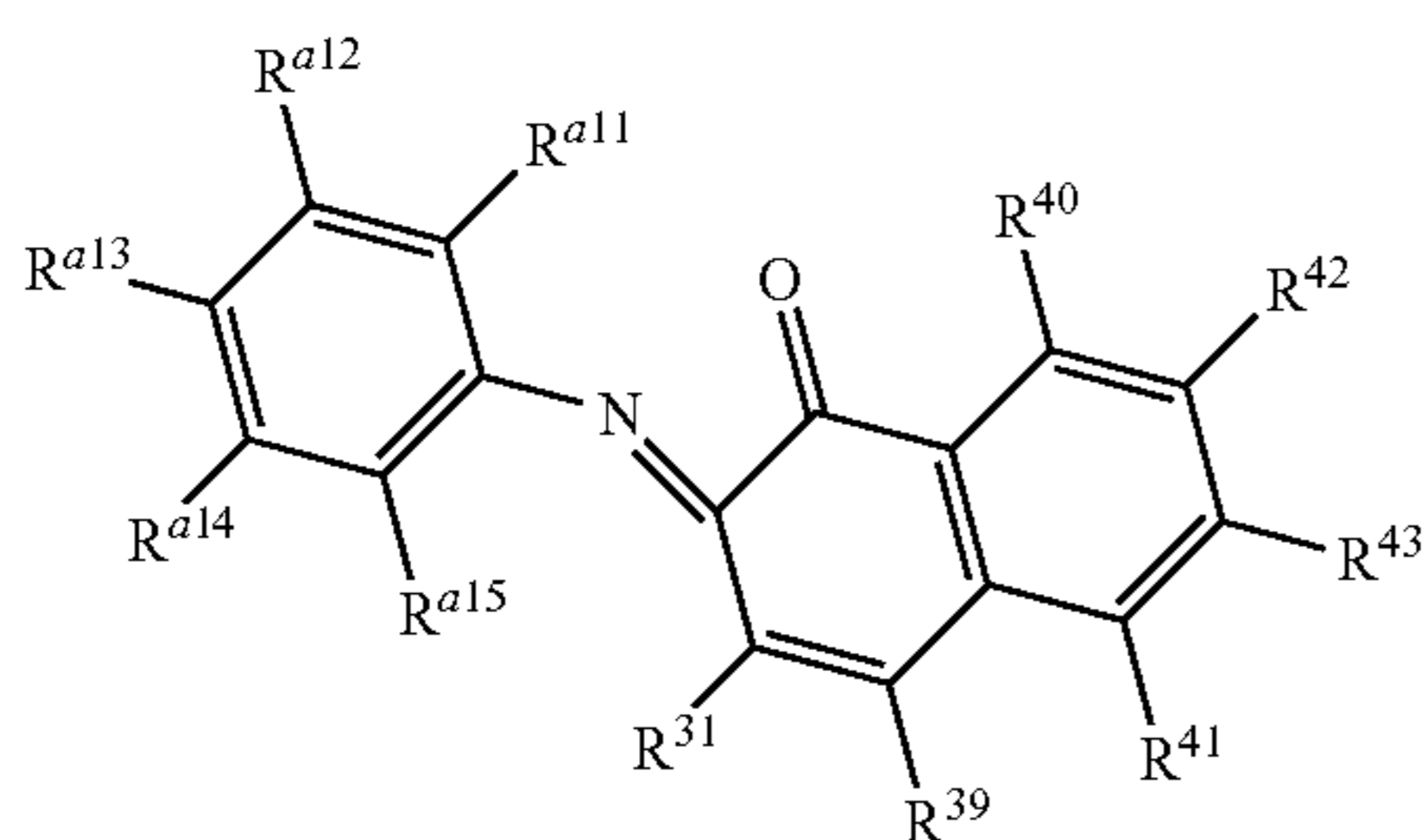
Structure 35b
