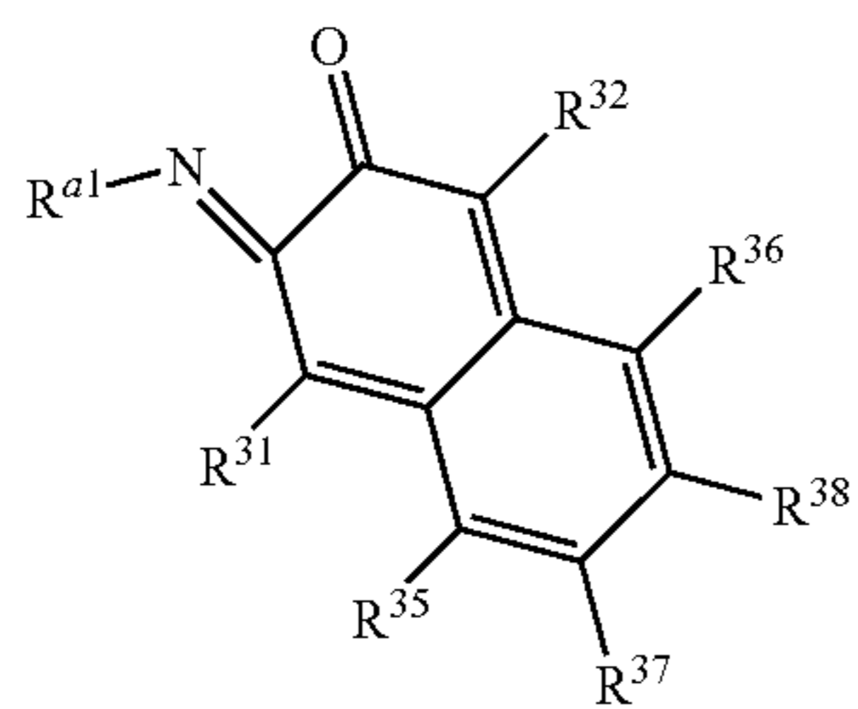
Structure 8b
