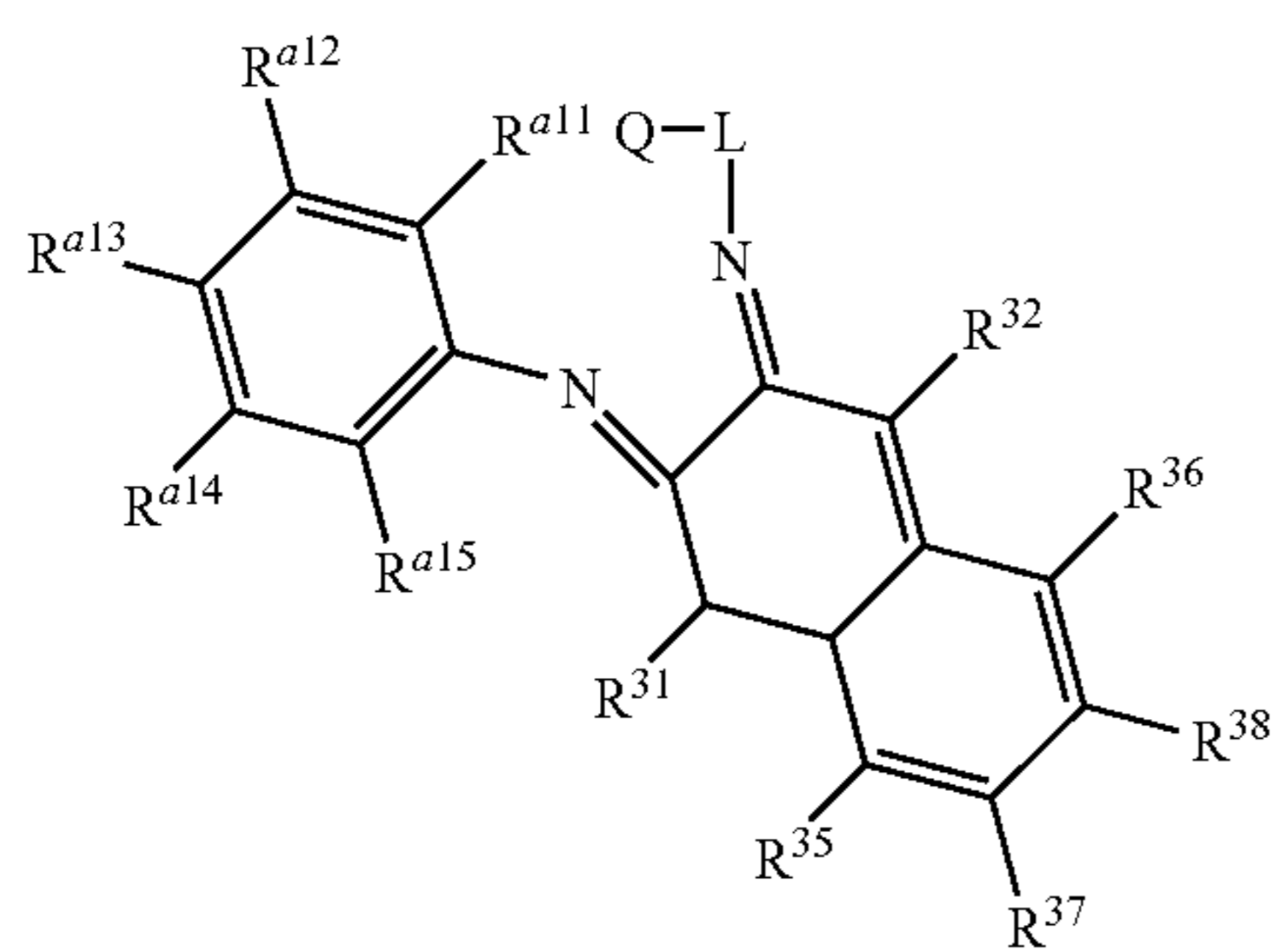
Structure 34f
