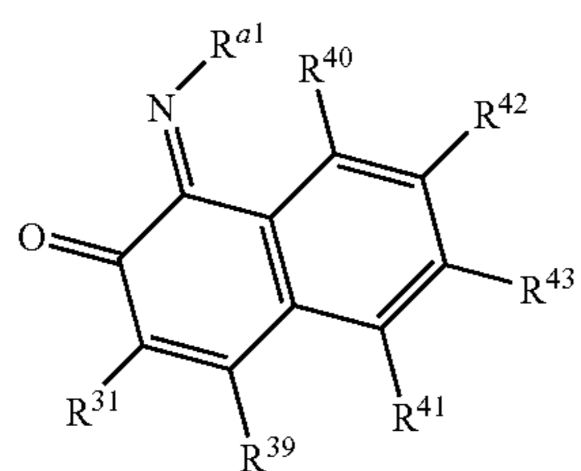
Structure 10b
