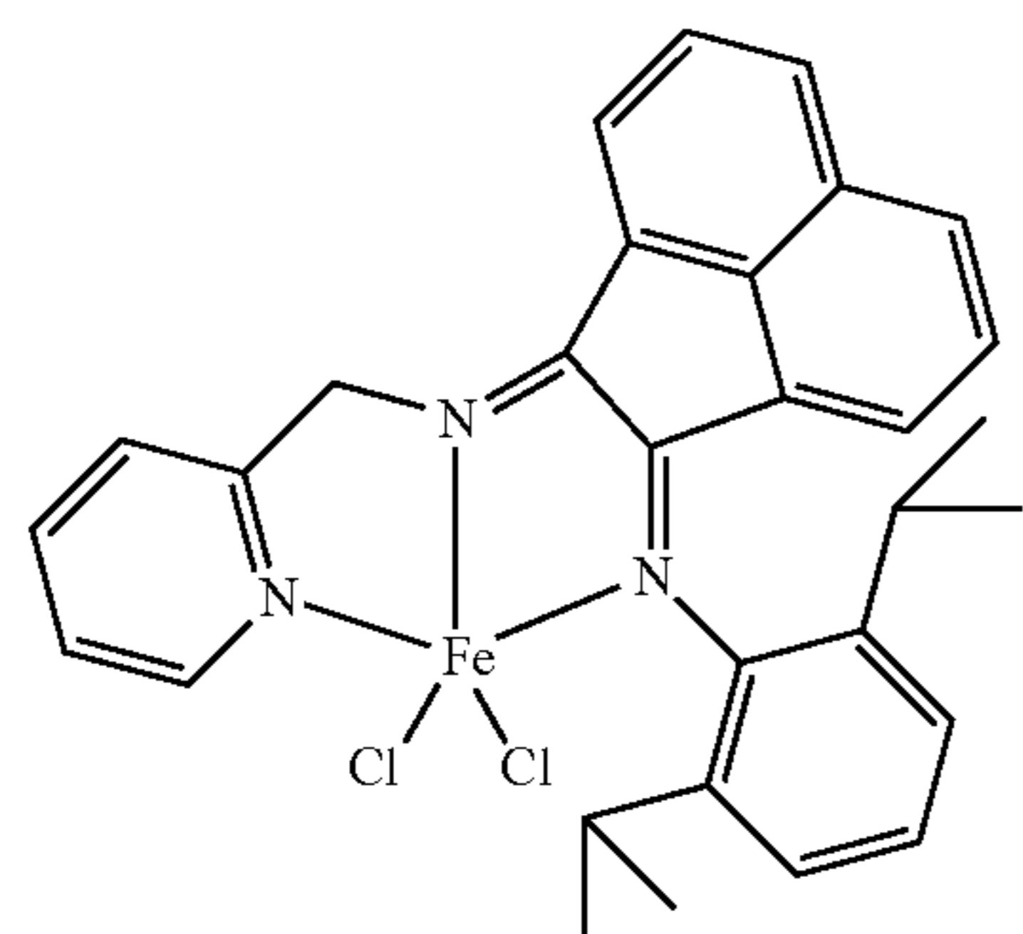
Structure II
