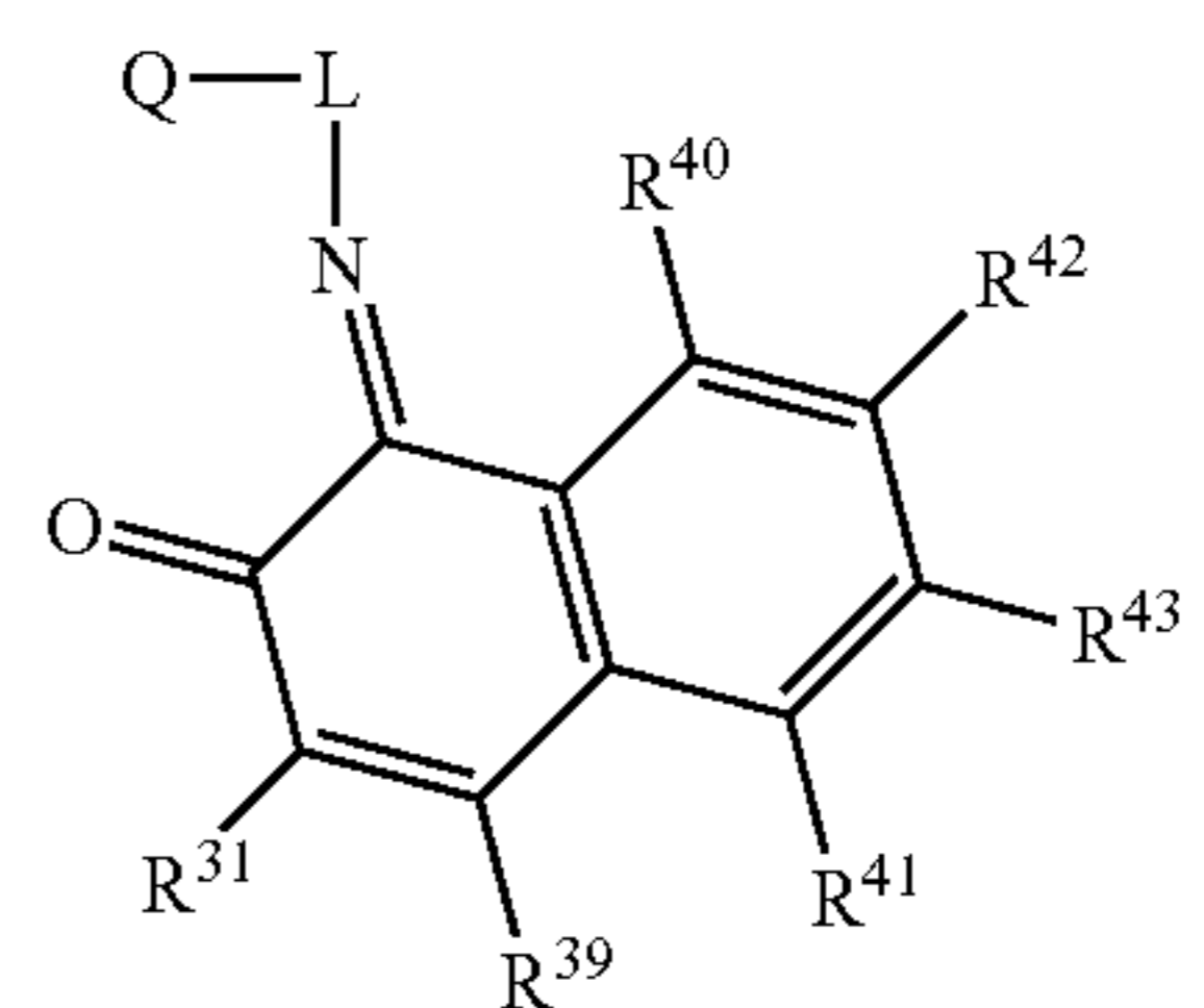
Structure 22b
