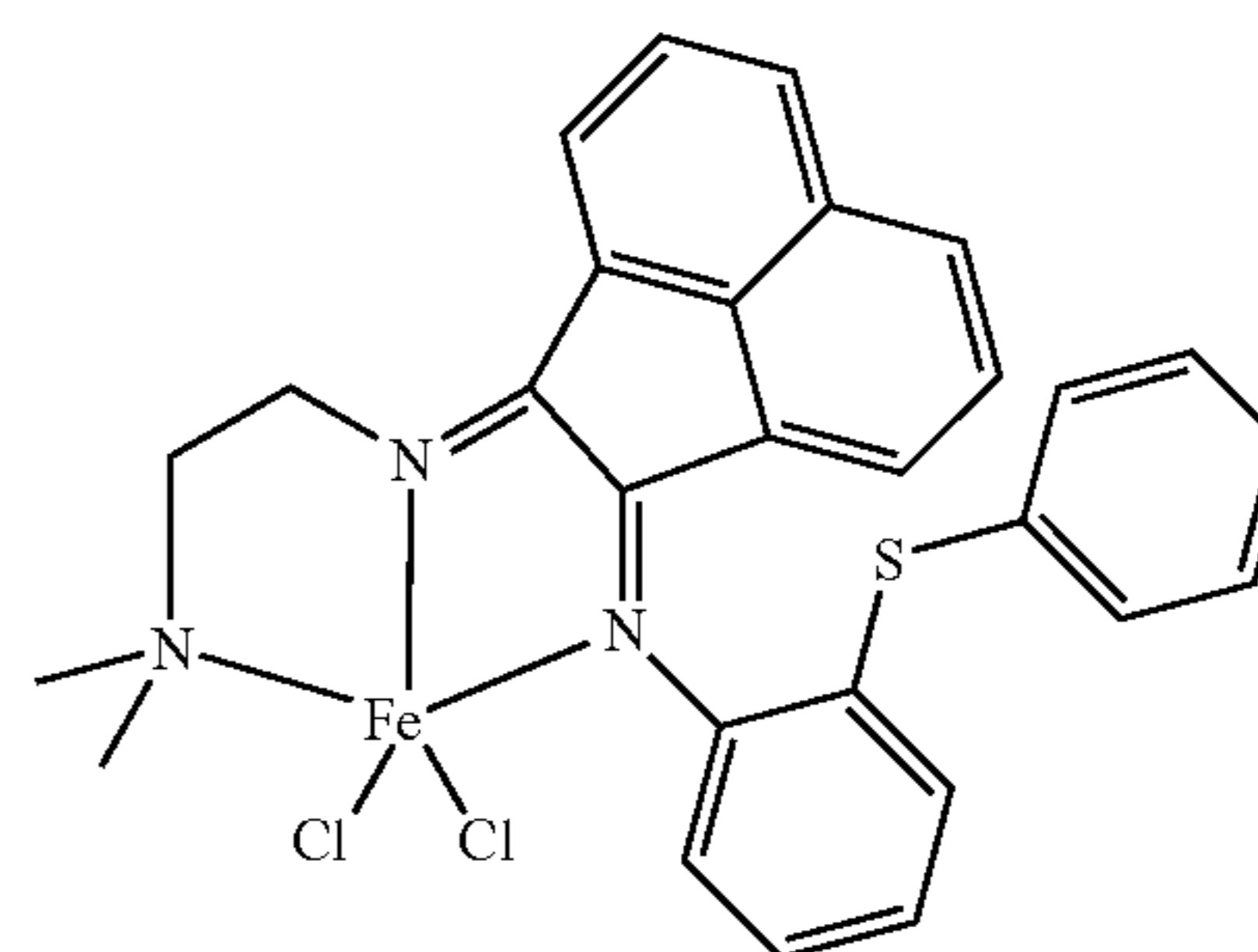
Structure XVI
