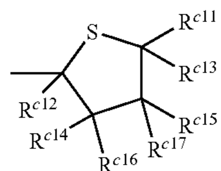
Structure 12c
