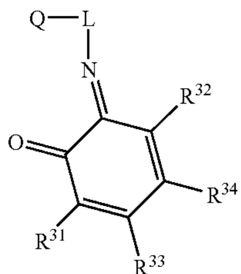
Structure 20b
