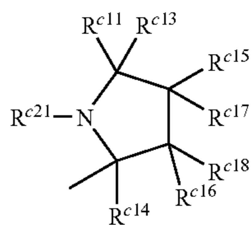
Structure 8c
