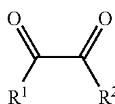
Structure 1
