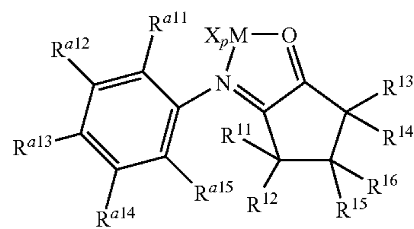
Structure 30d
