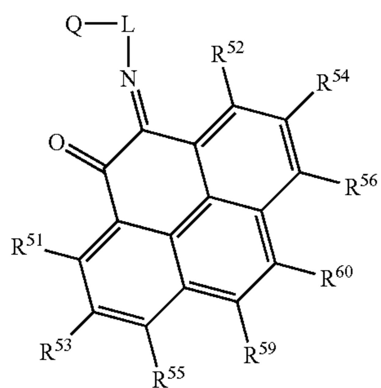
Structure 26b
