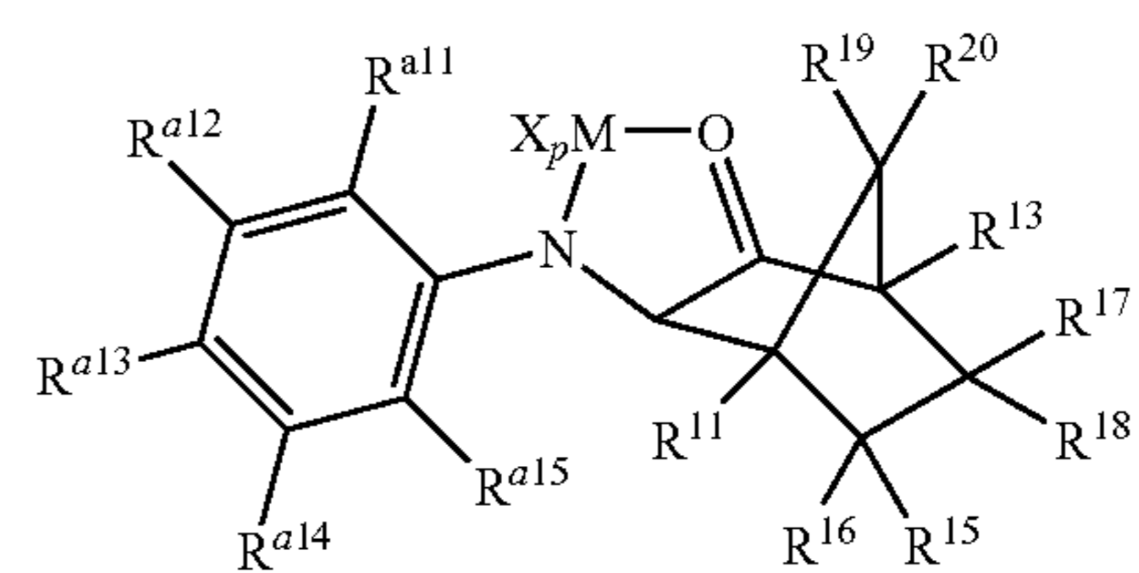
Structure 32d
