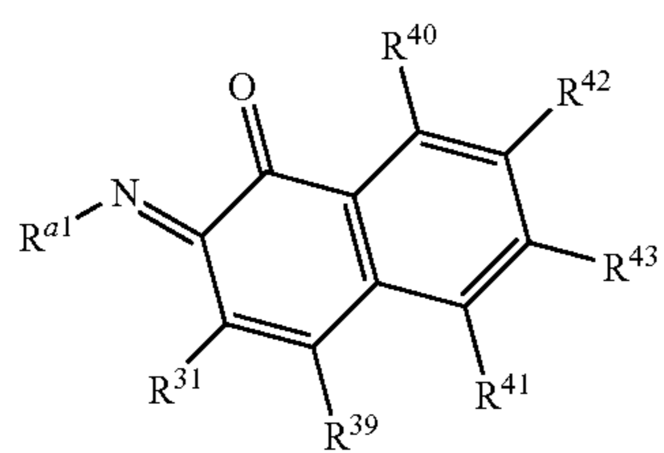
Structure 9b
