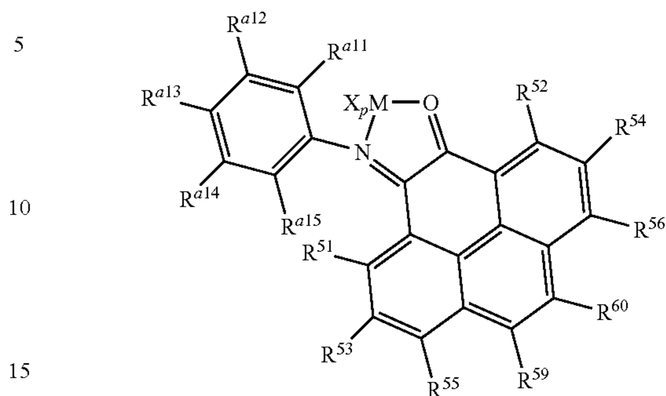
Structure 39d
