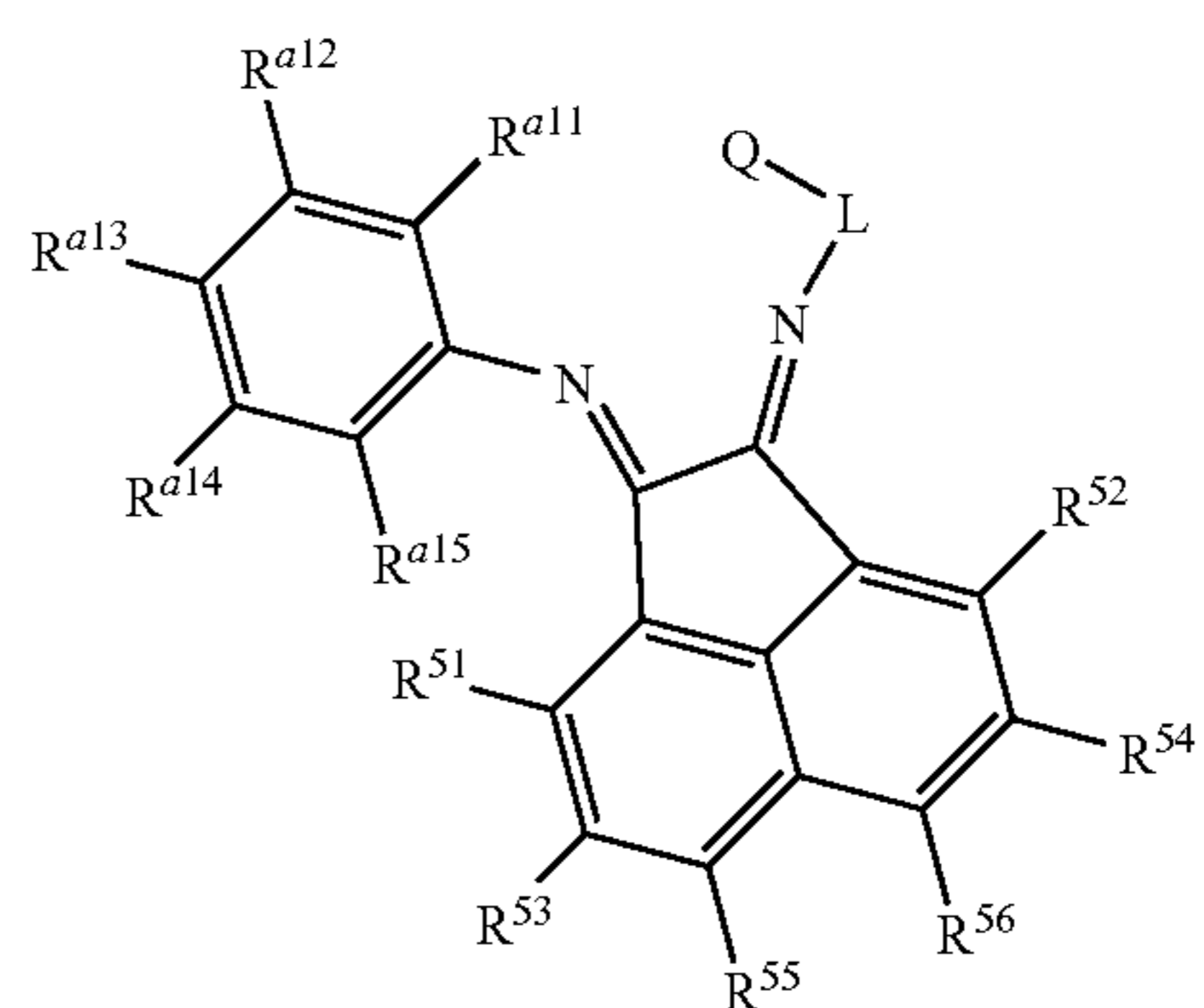
Structure 37f
