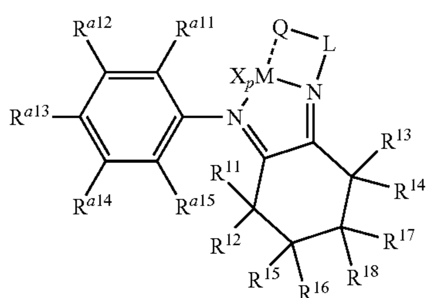
Structure 31e
