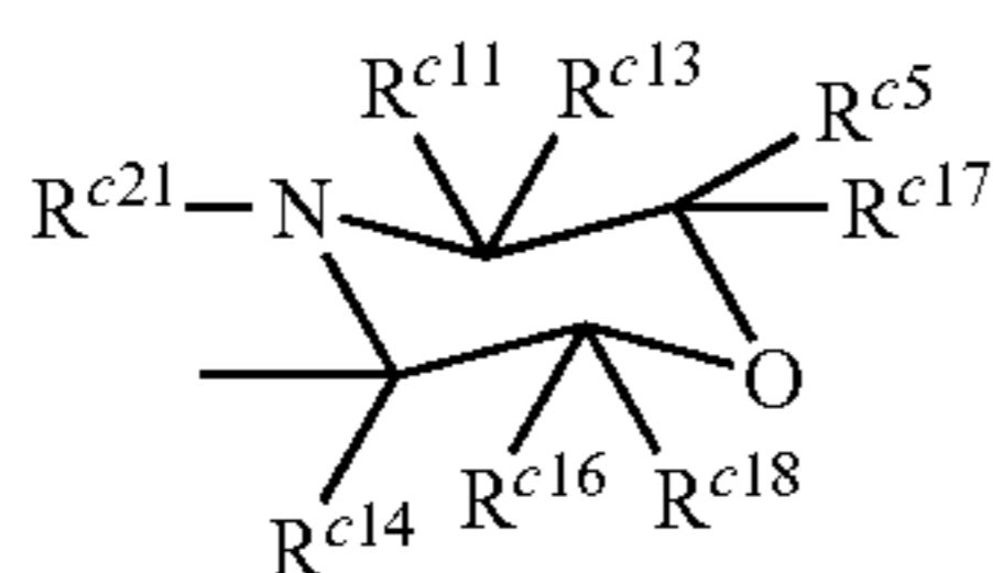
Structure 10c
