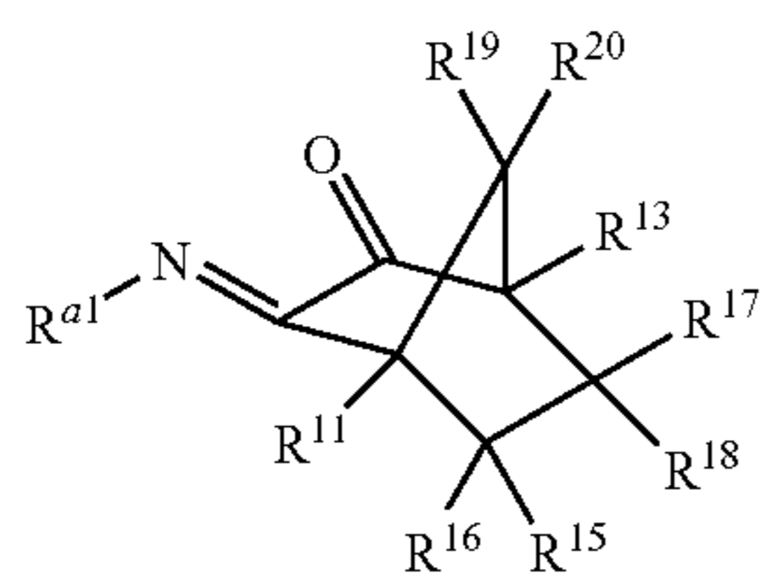
Structure 6b
