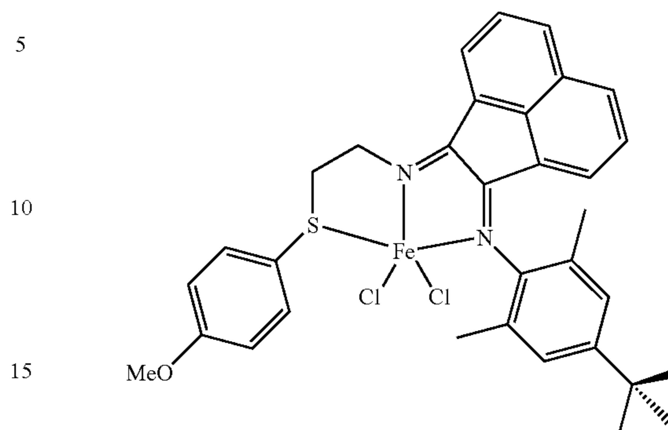
Structure XXXIX
