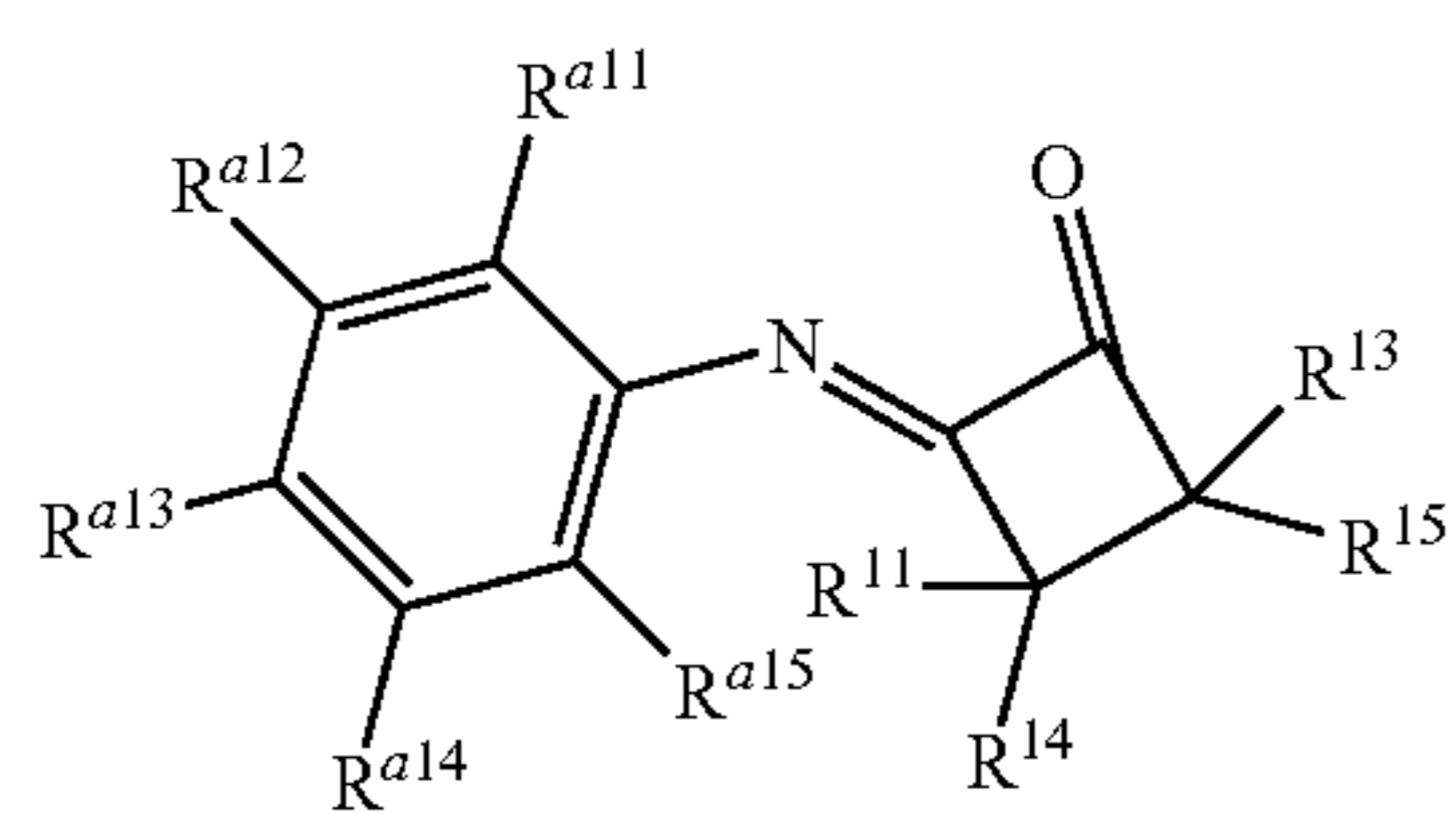
Structure 29b
