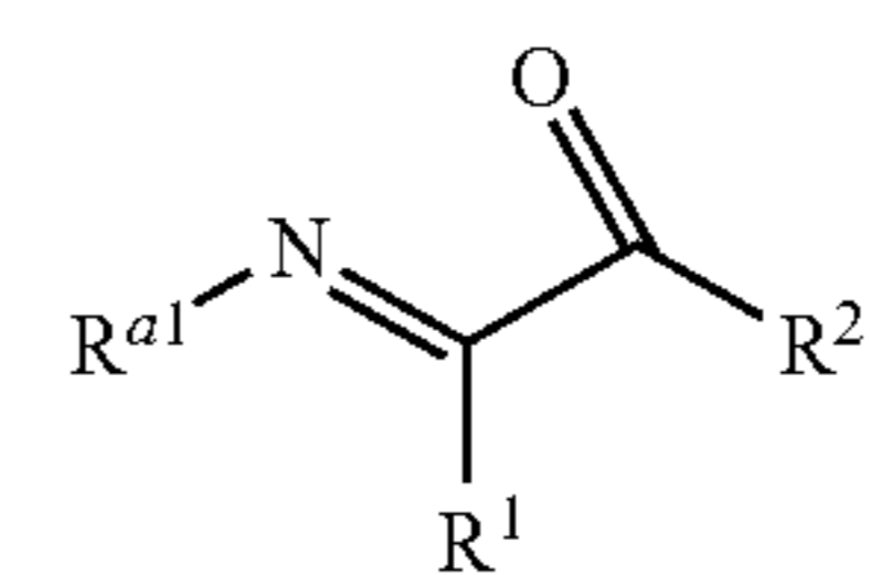
Structure 1b
