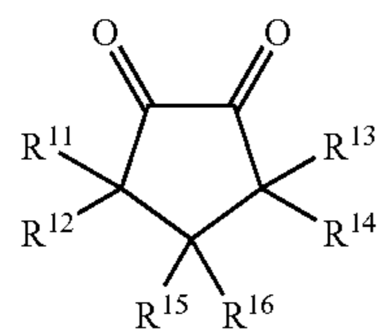
Structure 4
