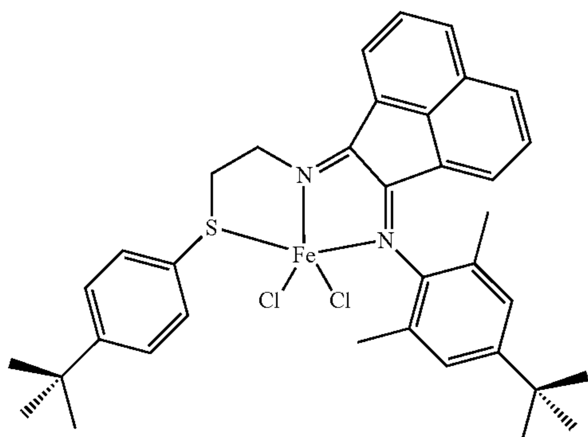
Structure XXXV
