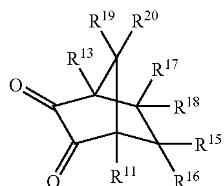
Structure 6
