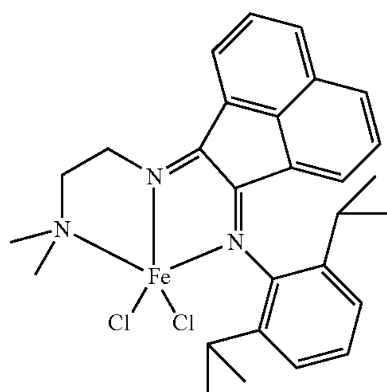
Structure XI
