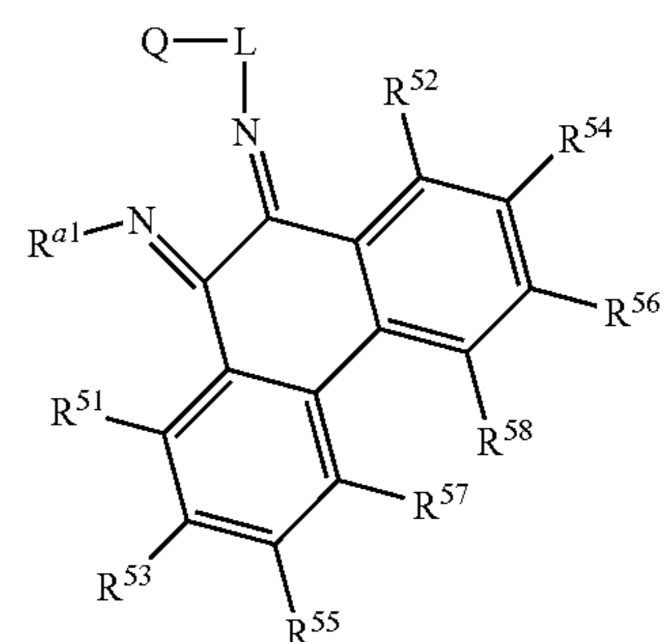
Structure 25f
