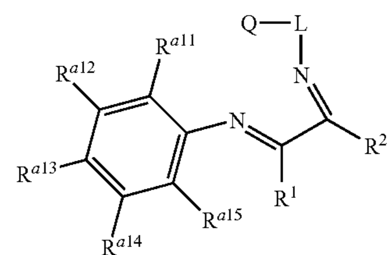
Structure 27f
