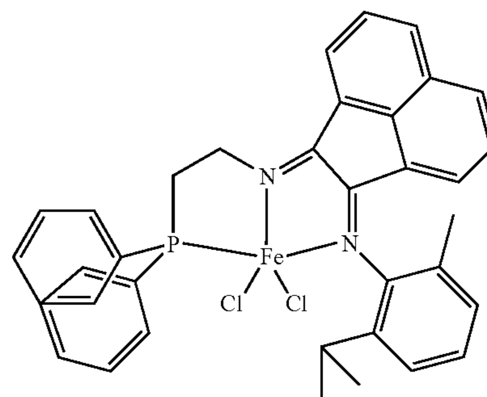
Structure XIV
