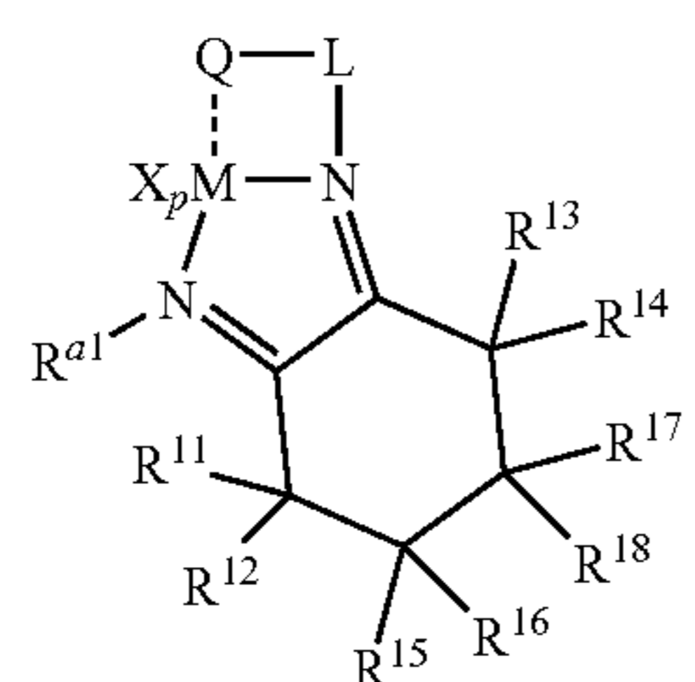
Structure 18c
