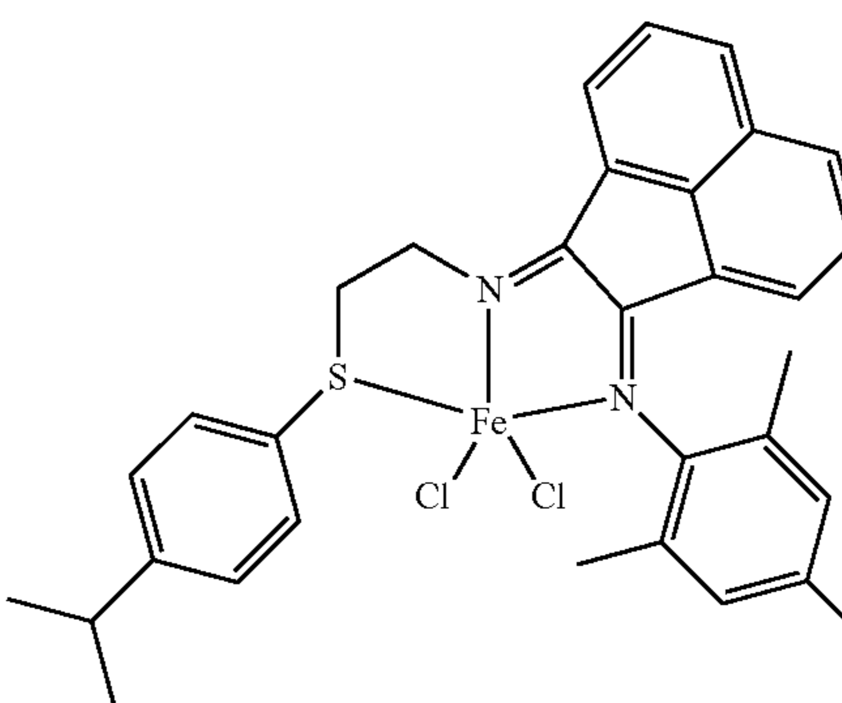
Structure XXXIII
