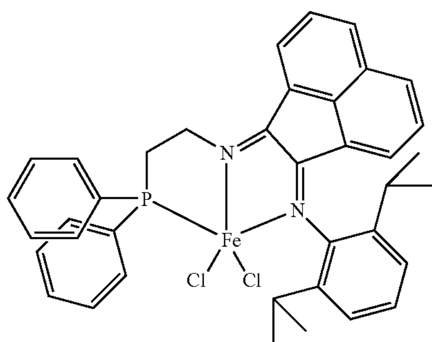
Structure III
