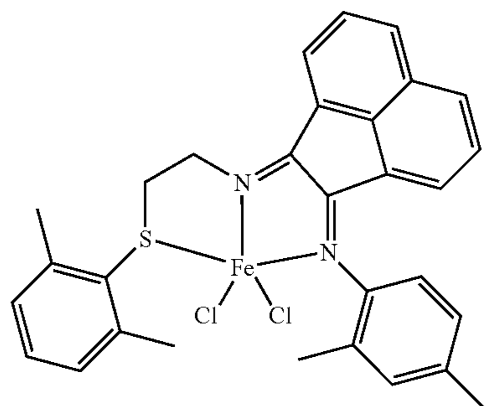
Structure XXXVIII
