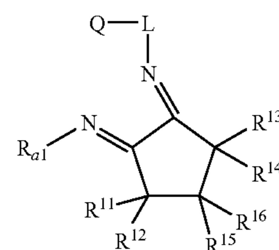
Structure 17f
