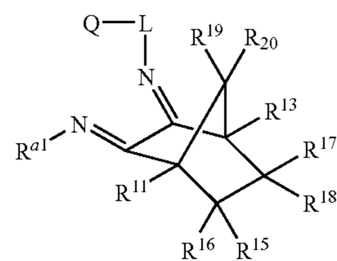
Structure 19f
