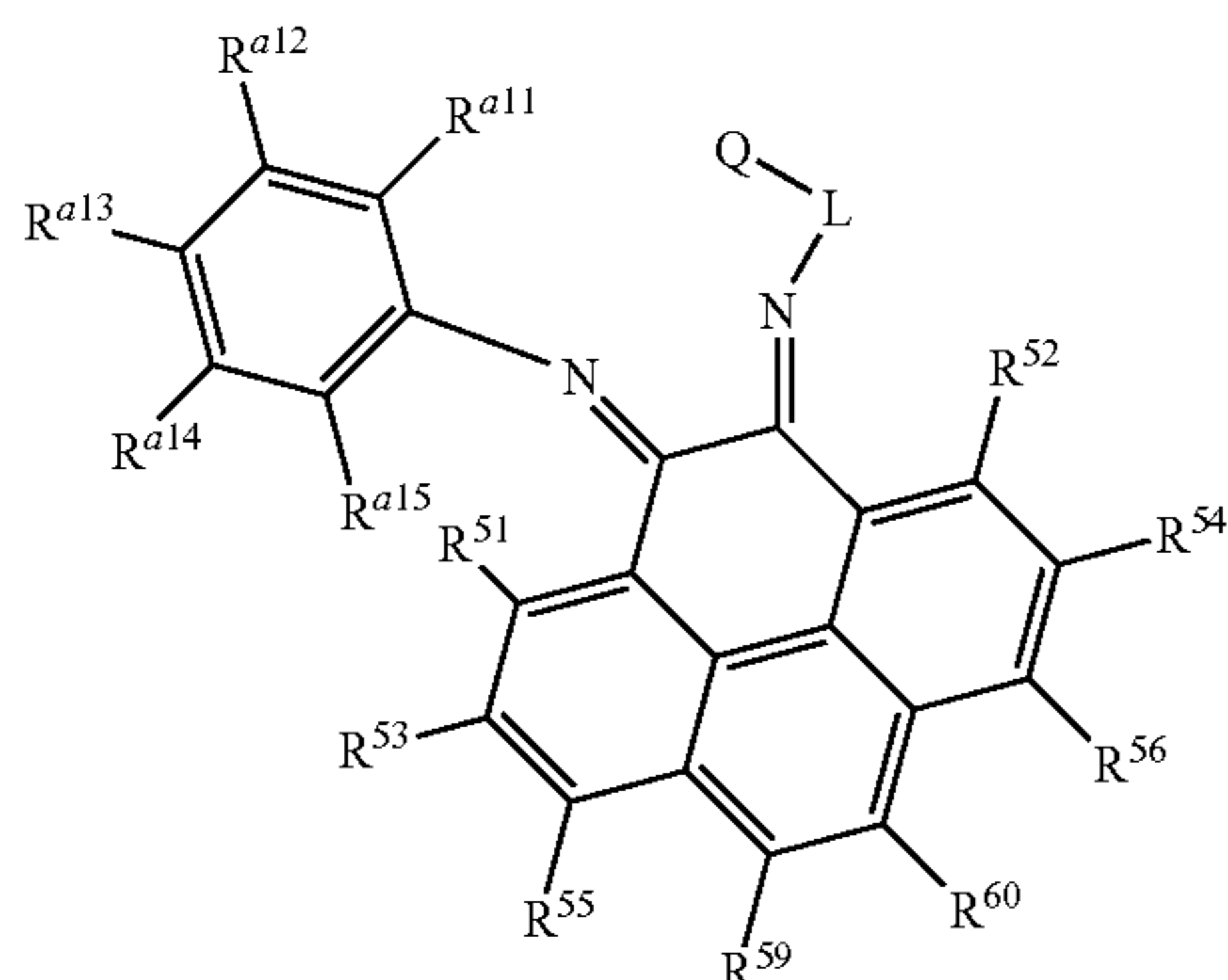
Structure 39f
