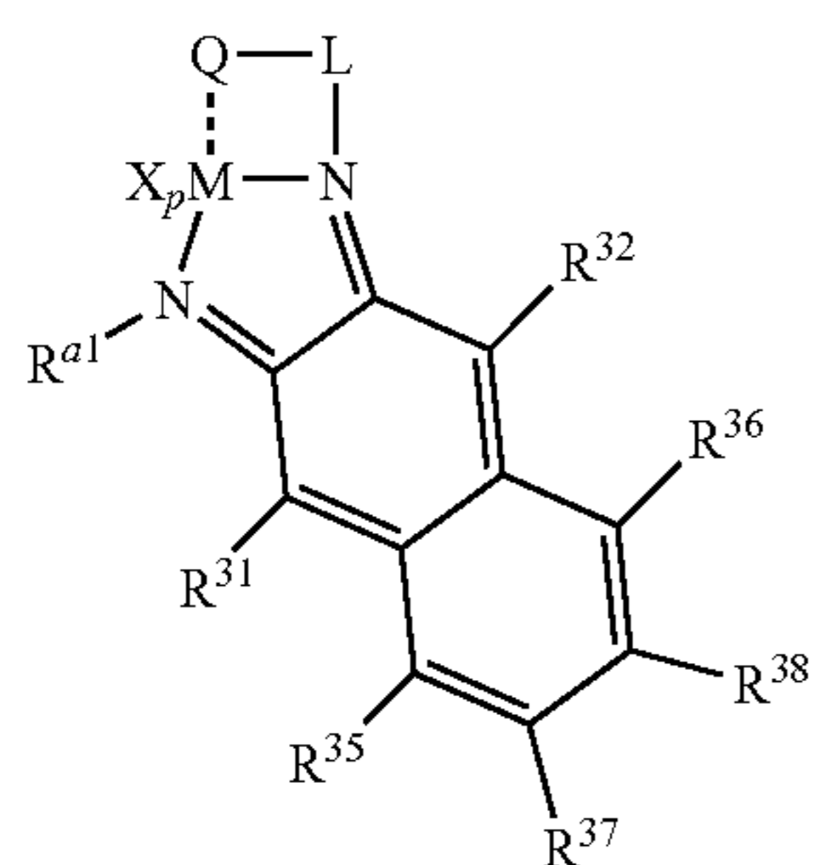
Structure 21e
