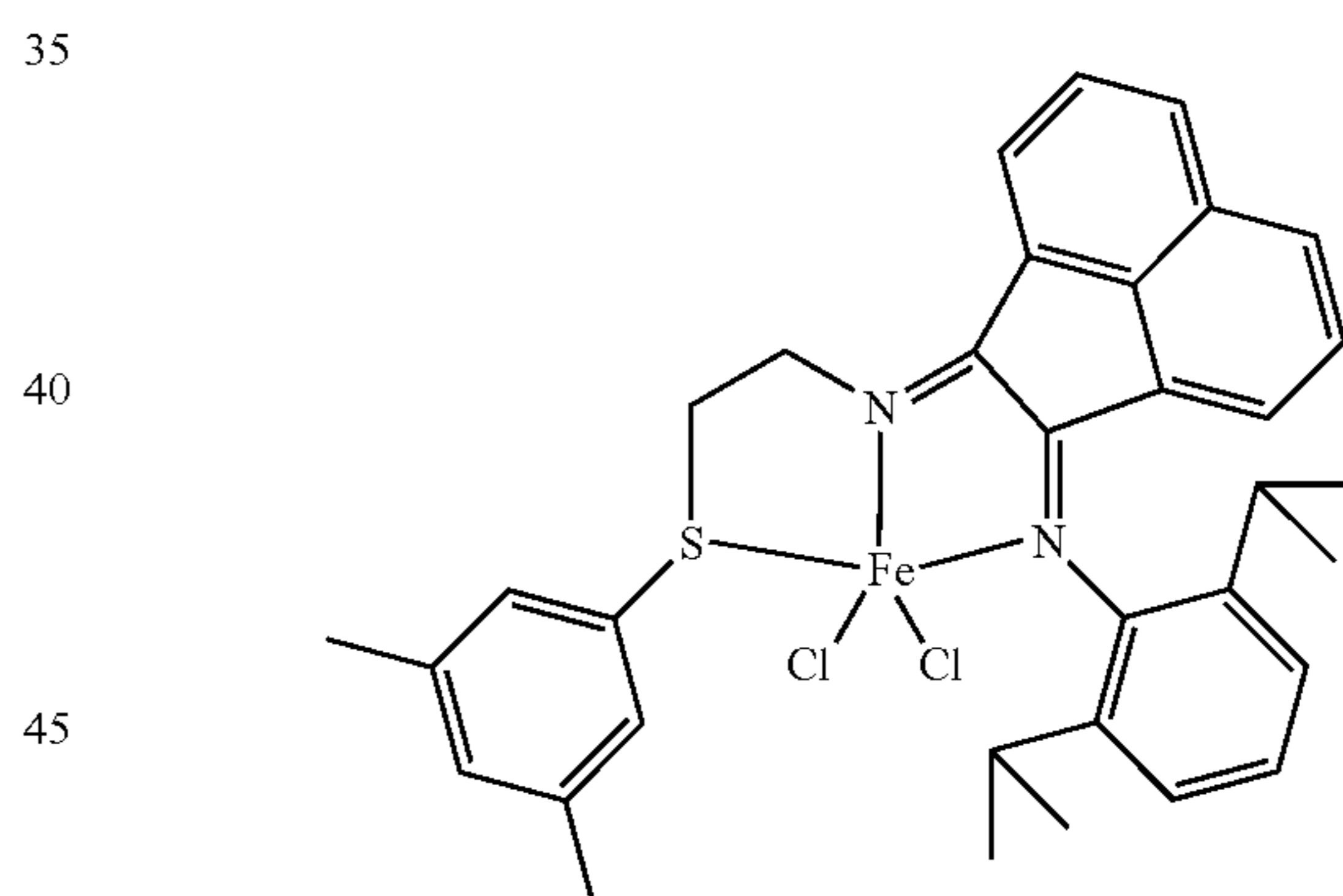
Structure XXV
