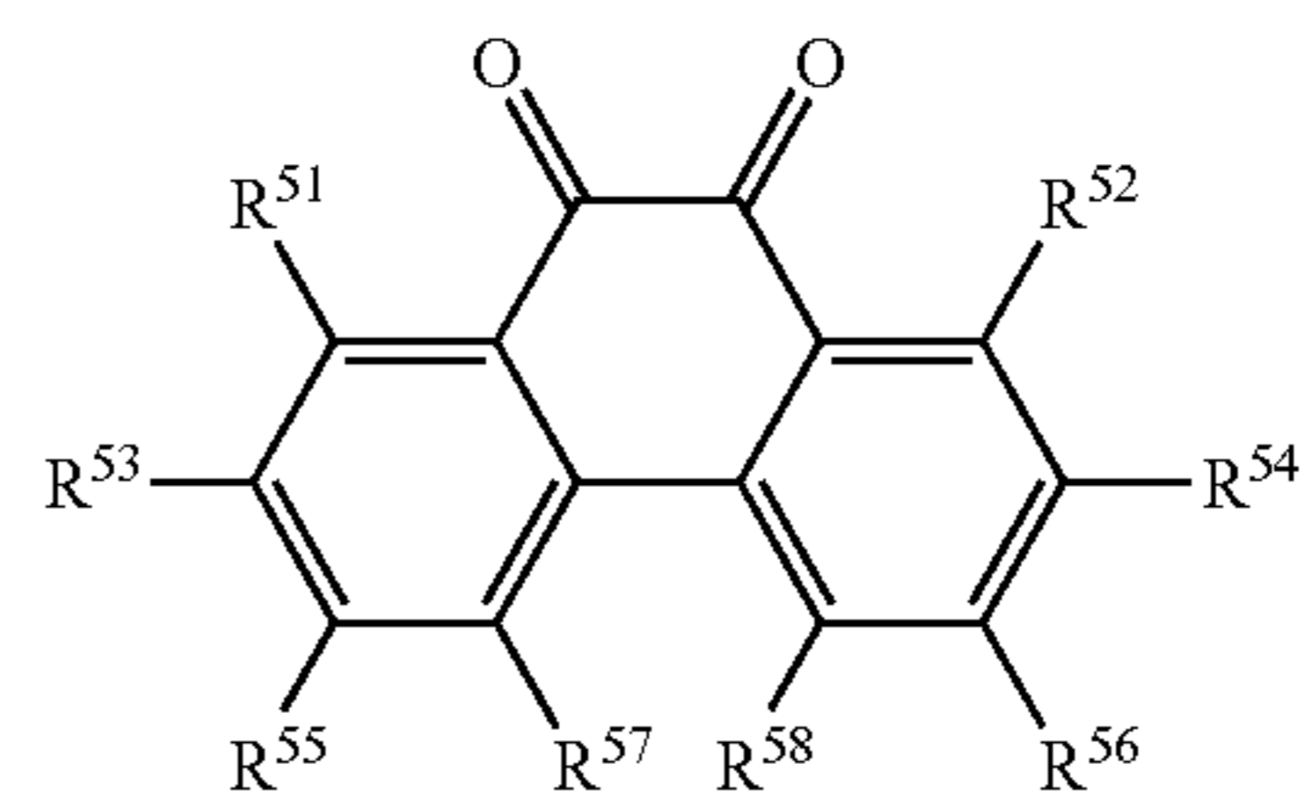
Structure 11
