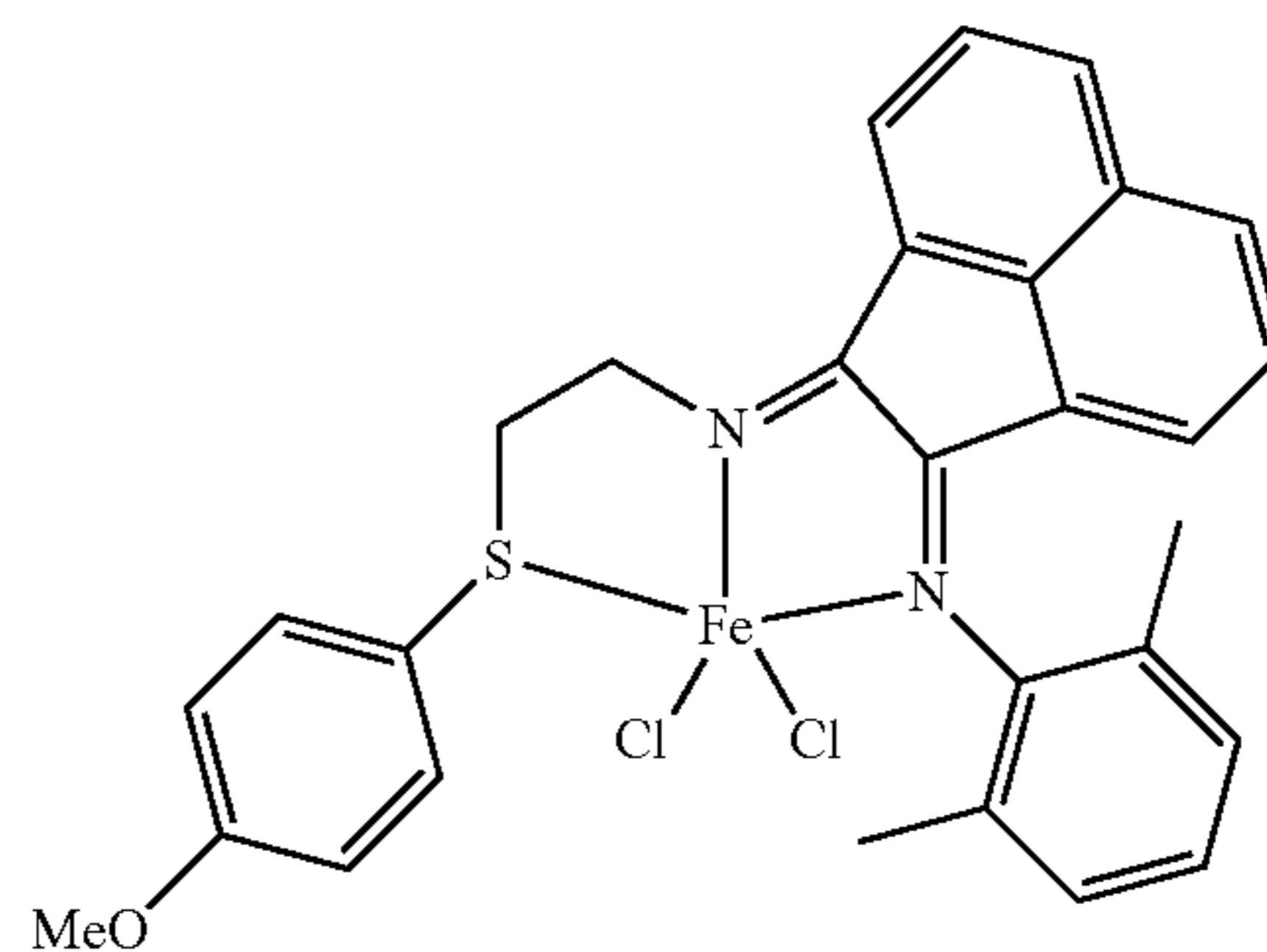
Structure XXXII
