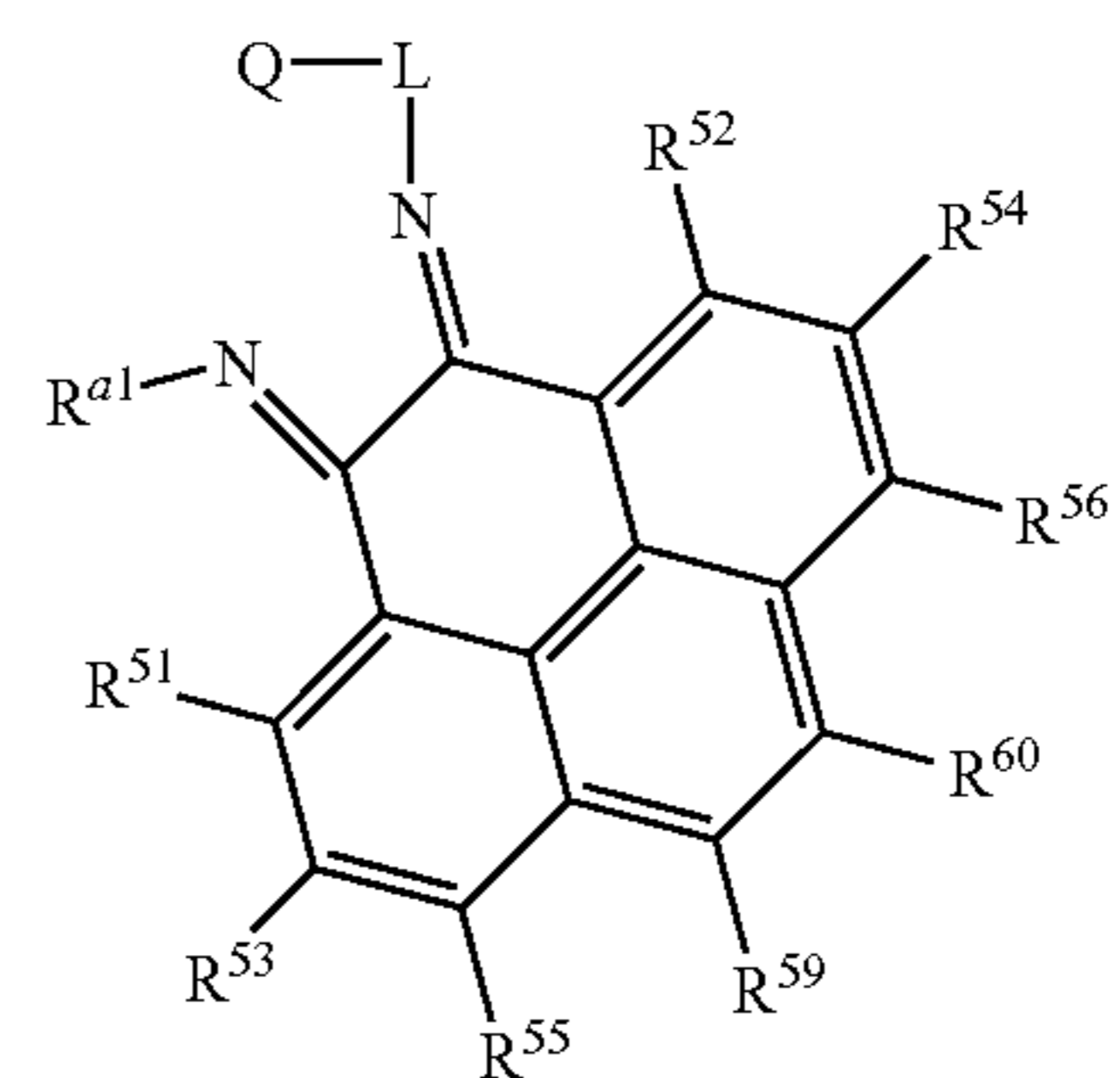
Structure 26f
