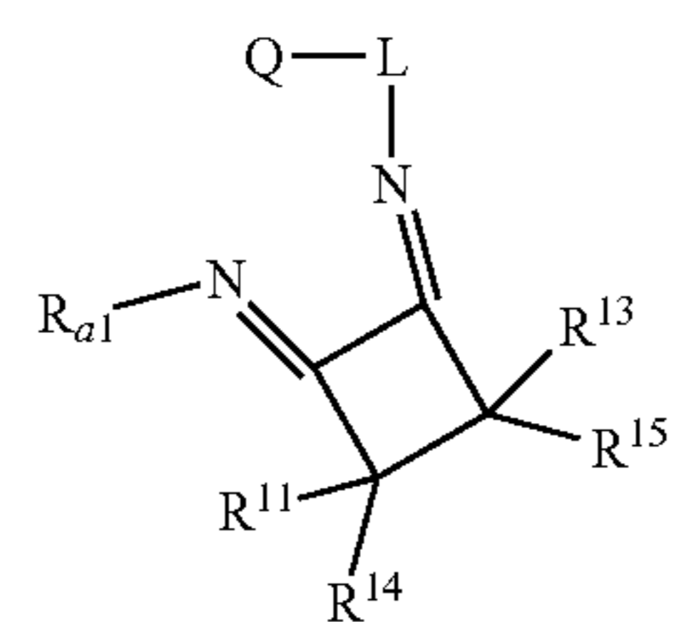
Structure 16f
