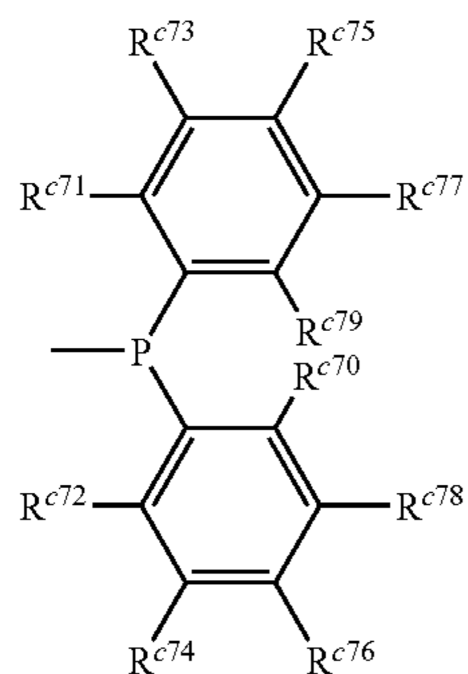
Structure 22c
