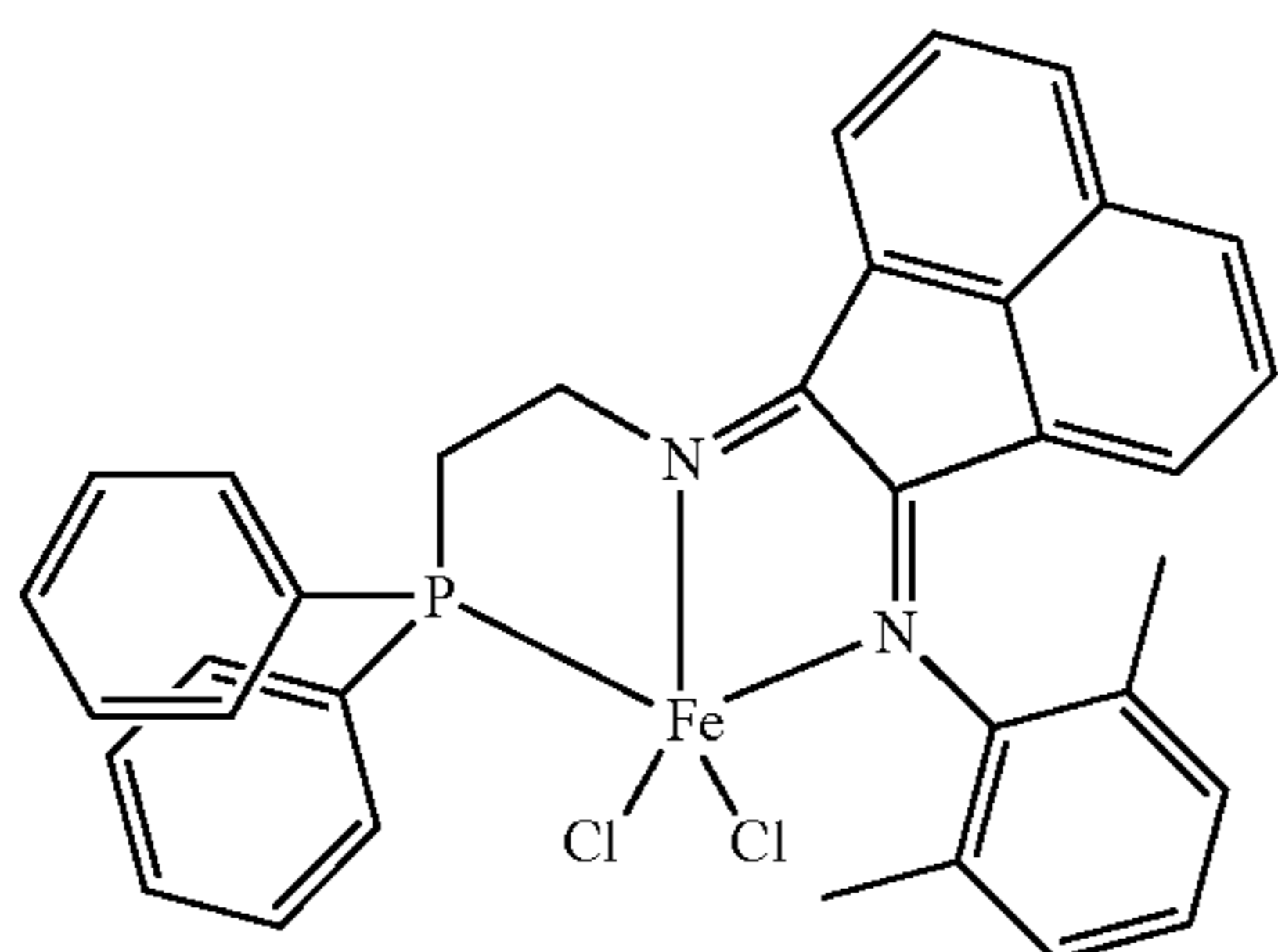
Structure IV
