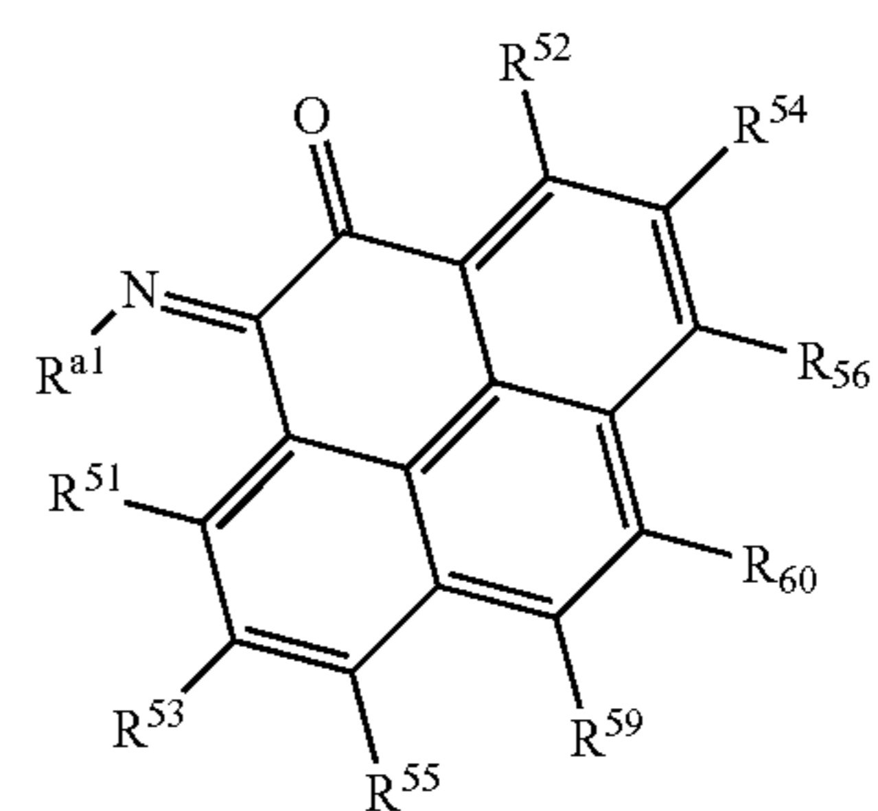
Structure 13b
