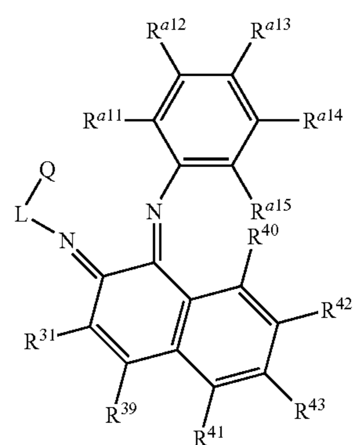
Structure 36f
