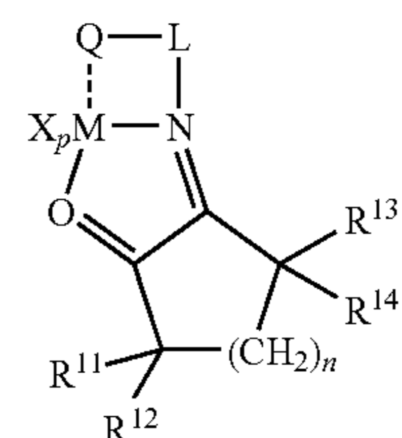
Structure 15d
