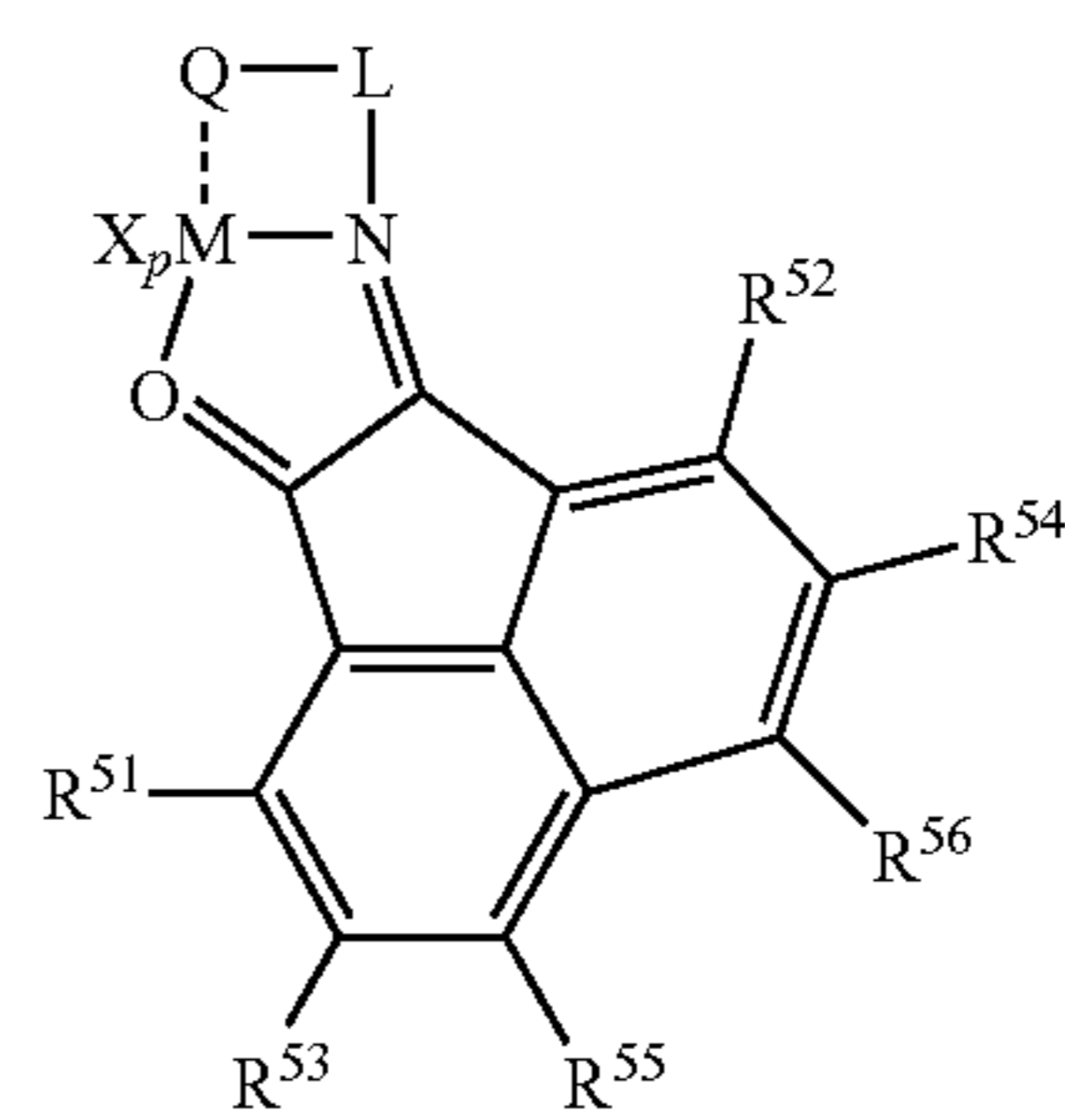
Structure 24d
