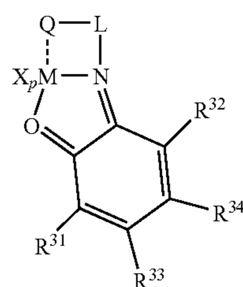
Structure 20d
