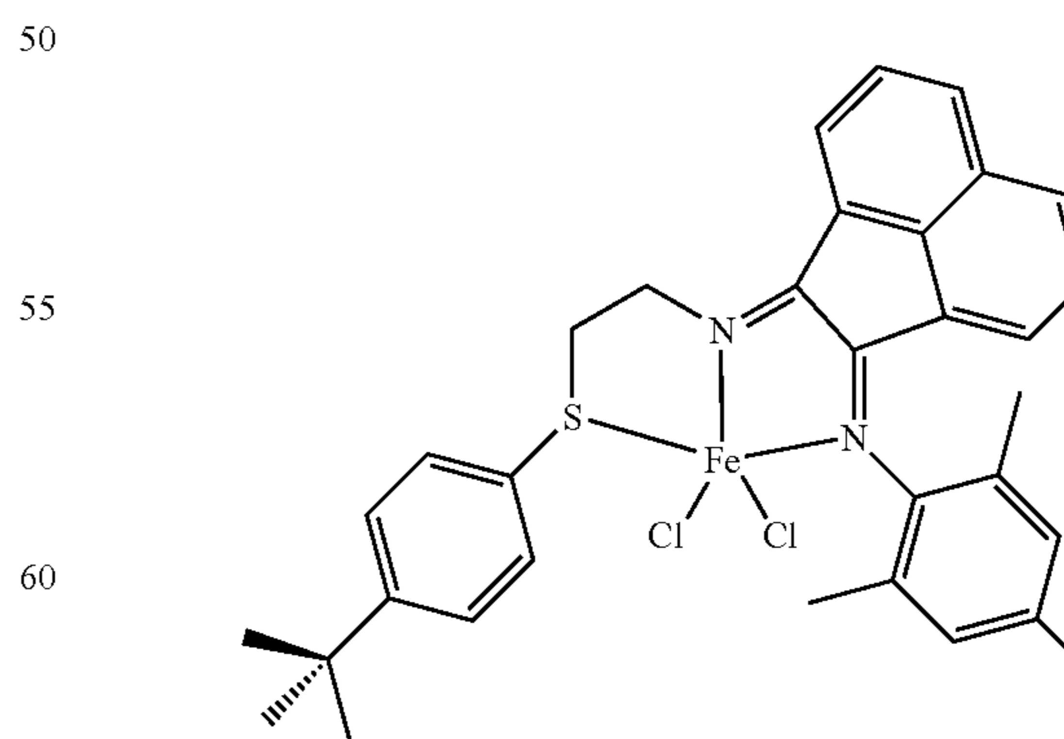
Structure XXV
