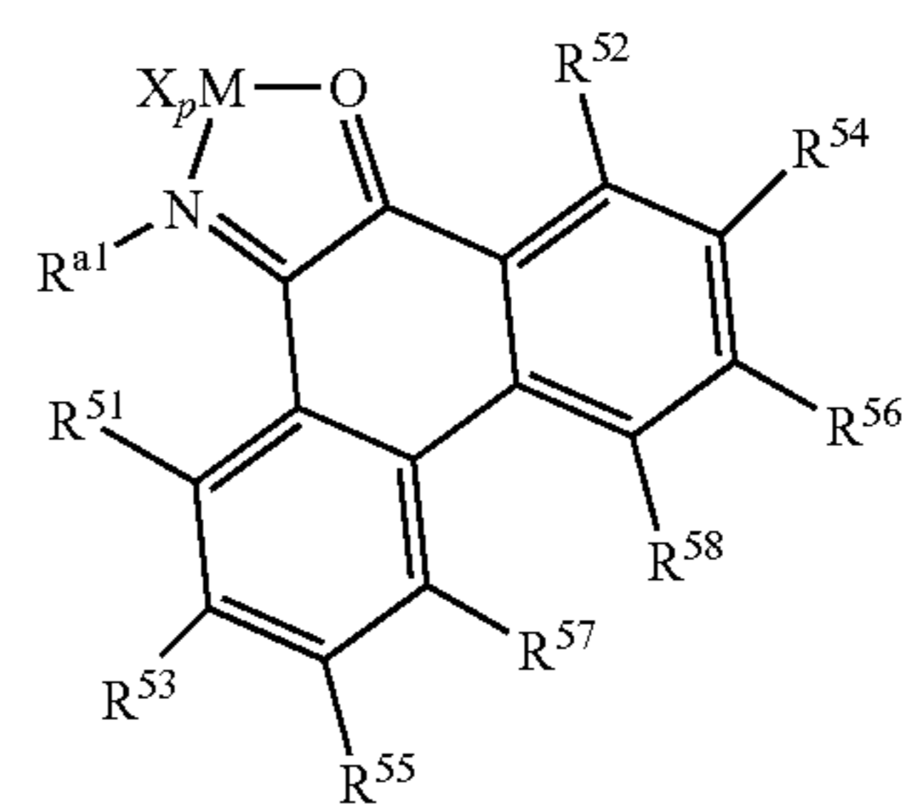
Structure 12d
