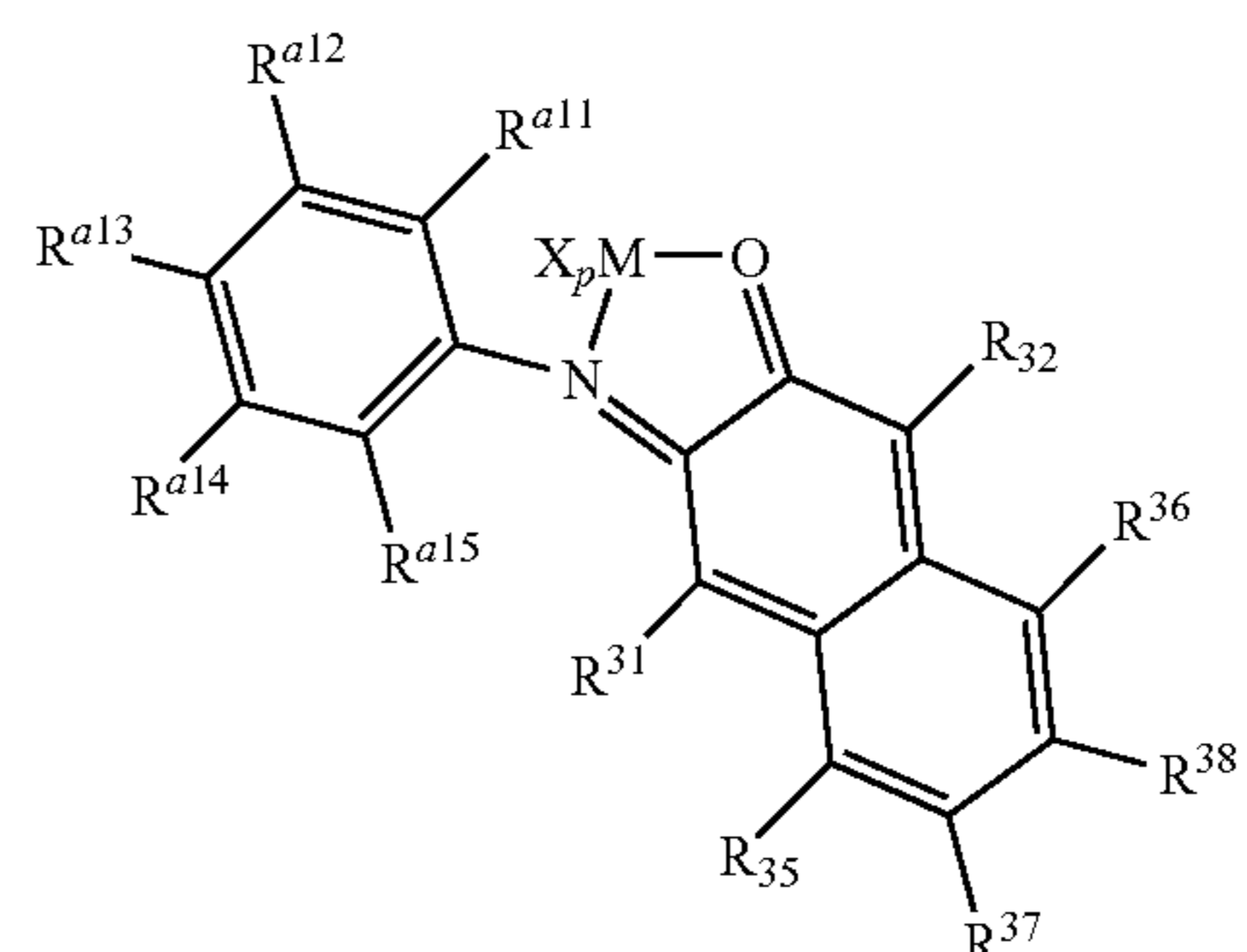
Structure 34d
