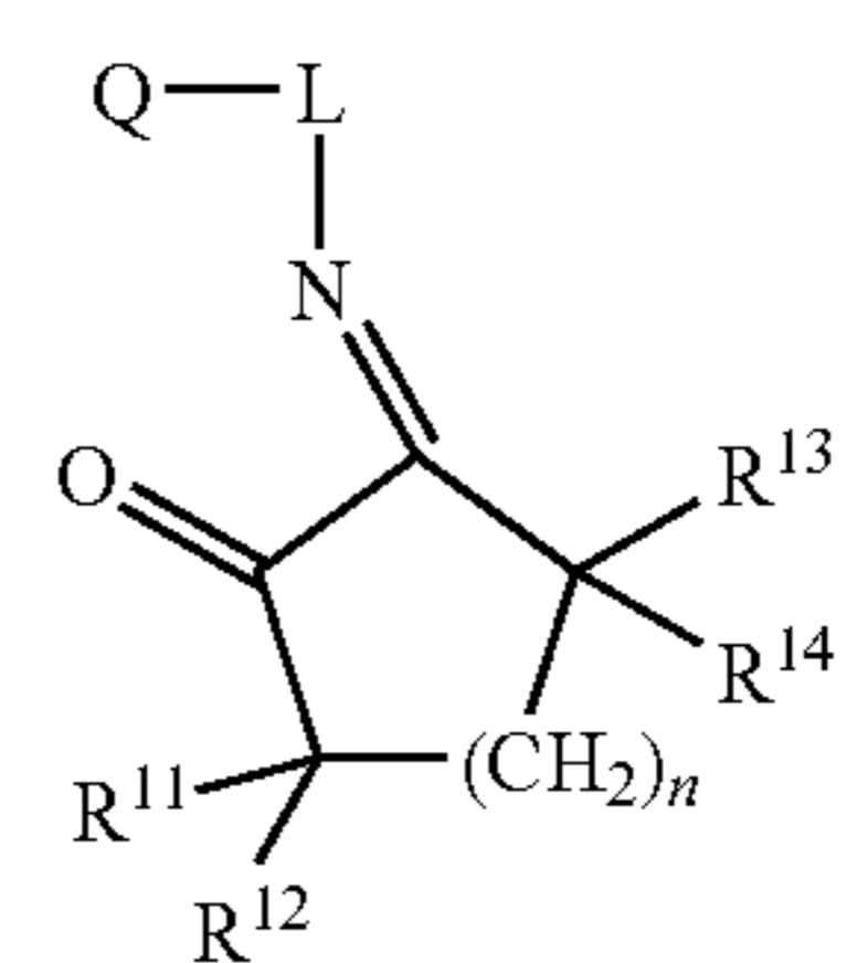
Structure 15b
