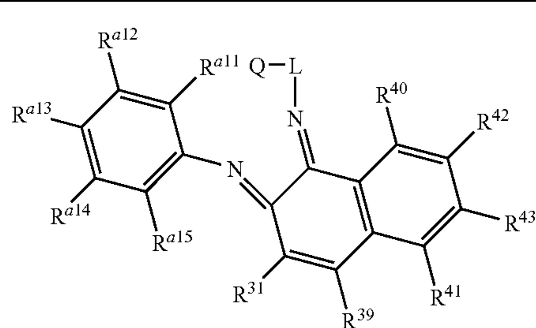
Structure 35f
