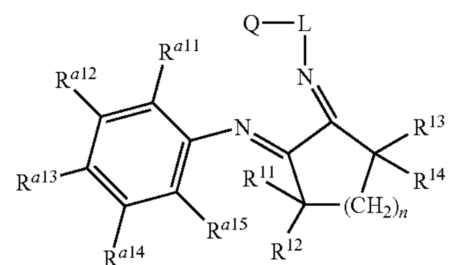
Structure 28f
