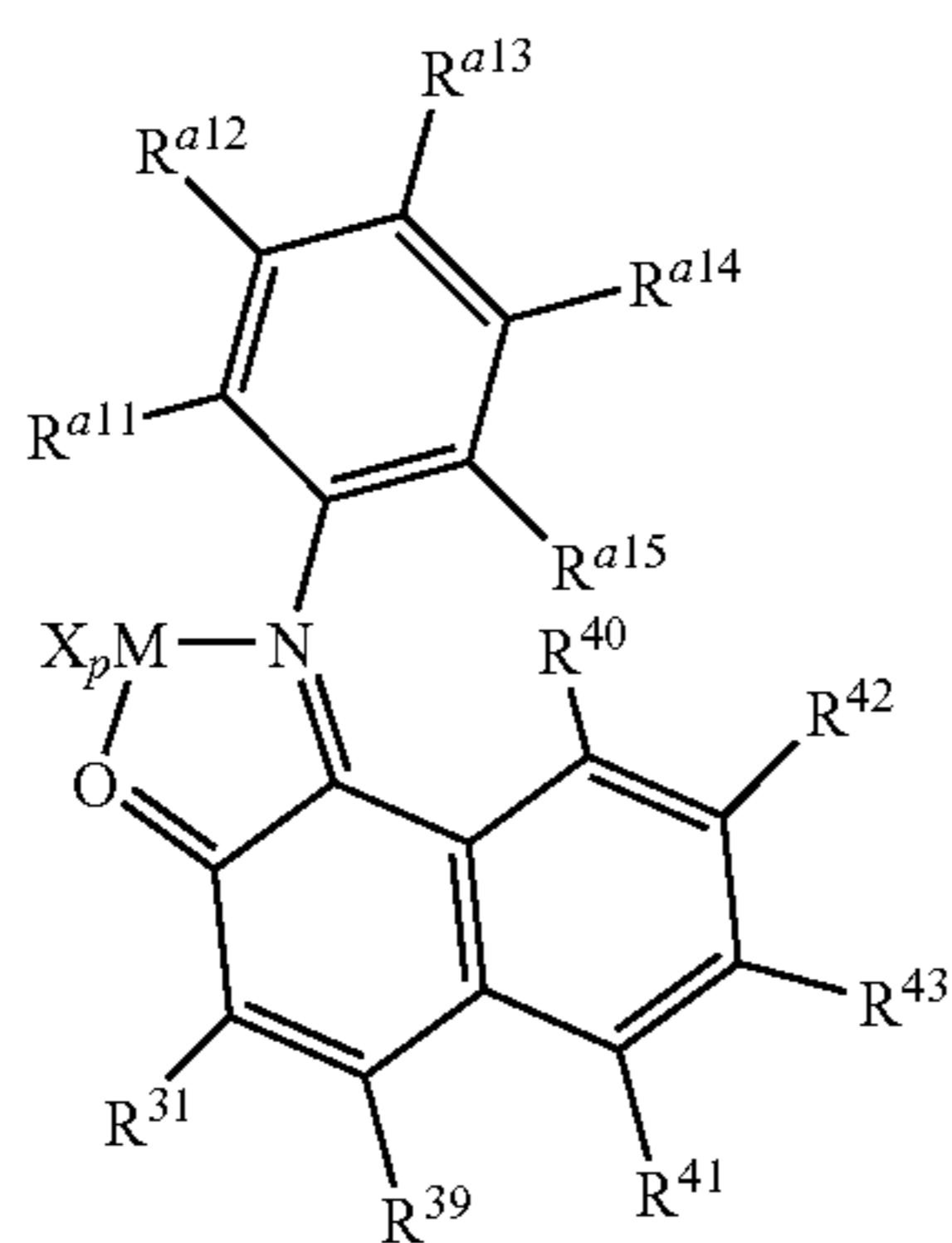
Structure 36d
