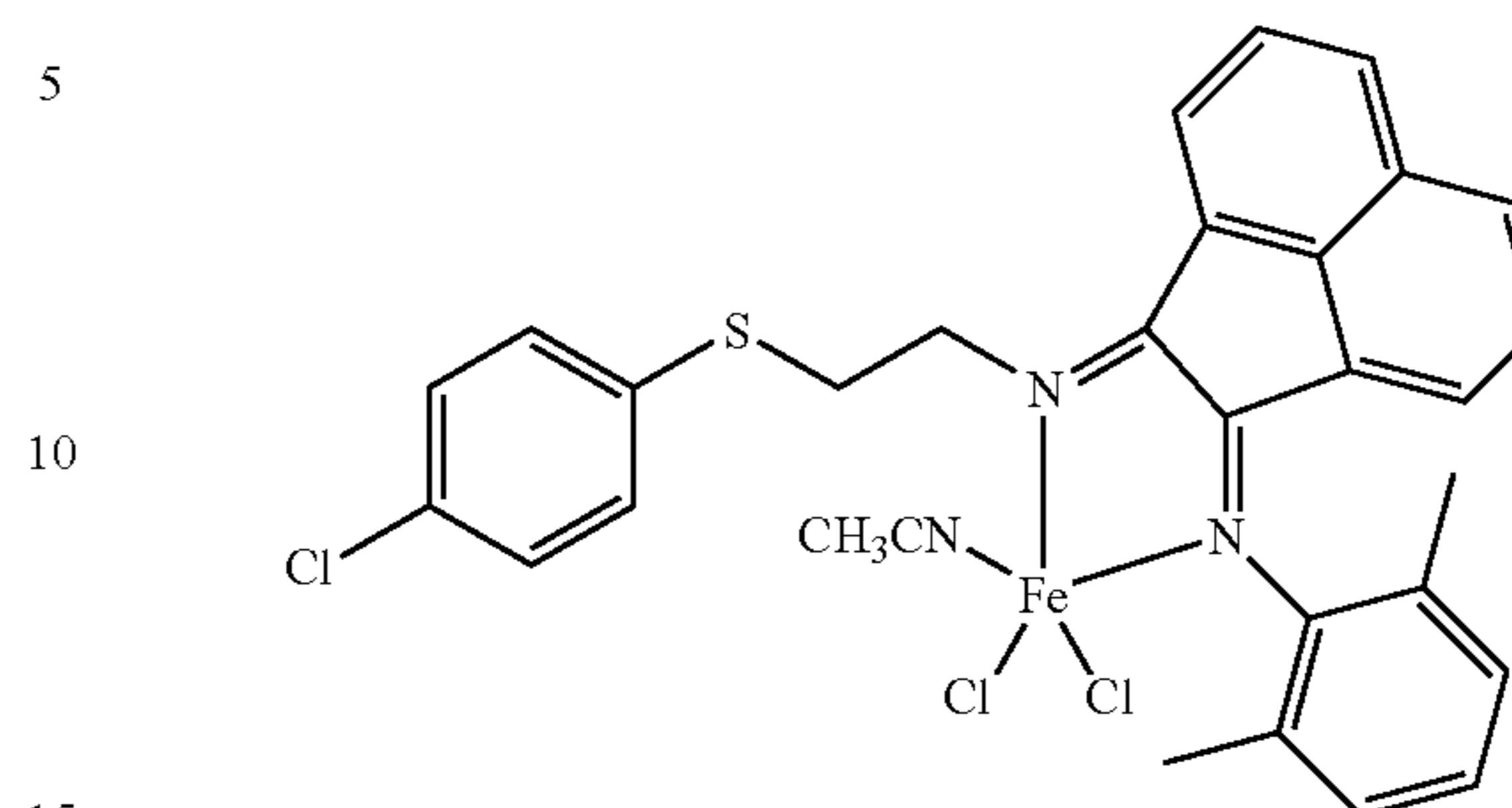
Structure XXIII
