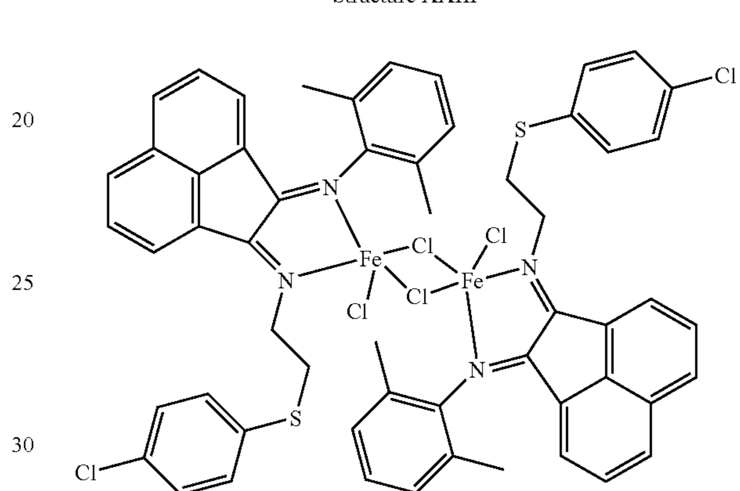
Structure XXIII
