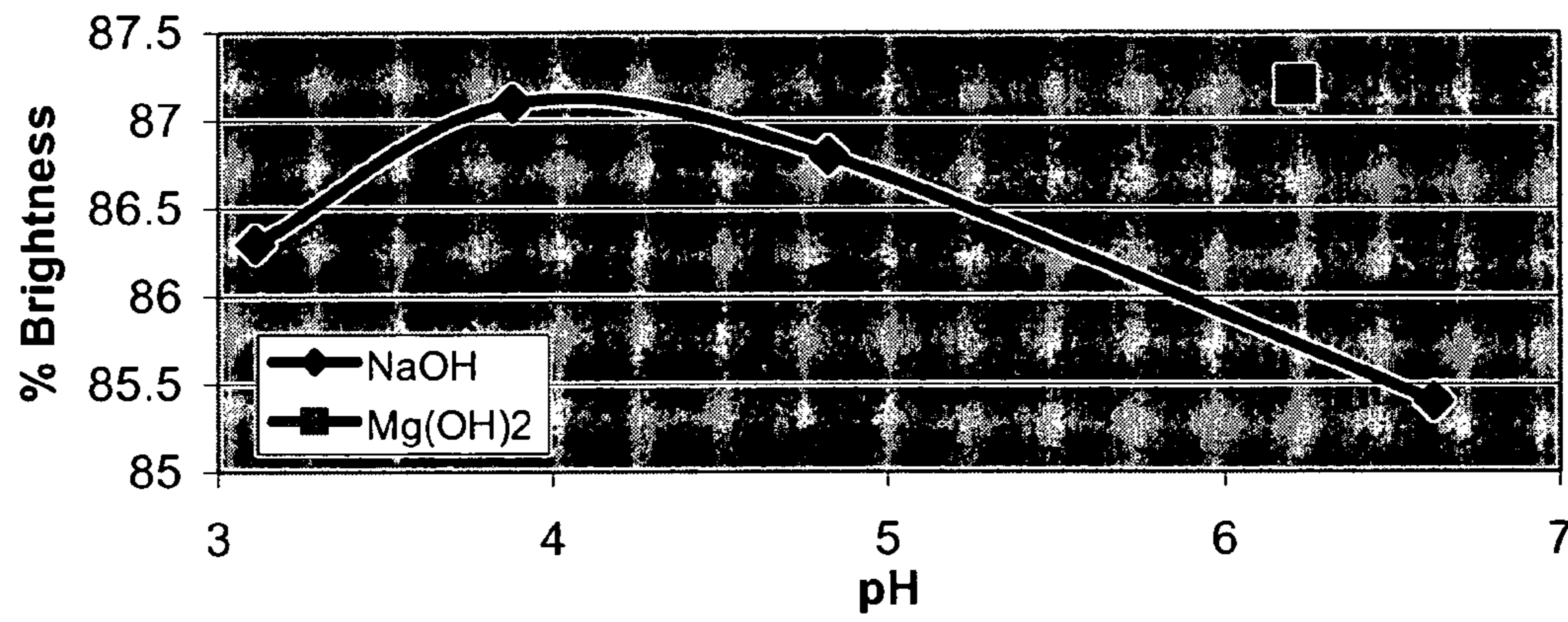
Fig. 2- Effect of D1 pH and Caustic Source on D1 Brightness - Softwood Pulp
