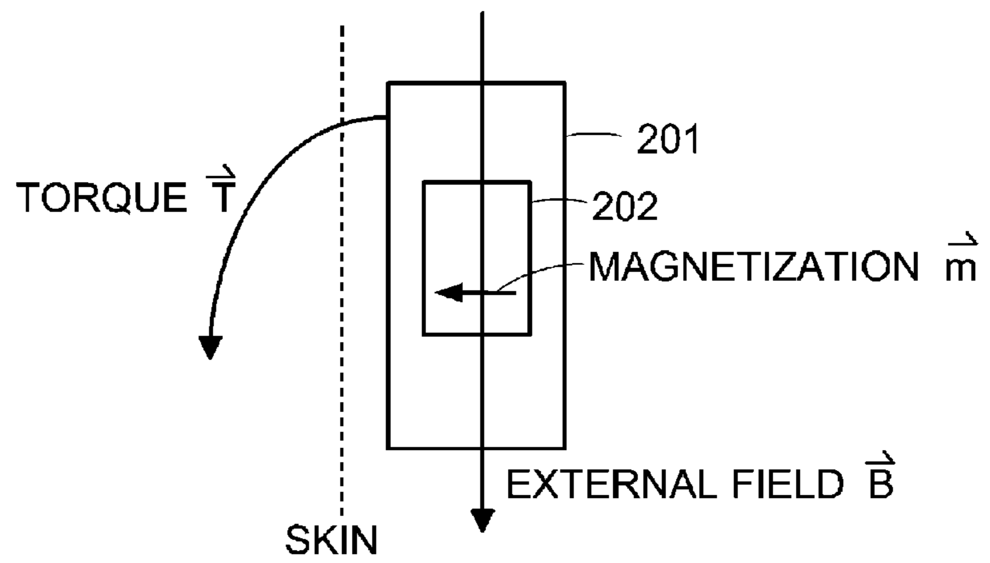
FIG. 2 PRIOR ART
