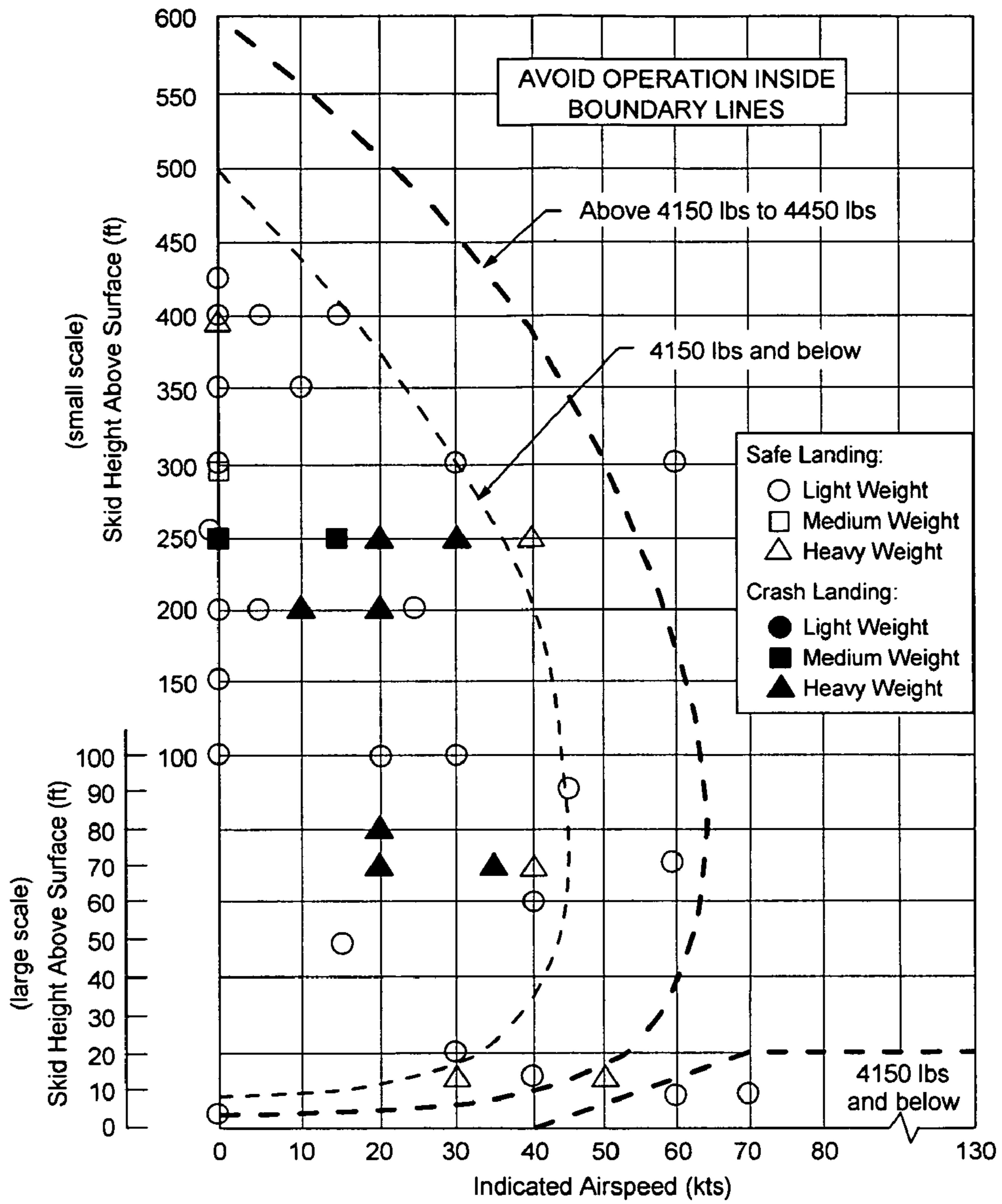
Figure 5. Automated autorotation flight conditions evaluated
