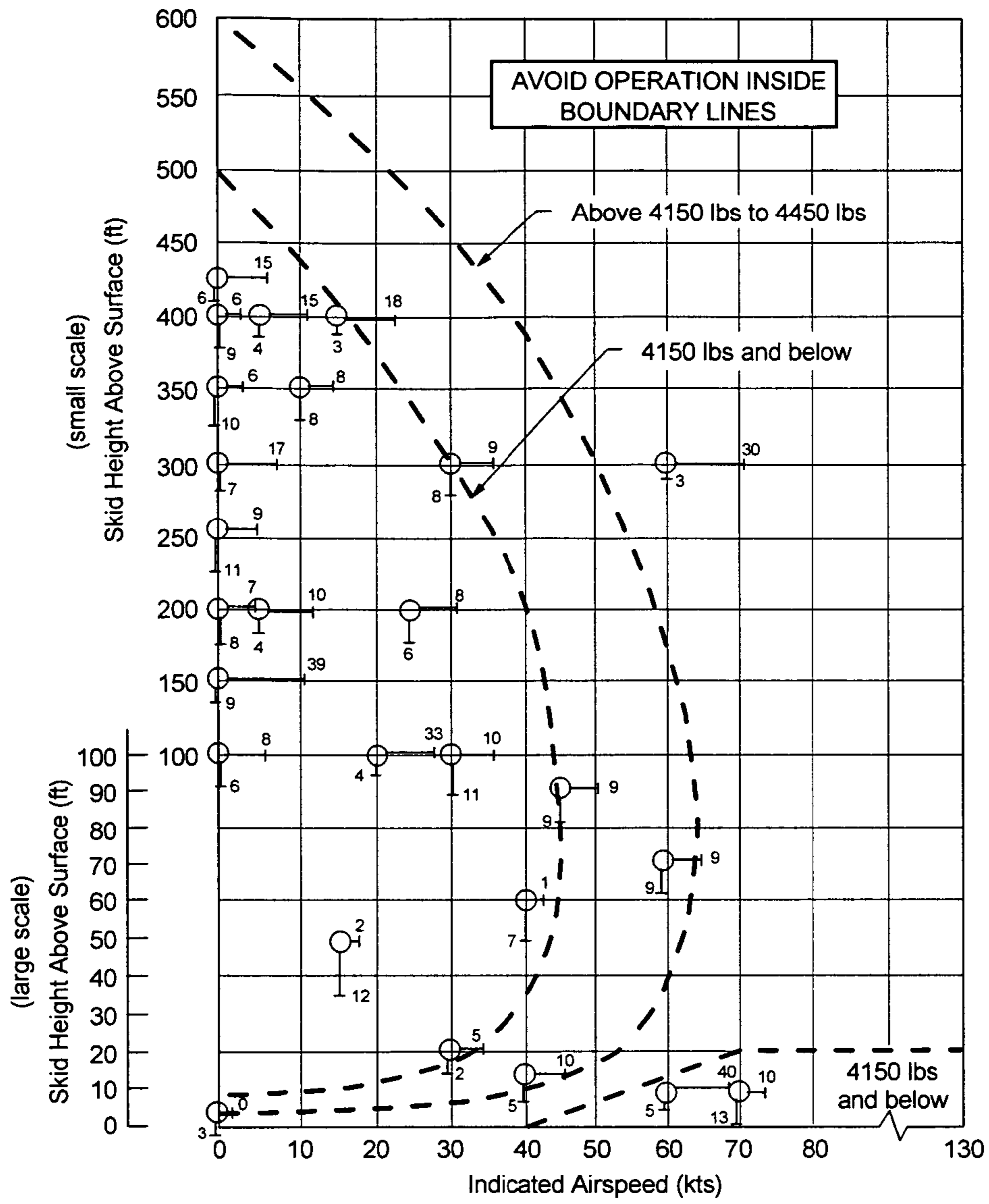
Figure 6 Touchdown ground-speed and sink-rate (light weight condition)
