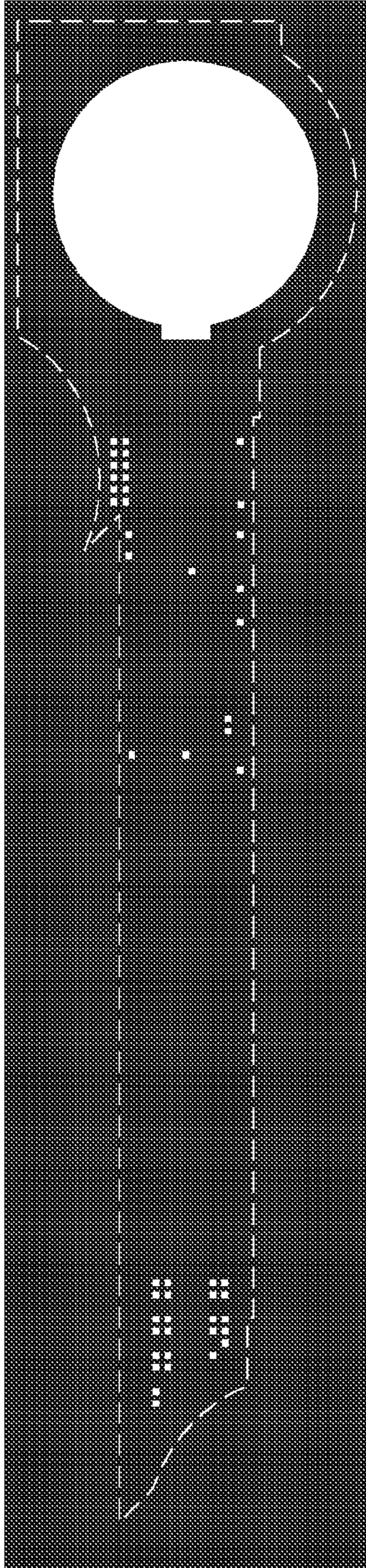
Via 1 mask
