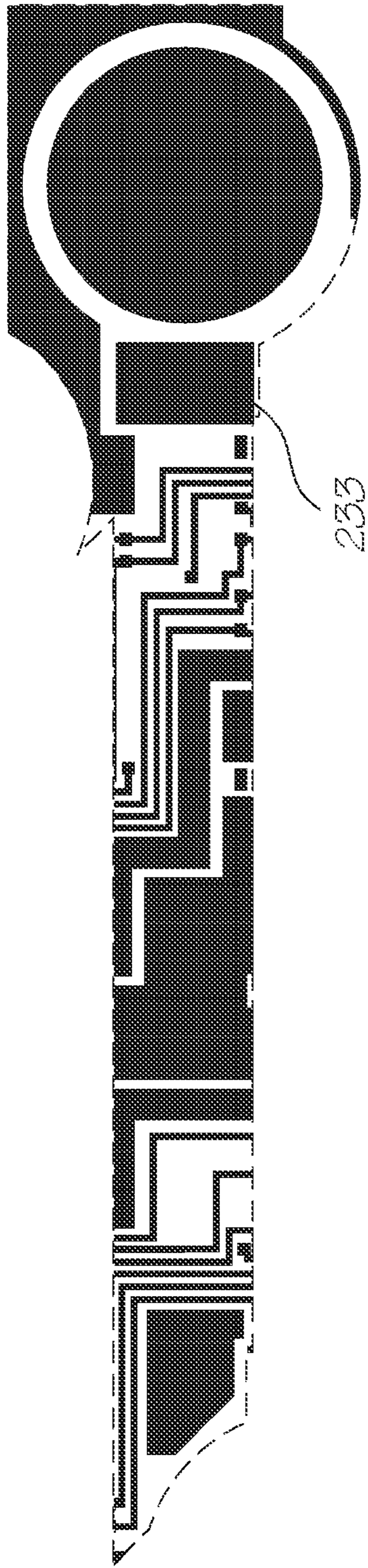
Metal 2 mask
