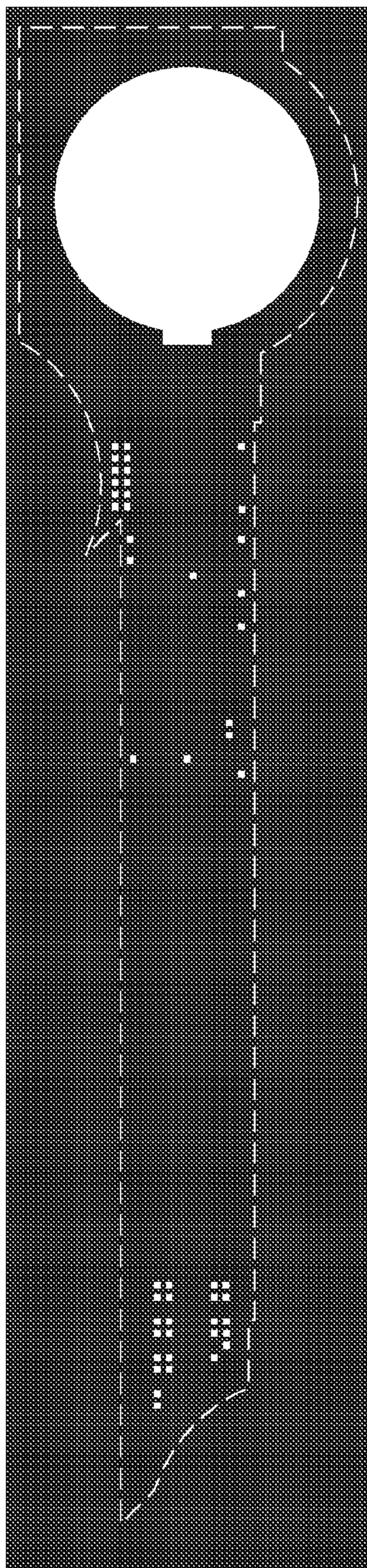
Via 1 mask
