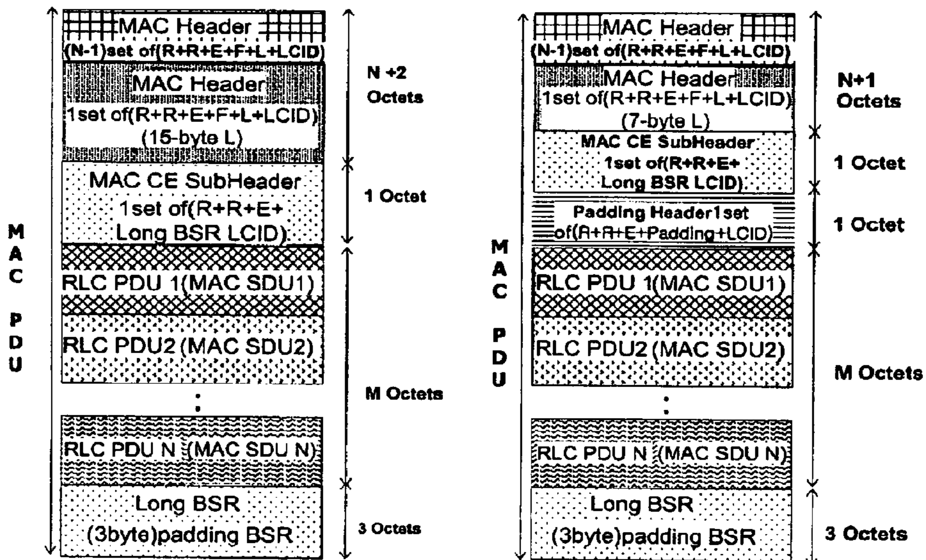
(b) case 2, 15-bit L field for the last MAC SDU
