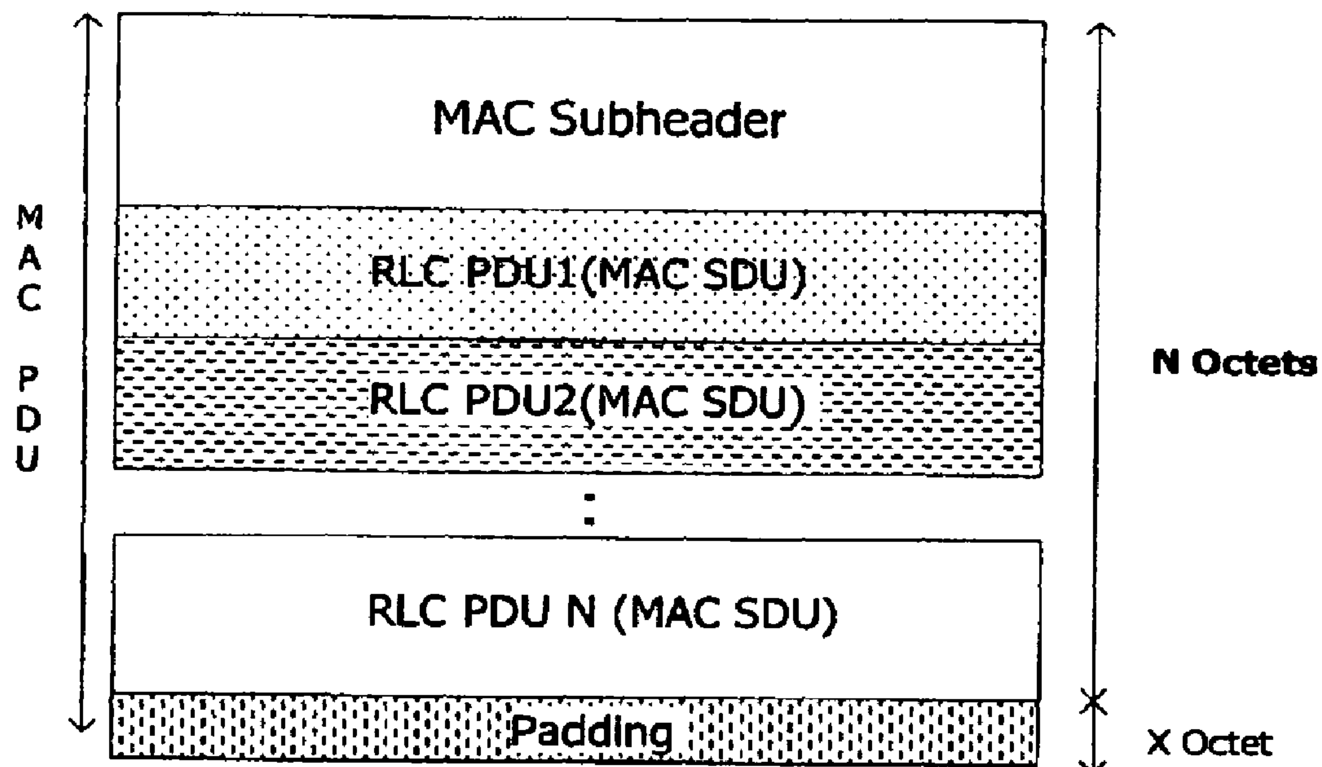
(a) MAC PDU with data and padding
