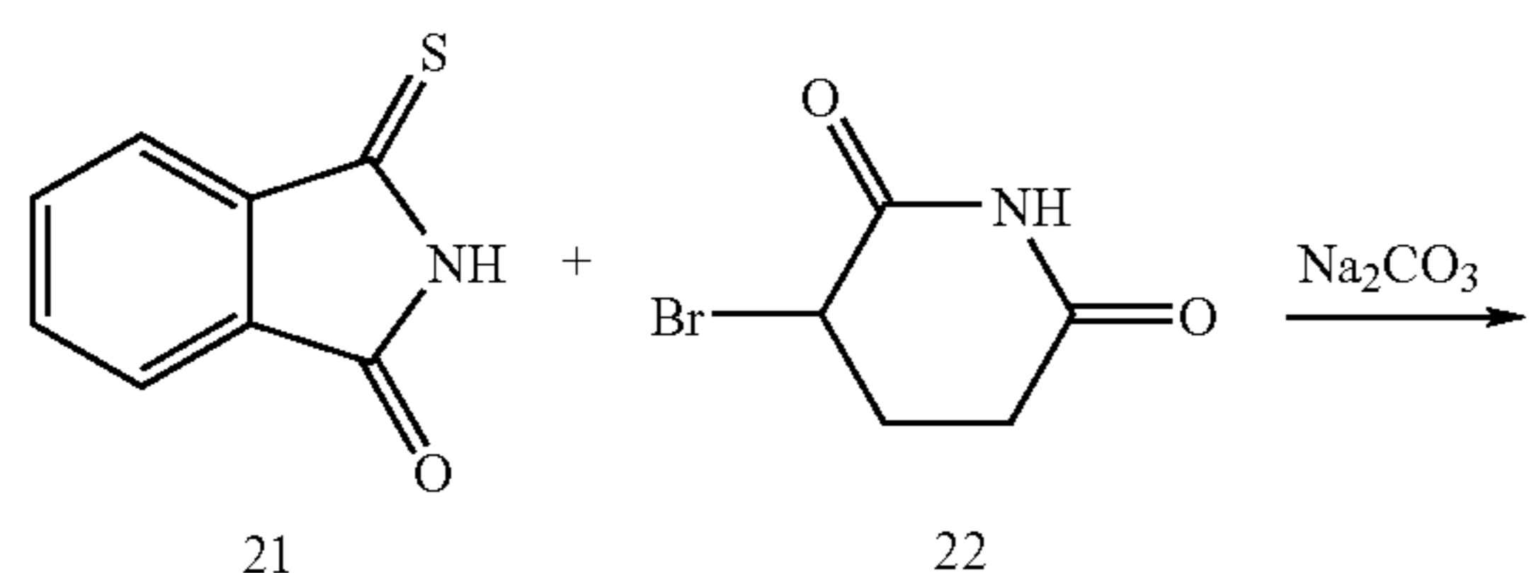
Scheme 9
