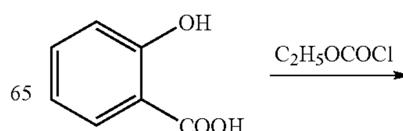
Scheme 8
