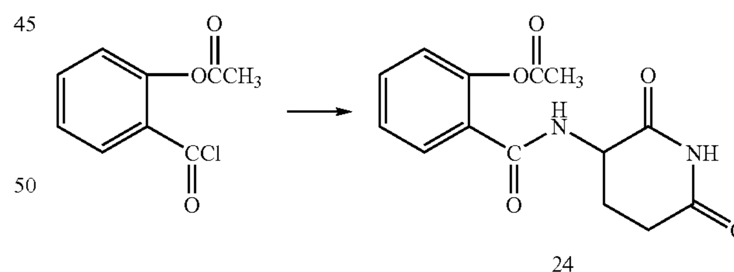
Scheme 10
