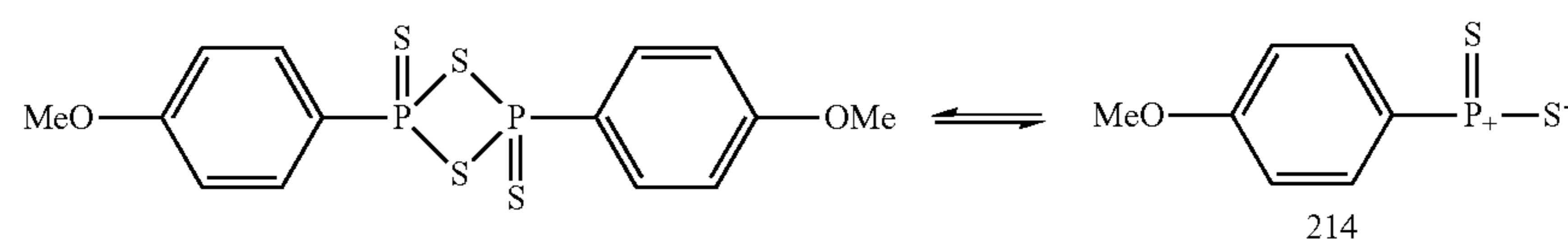
Scheme 14. The mechanism of catalysis for Lawesson's reagent.
