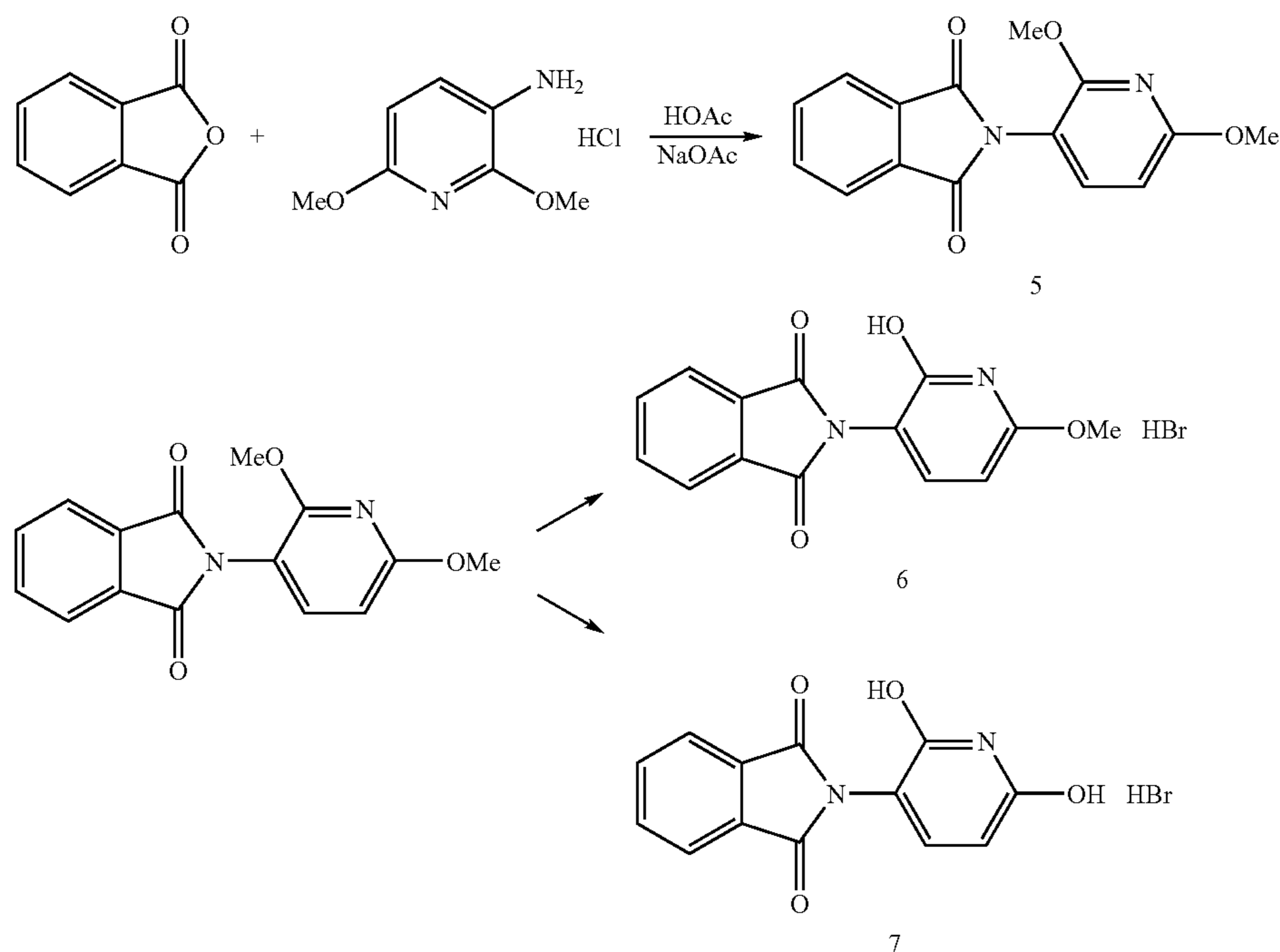
Scheme 2
